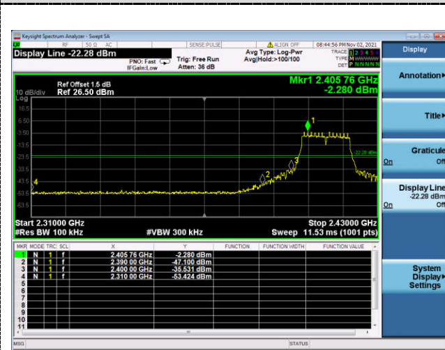
Left bandedge
