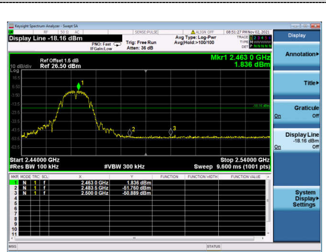
Right bandedge
