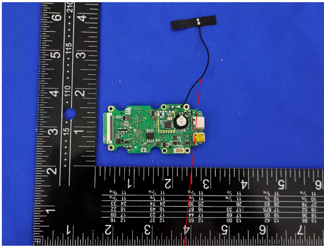
FPC antenna
