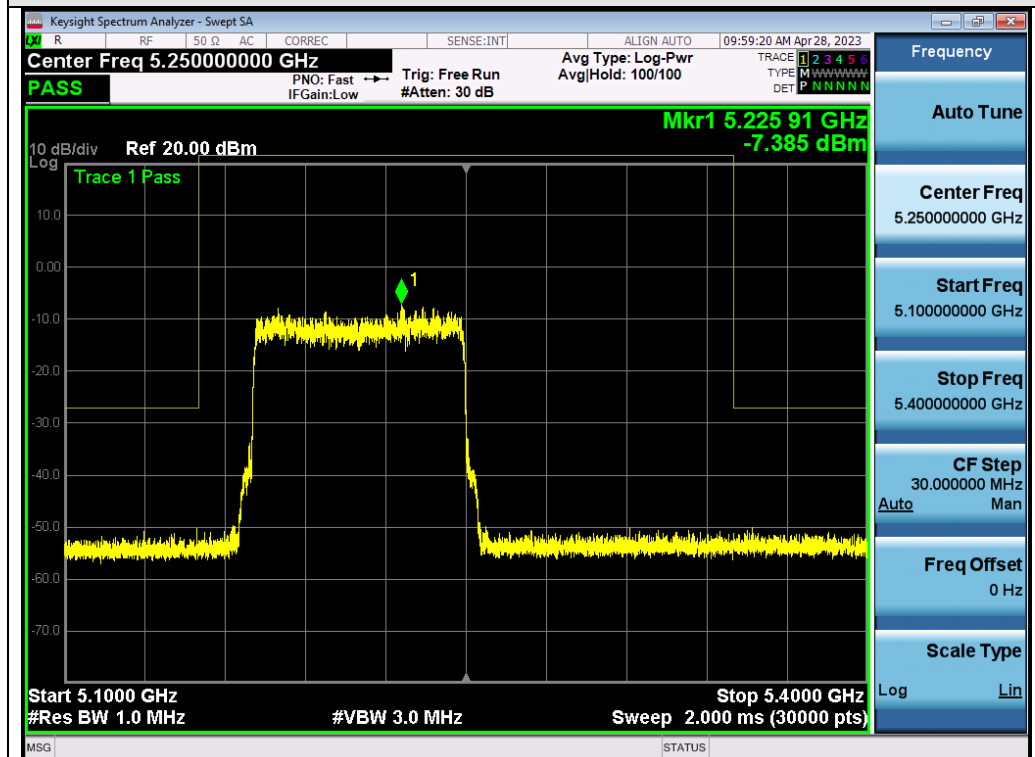
Test_Graph_802.11ax80_ANT2_5210_MCS9_Frequency Band 3
