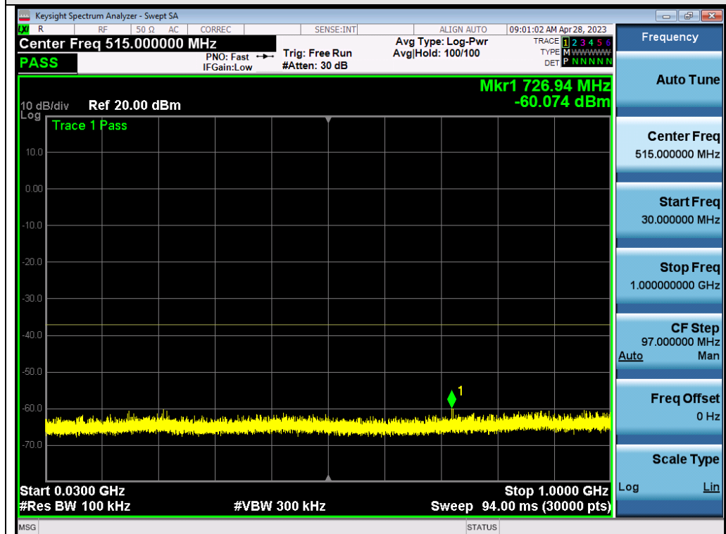
Test_Graph_802.11ax80_ANT1_5210_MCS9_Frequency Band 1
