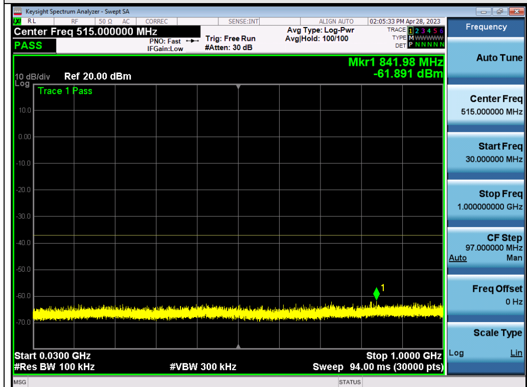
Test_Graph_802.11ax80_ANT1_5775_MCS9_Frequency Band1
