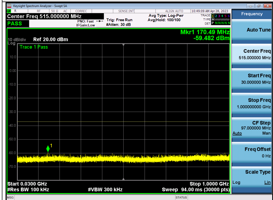
Test_Graph_802.11n40_ANT1_5795_MCS0_Frequency Band1
