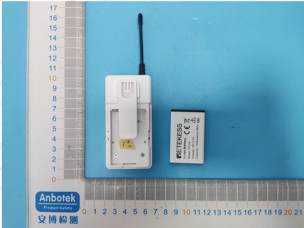
Transmitter ANT
