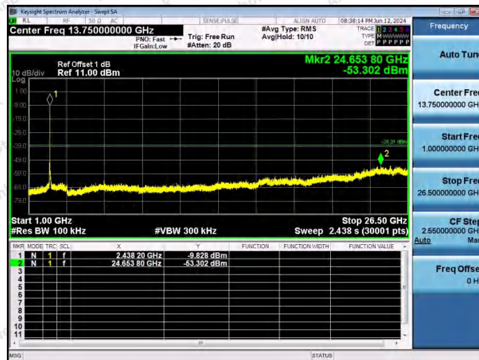
11G-Ant1-2437-1000~26500-PASS
