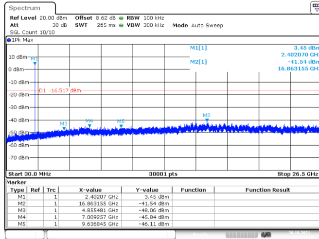
Tx. Spurious NVNT 1-DH1 2402MHz Ant1 Emission
