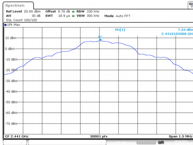
Tx. Spurious NVNT 1-DH1 2441MHz Ant1 Ref
