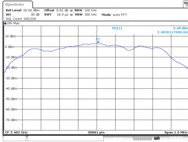
Tx. Spurious NVNT 1-DH1 2402MHz Ant1 Ref
