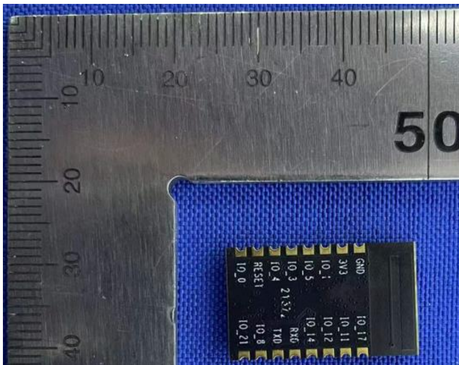
PCB Antenna
