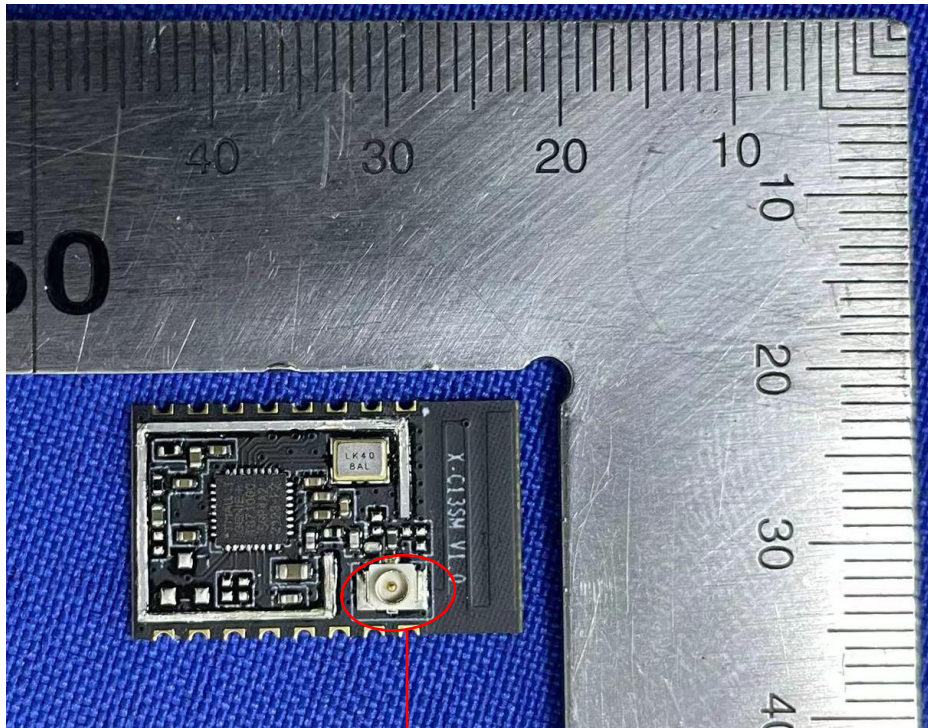
Antenna interface position
