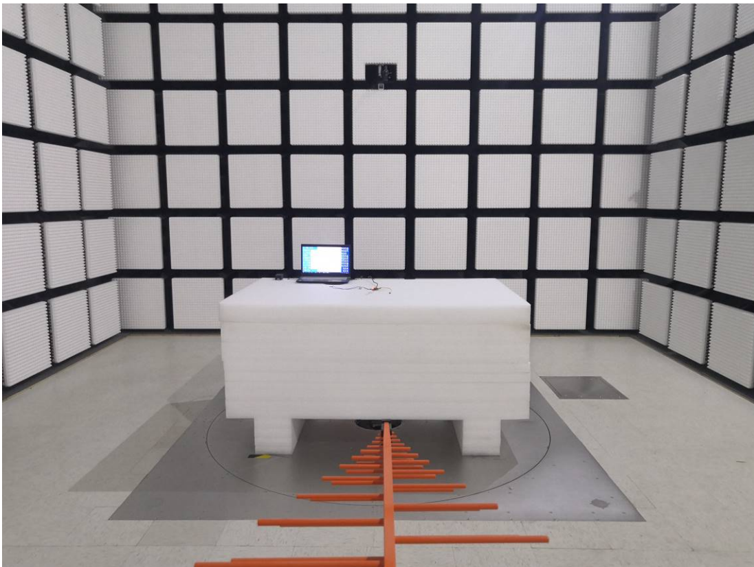
Radiated Emission Below 1GHz View X-C13SL-0
