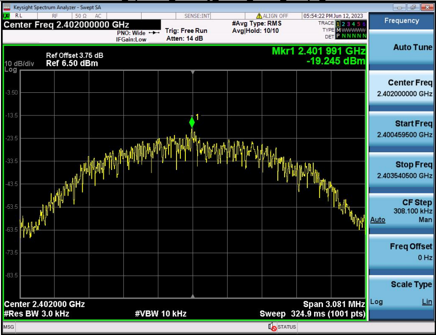
Power Spectral Density NVNT ANT1 2Mbps 2402
