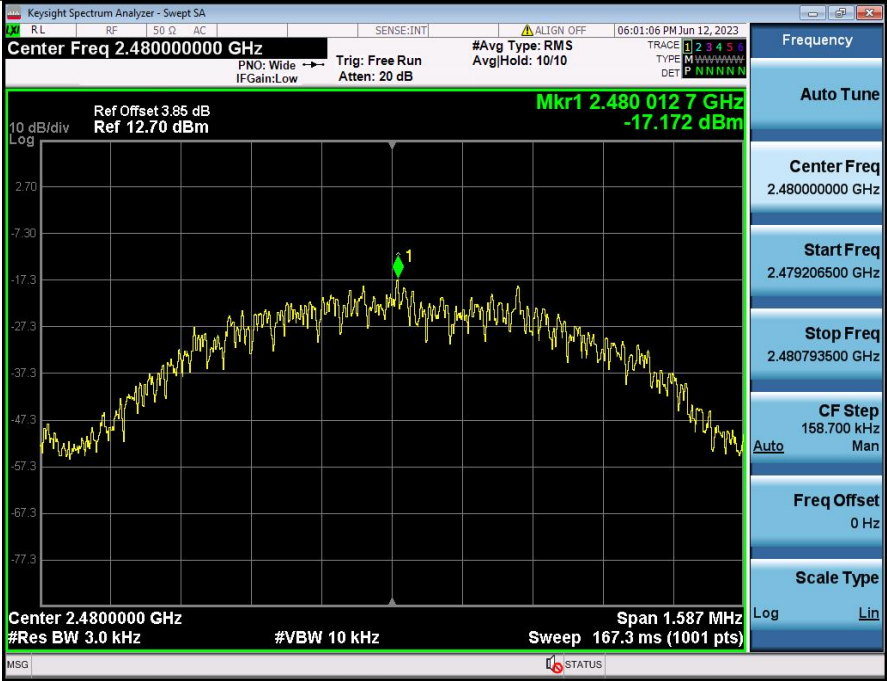
Power Spectral Density NVNT ANT1 1Mbps 2480
