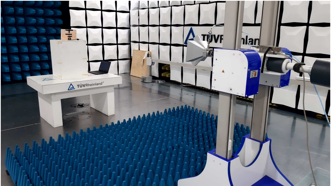
Radiated emission 1GHz-10GHz
