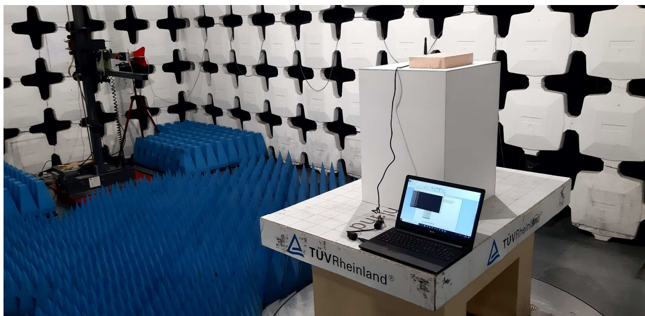
Radiated emission 1GHz-10GHz
