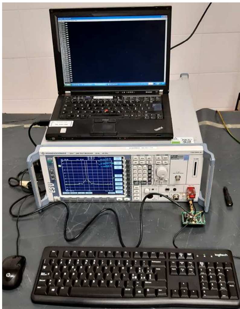
Conducted emission tests
