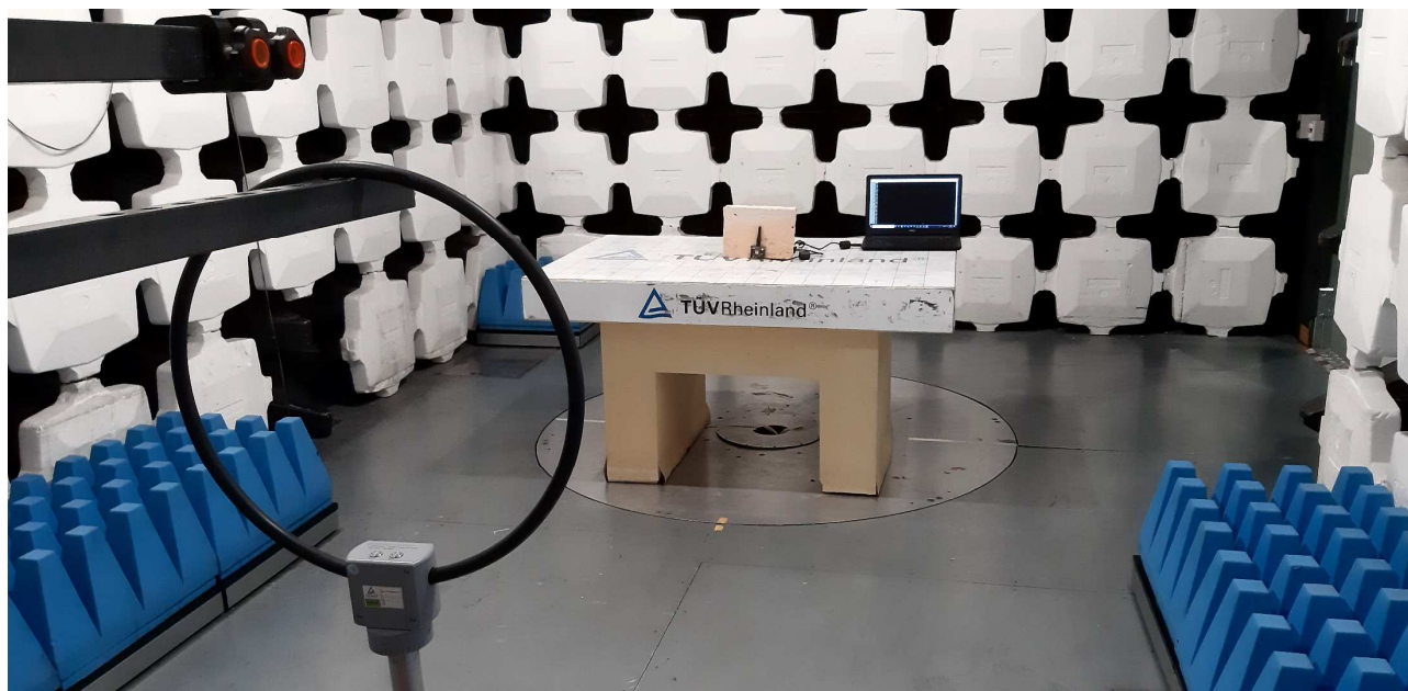
Radiated emission 9kHz-30MHz
