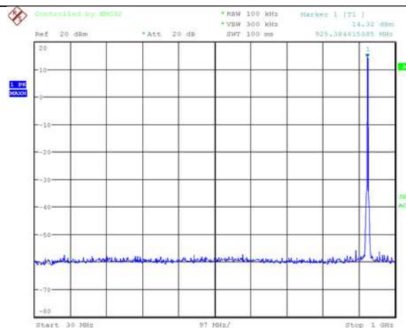
30MHz-1GHz
