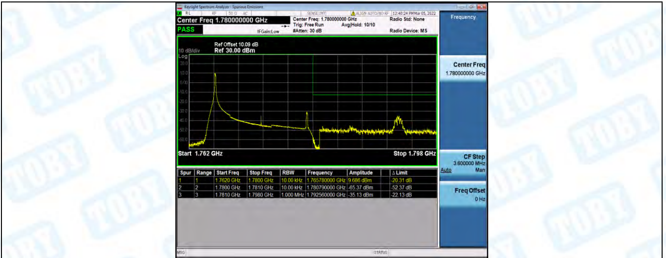
Band66-15MHz-QPSK-132597-1RB#74
