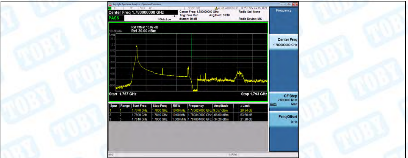
Band66-10MHz-16QAM-132622-1RB#49
