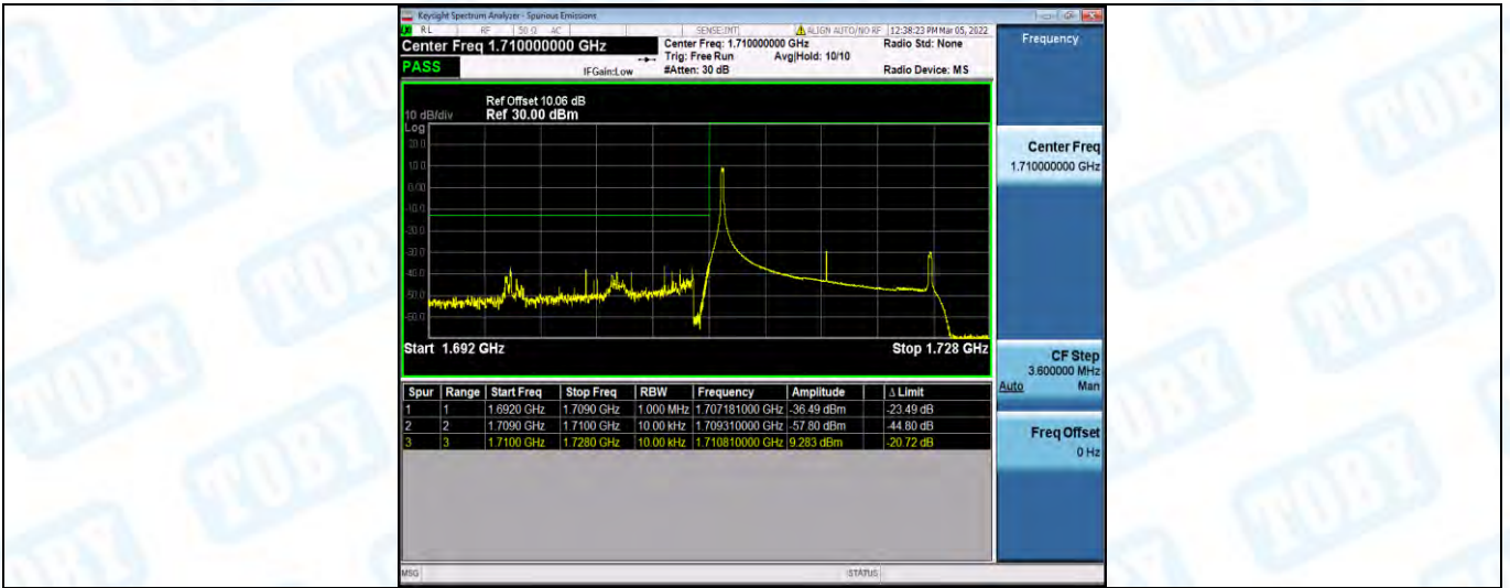
Band66-15MHz-16QAM-132047-1RB#74
