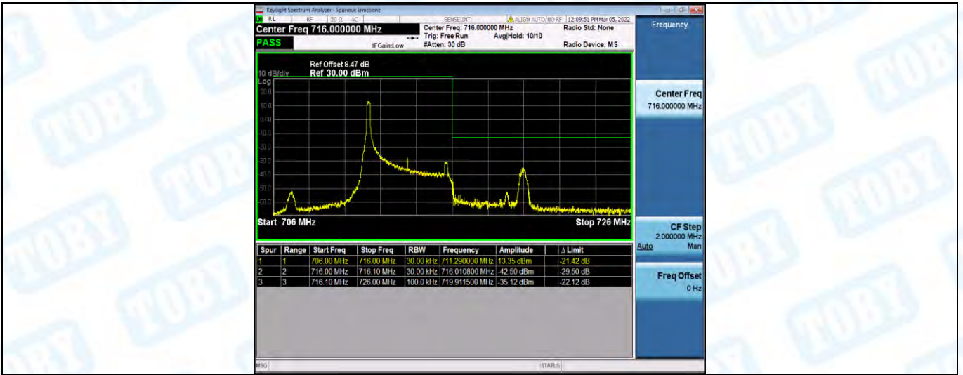
Band17-5MHz-QPSK-23825-1RB#24
