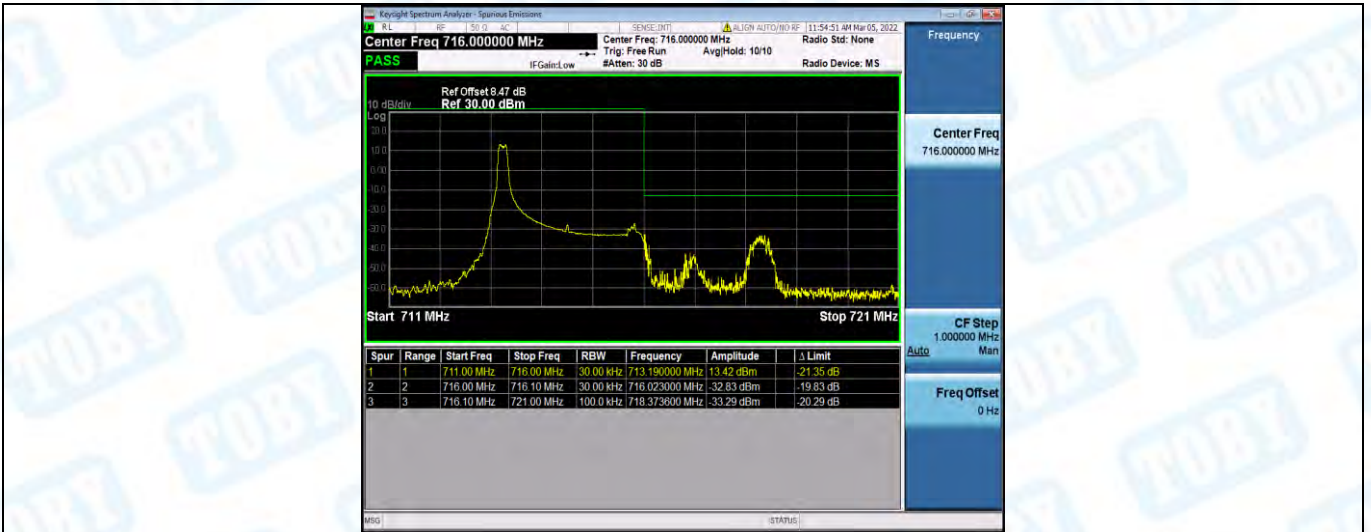
Band12-3MHz-16QAM-23165-1RB#14
