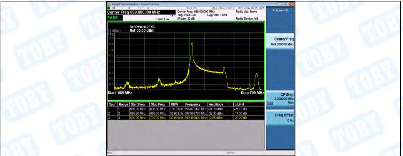
Band12-5MHz-16QAM-23035-1RB#24
