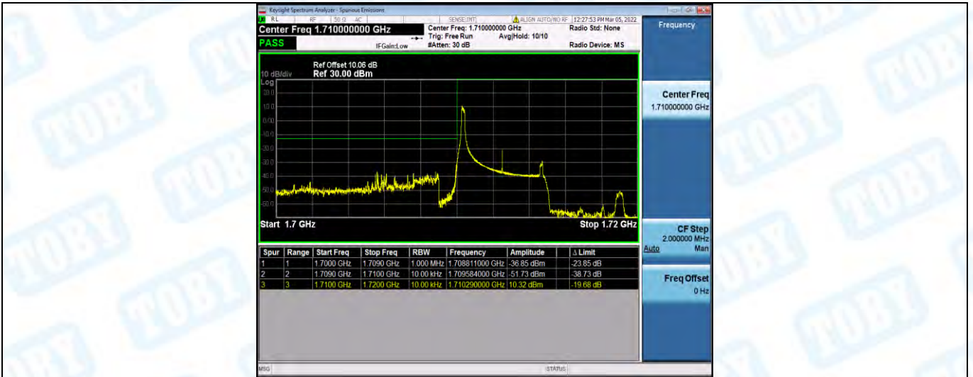
Band66-5MHz-16QAM-131997-1RB#24
