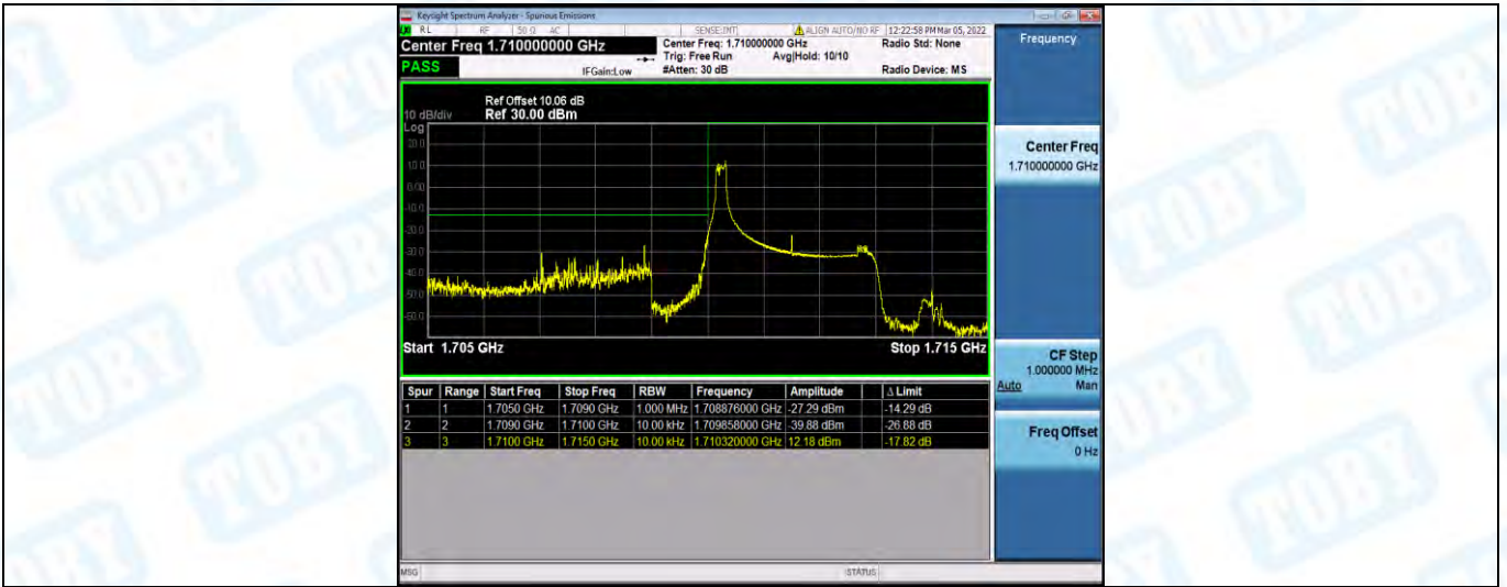
Band66-3MHz-16QAM-131987-1RB#14
