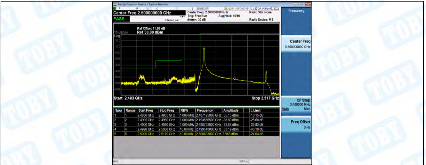
Band7-15MHz-16QAM-20825-1RB#74
