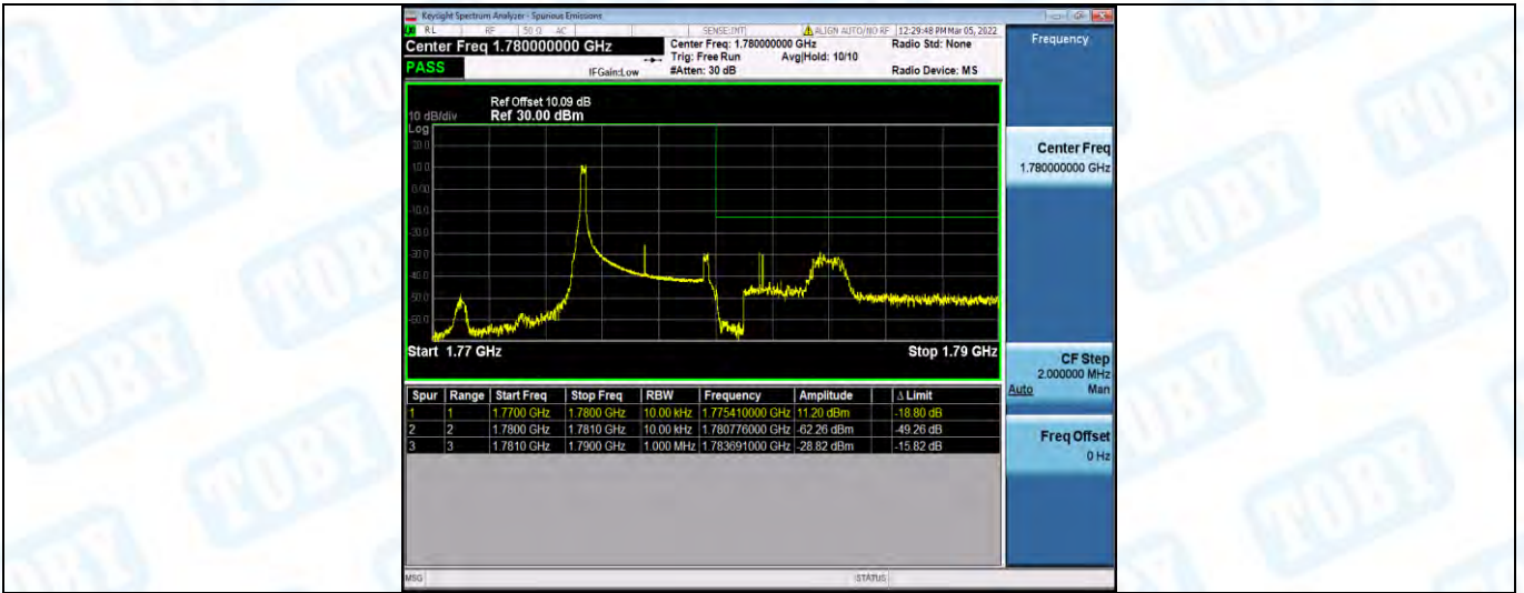
Band66-5MHz-QPSK-132647-1RB#24
