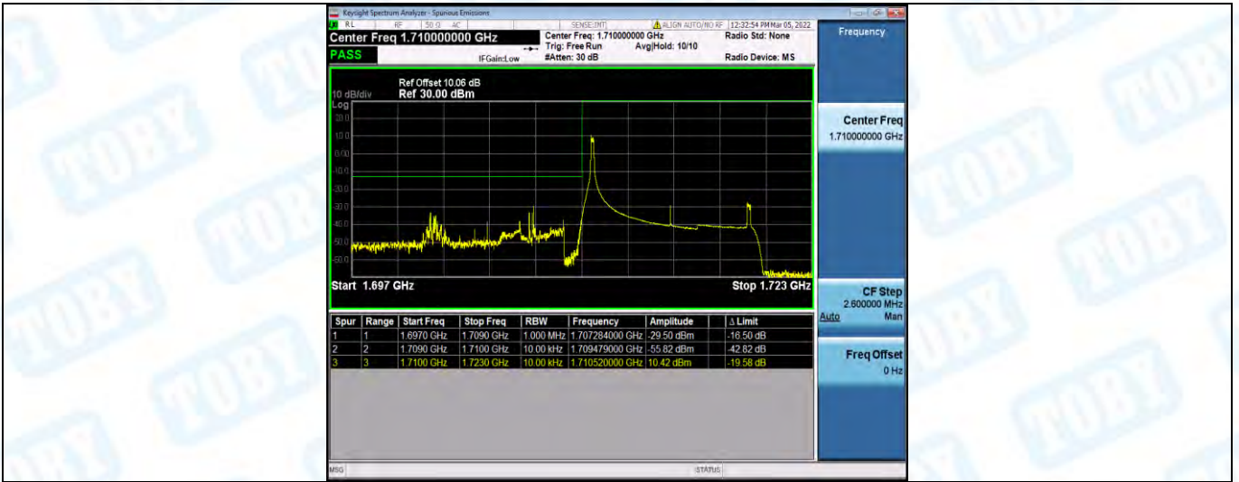
Band66-10MHz-16QAM-132022-1RB#49
