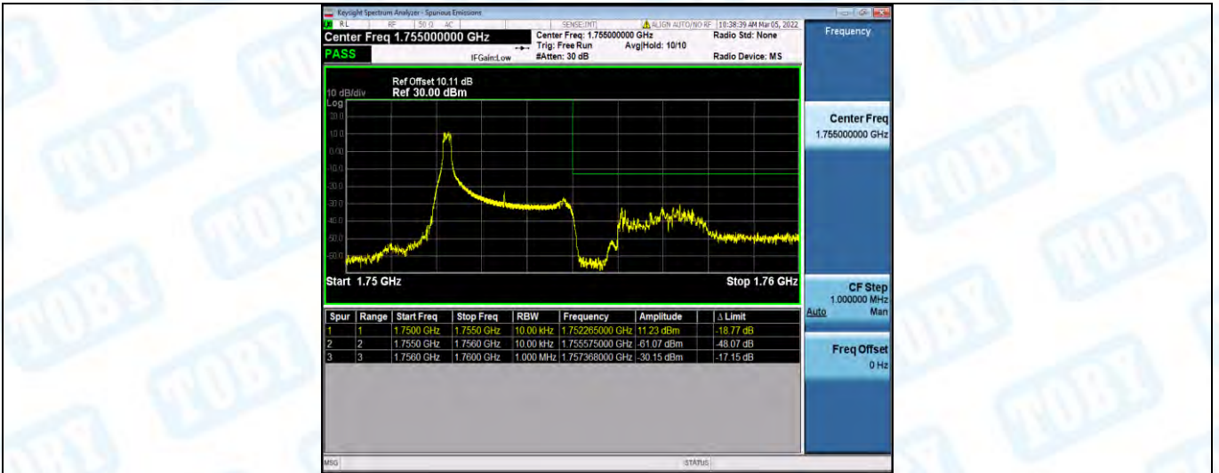
Band4-3MHz-16QAM-20385-1RB#14
