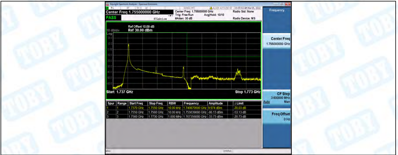
Band4-15MHz-16QAM-20325-1RB#74
