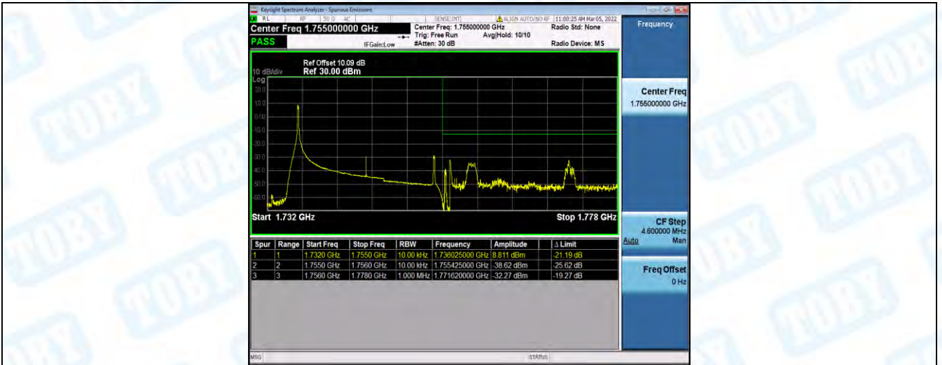
Band4-20MHz-16QAM-20300-1RB#99
