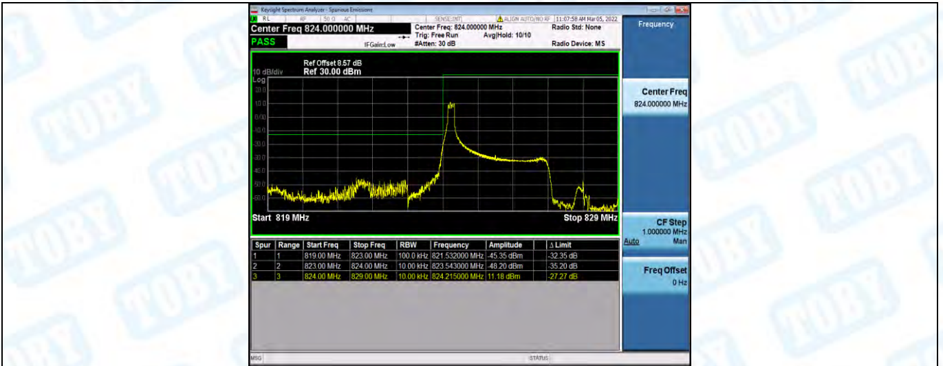
Band5-3MHz-QPSK-20415-1RB#14
