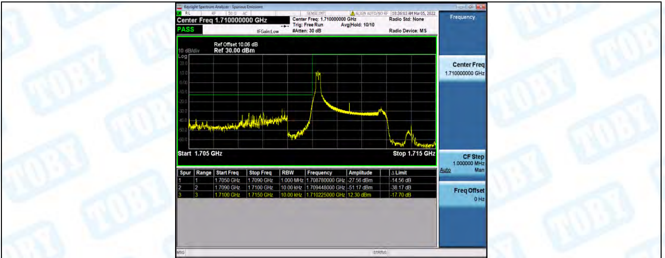
Band4-3MHz-16QAM-19965-1RB#14
