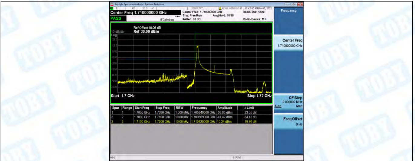
Band4-5MHz-16QAM-19975-1RB#24
