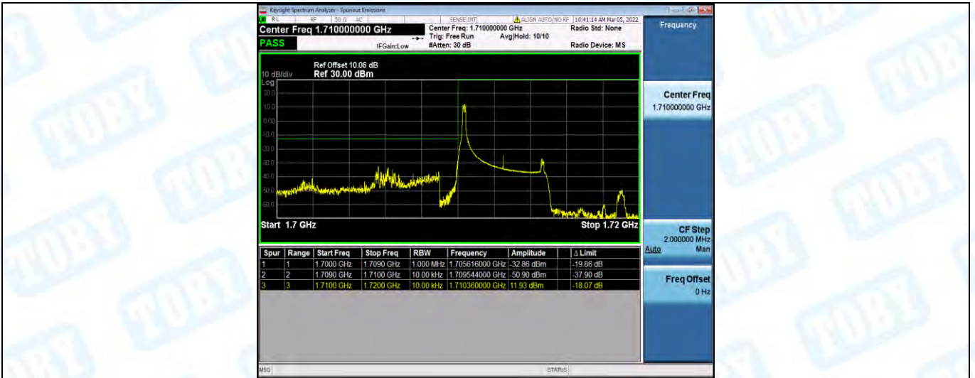
Band4-5MHz-QPSK-19975-1RB#24
