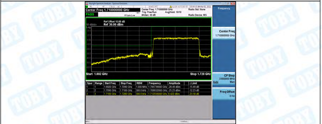
Band4-15MHz-16QAM-2025-1RB#0
