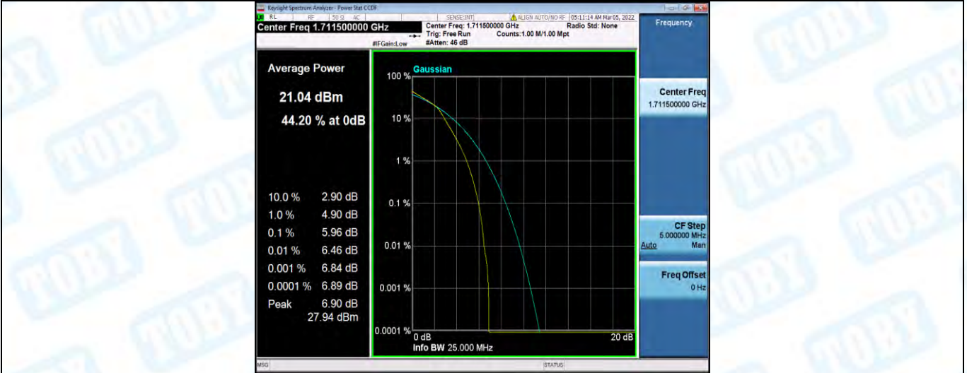
Band66-3MHz-16QAM-132322-1RB#0
