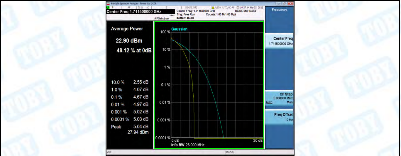
Band66-3MHz-QPSK-131987-15RB#0
