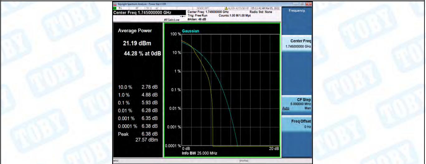
Band66-3MHz-16QAM-132322-15RB#0
