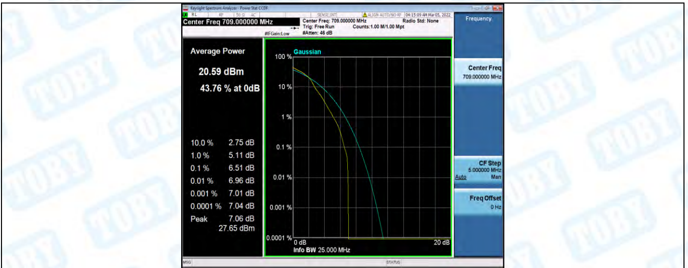
Band17-10MHz-16QAM-23780-50RB#0
