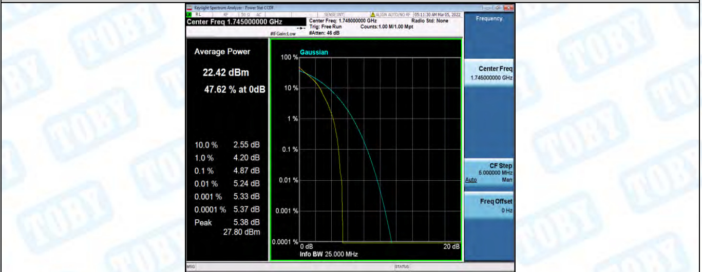
Band66-3MHz-QPSK-132322-15RB#0
