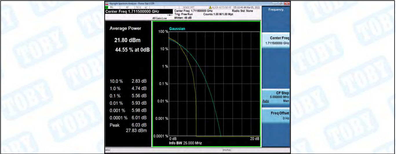
Band66-3MHz-16QAM-131987-15RB#0
