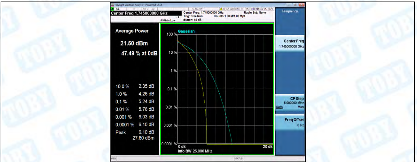
Band66-5MHz-QPSK-132647-1RB#0
