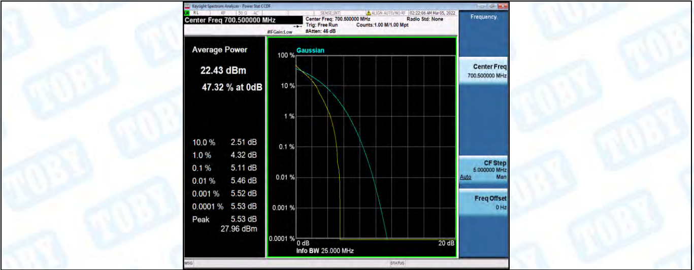
Band12-3MHz-QPSK-23025-15RB#0
