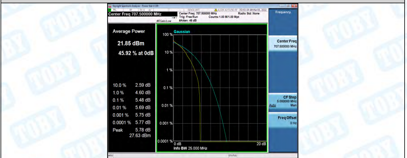
Band12-5MHz-QPSK-23095-25RB#0
