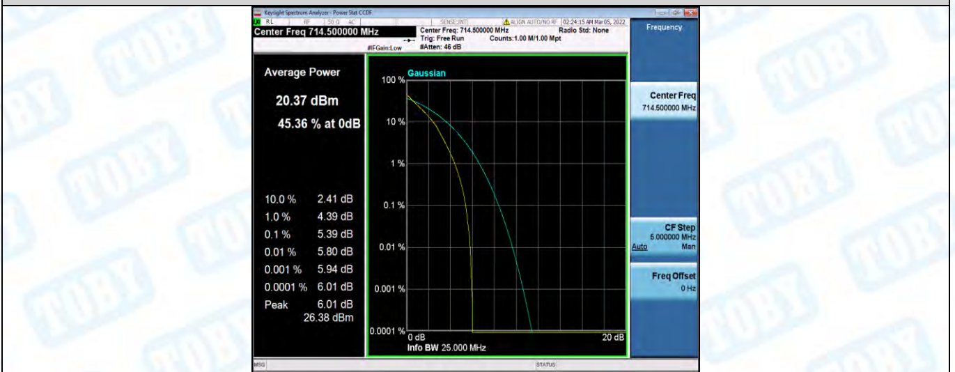
Band12-3MHz-16QAM-23025-1RB#0
