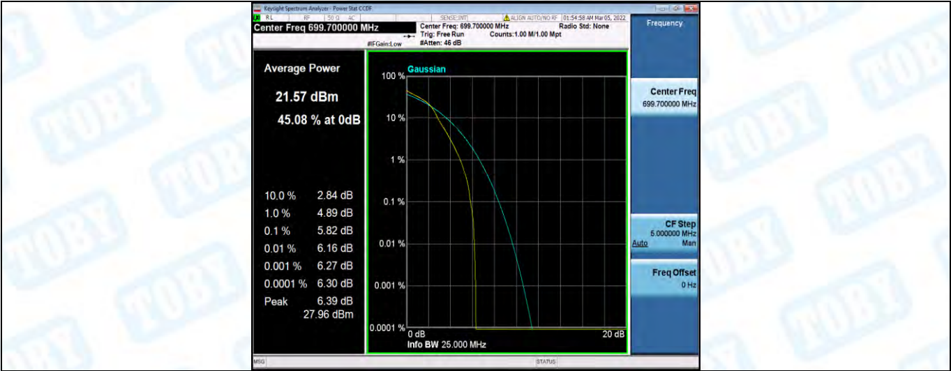
Band12-1.4MHz-16QAM-23017-6RB#0
