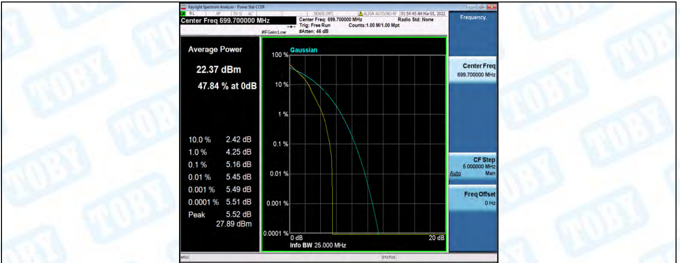
Band12-1.4MHz-QPSK-23017-6RB#0
