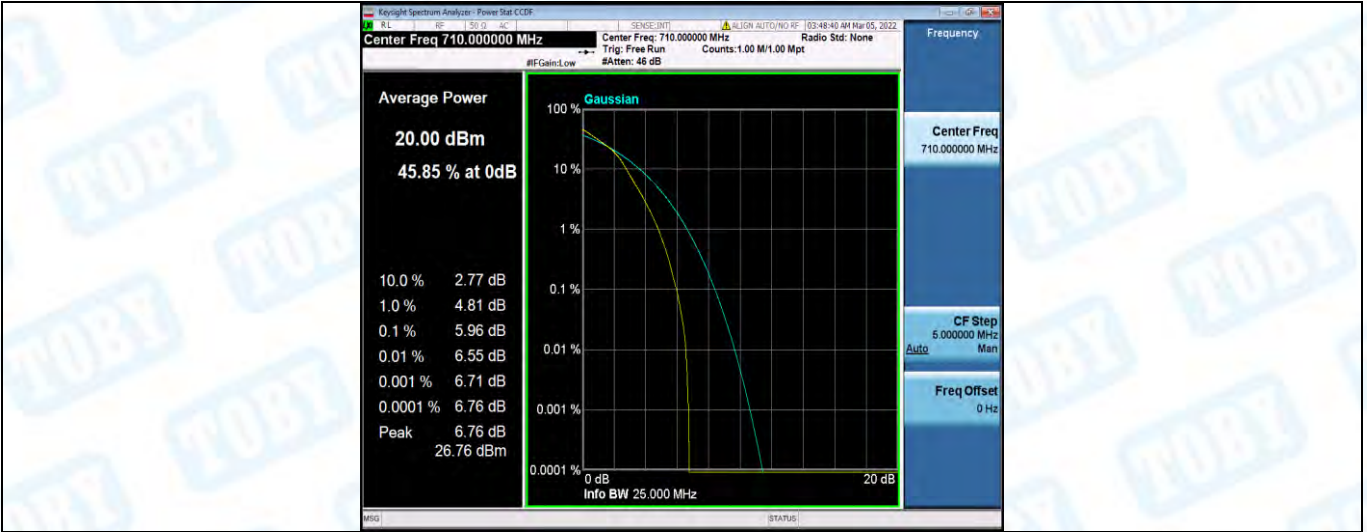
Band17-5MHz-16QAM-23825-1RB#0
