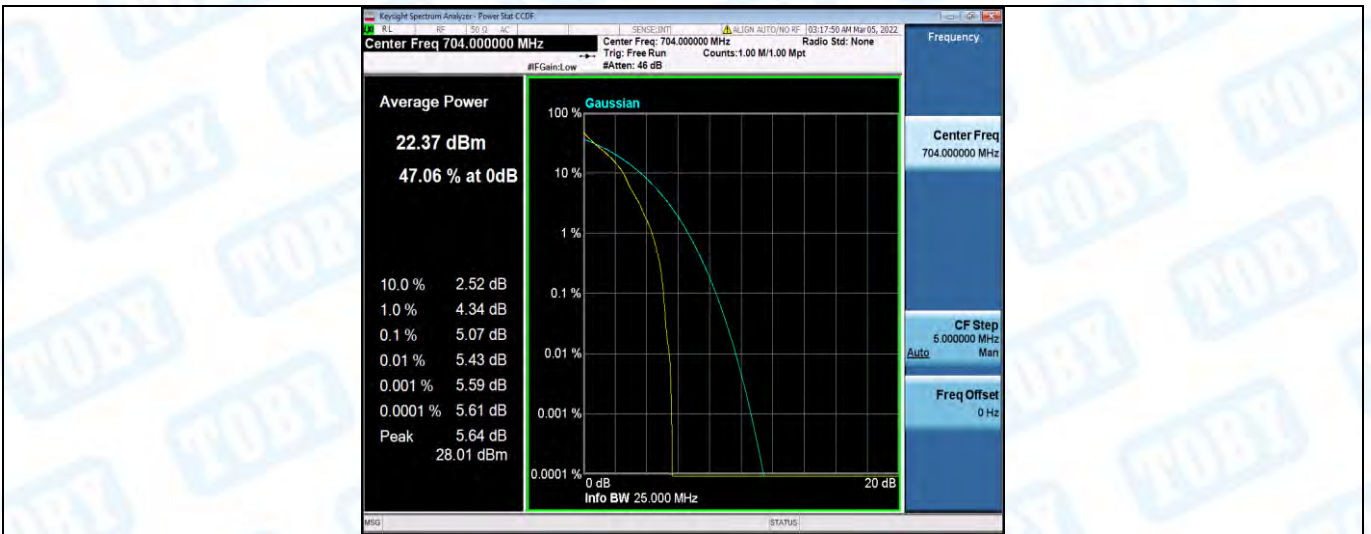
Band12-10MHz-QPSK-23060-50RB#0
