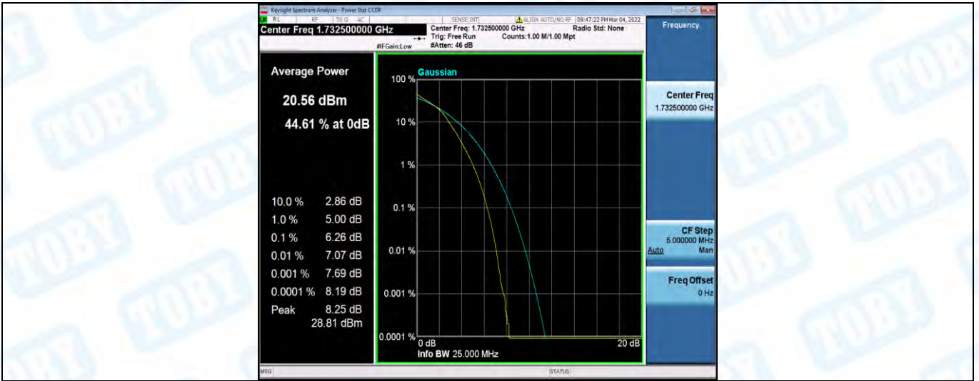
Band4-20MHz-16QAM-20300-1RB#0
