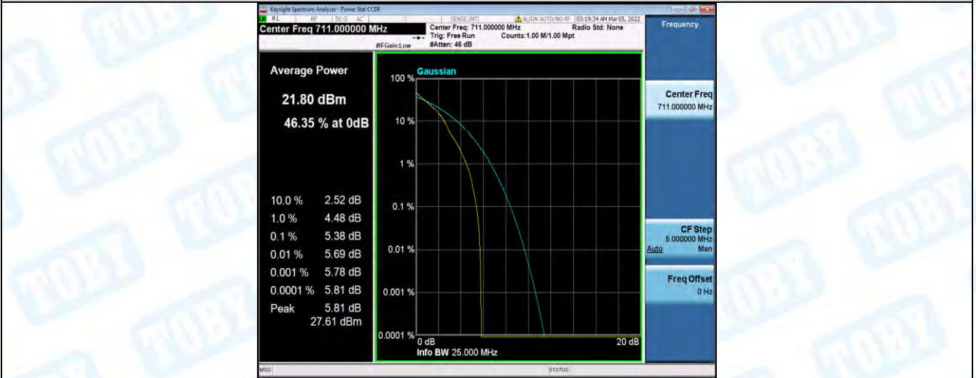
Band12-10MHz-QPSK-23130-50RB#0
