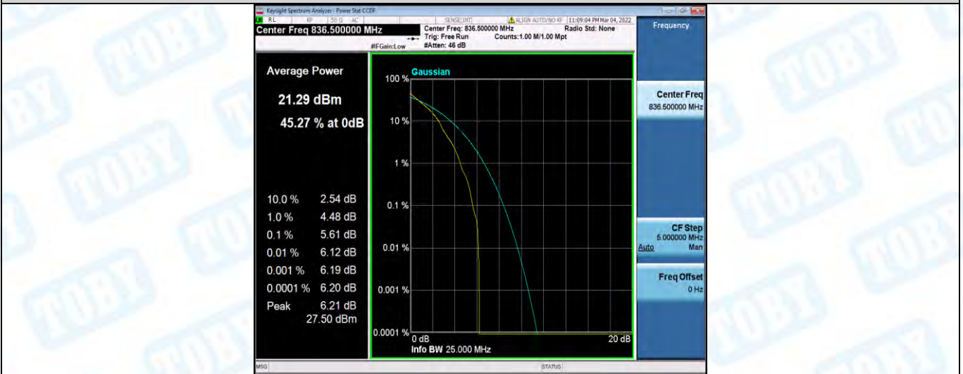
Band5-5MHz-QPSK-20525-25RB#0
