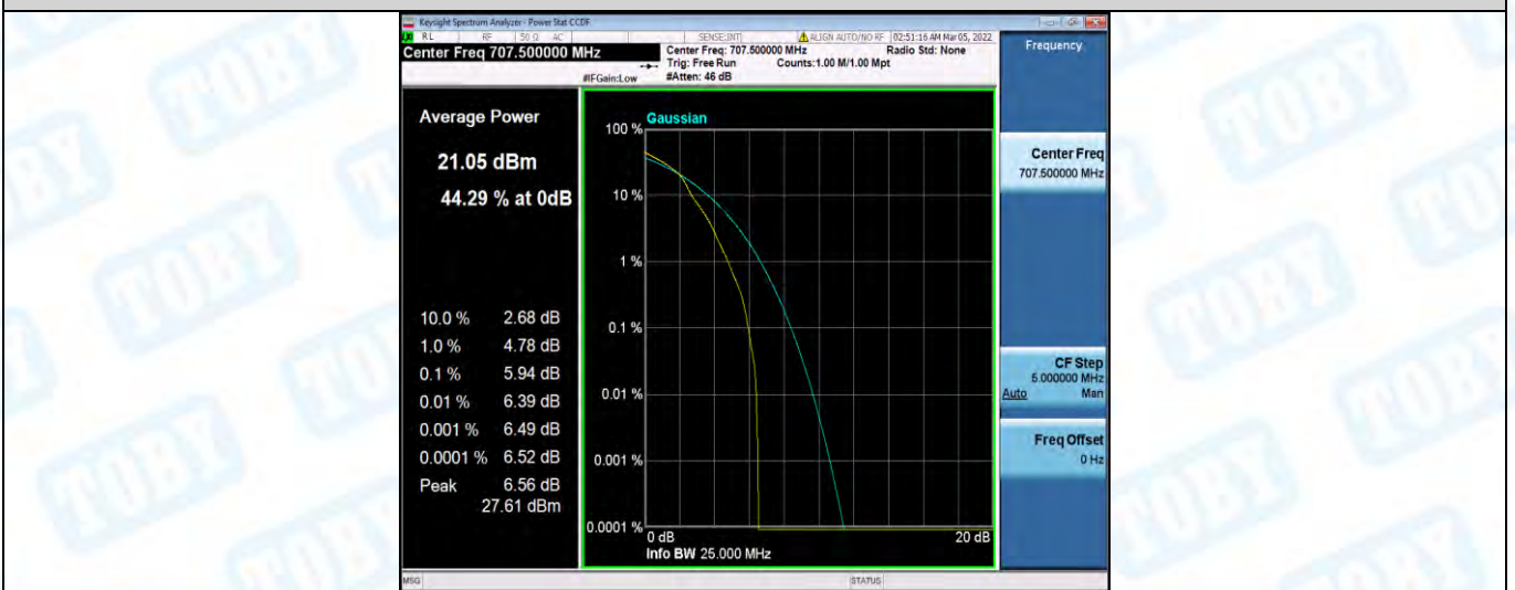
Band12-5MHz-16QAM-23095-25RB#0
