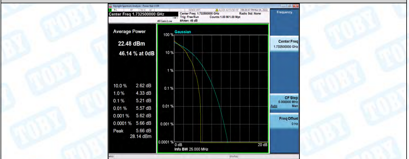
Band4-5MHz-QPSK-20175-25RB#0
