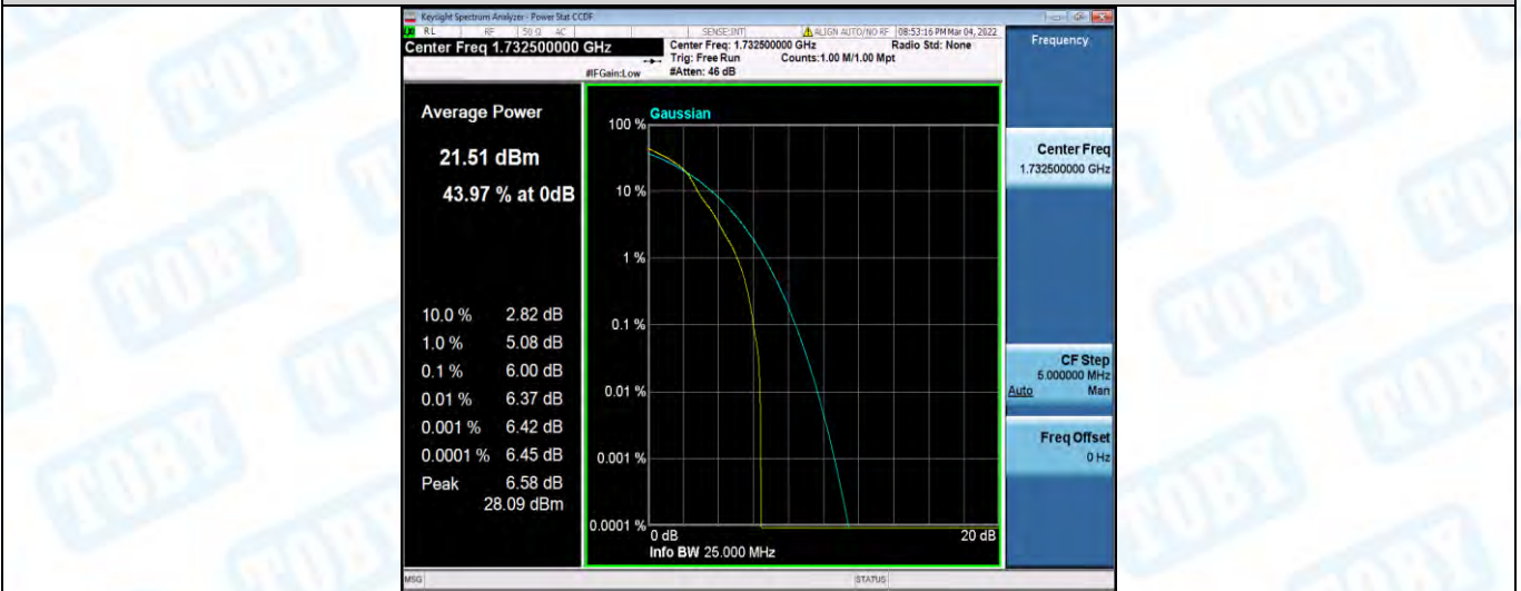
Band4-10MHz-16QAM-20175-50RB#0
