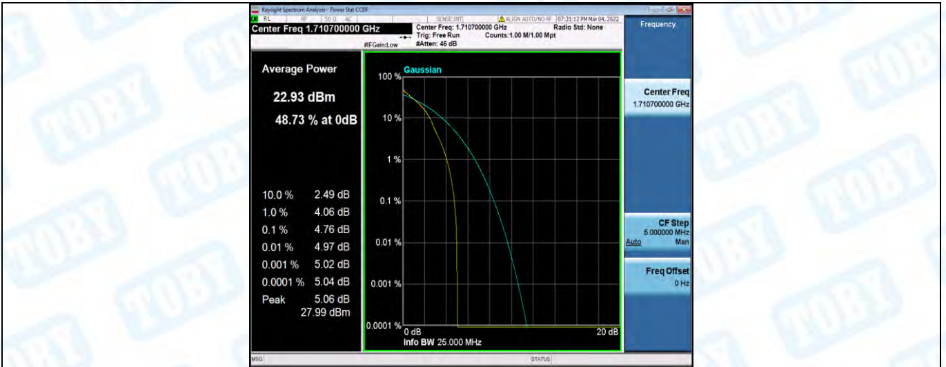
Band4-1.4MHz-QPSK-19957-6RB#0
