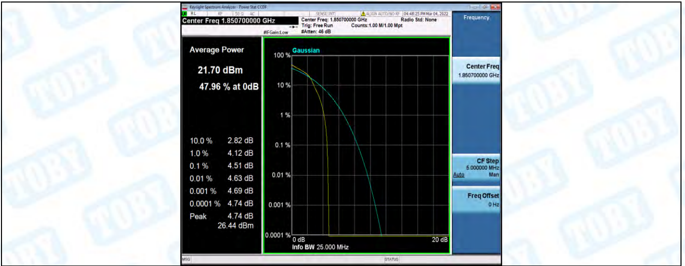
Band2-1.4MHz-16QAM-18607-6RB#0
