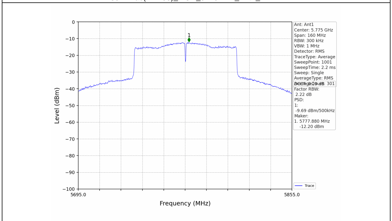
802.11ac(VHT80)_MCH_5775MHz_Ant1_NTNV
