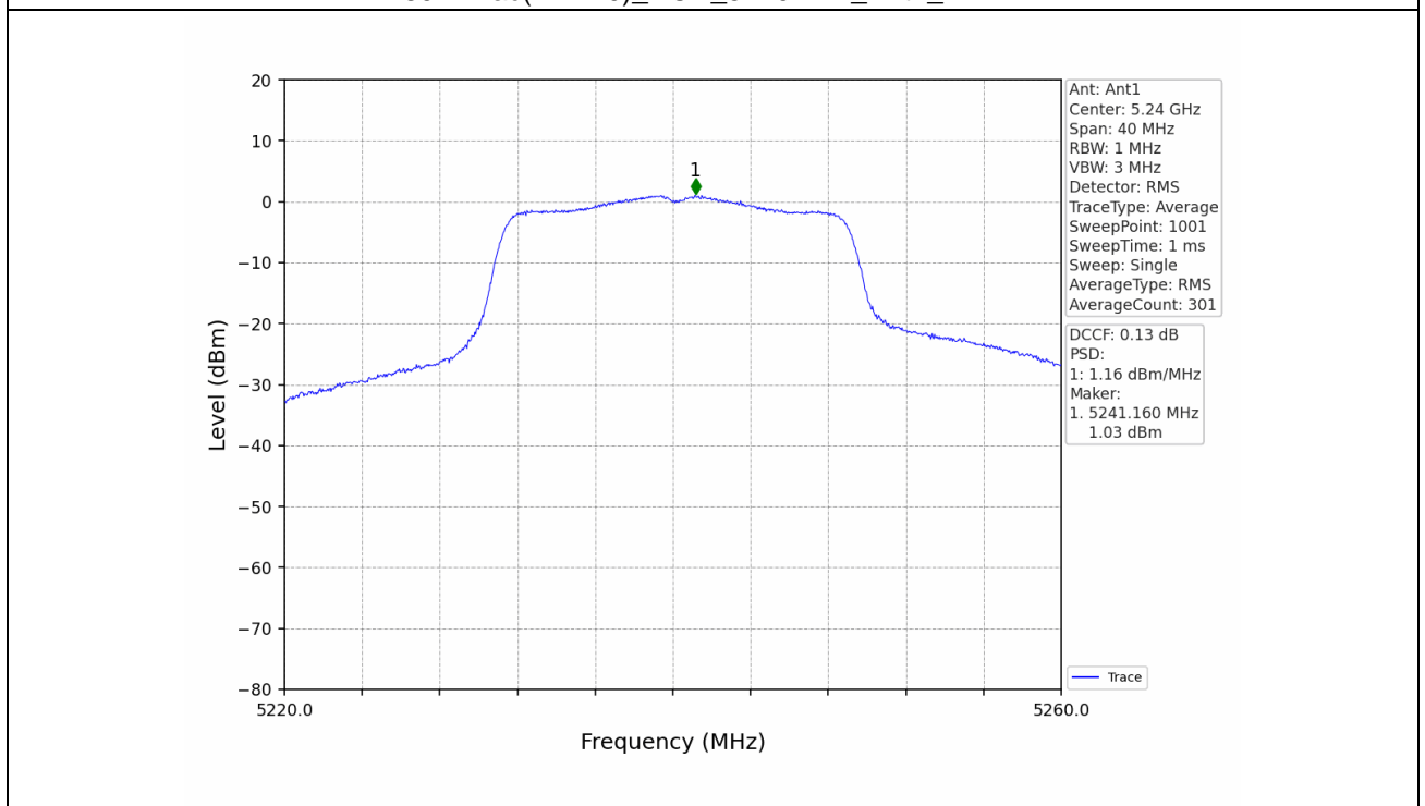
802.11ac(VHT20)_HCH_5240MHz_Ant1_NTNV
