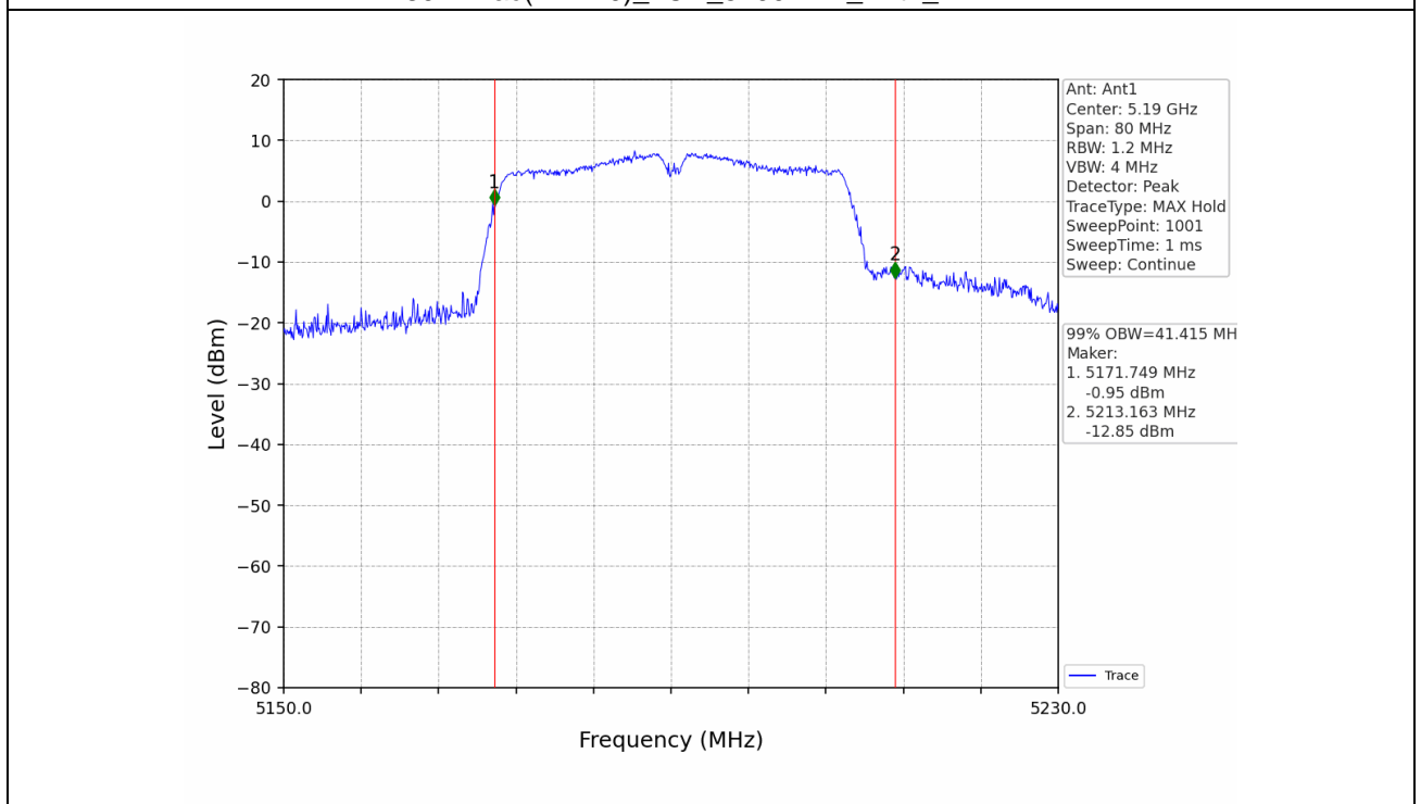
802.11ac(VHT40)_LCH_5190MHz_Ant1_NTNV
