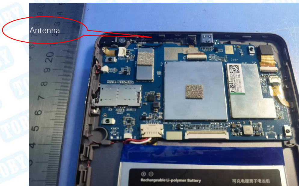
Photo 10 Internal of EUT
