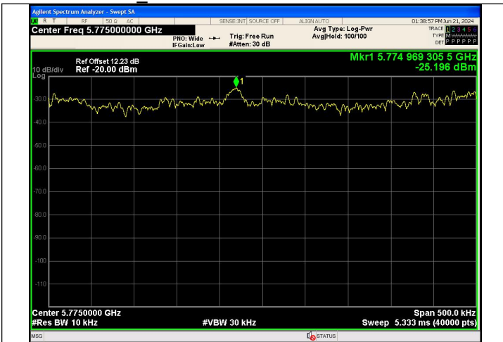
NT/NV_Antenna 0 IEEE 802.11ac_Channel 155_80MHz
