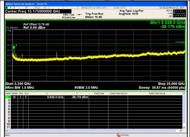
Spurious Emission:5350~25000.0 MHz IEEE 802.11a Channel 40 20MHz Antenna 0
