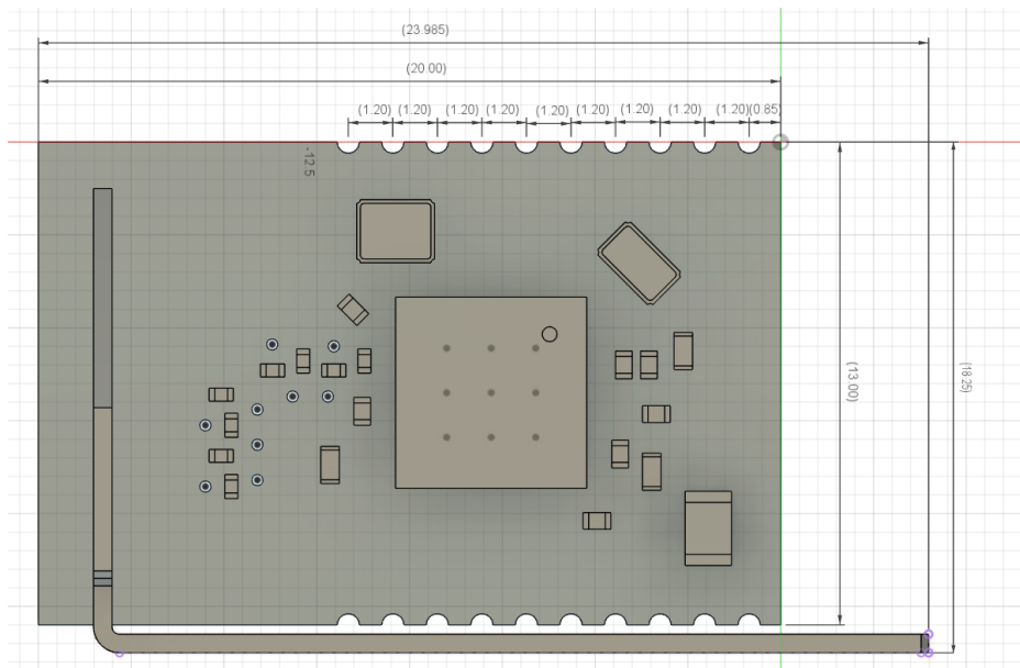
Figure 1: Top view sepioo S1 module
