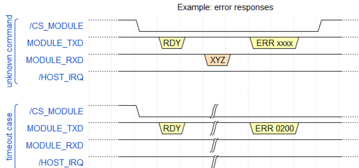
Figure 3 error responses
