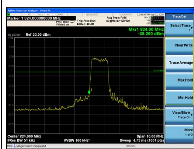
LTE Band 26 QPSK 3MHz CH-Low 1RB
