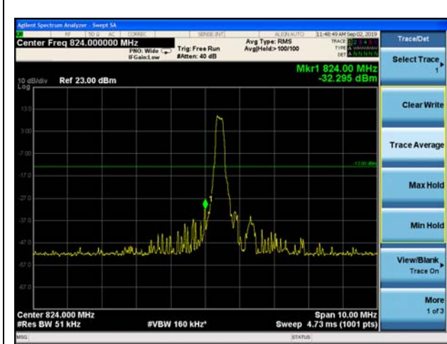
LTE Band 26 QPSK 3MHz CH-Low 1RB
