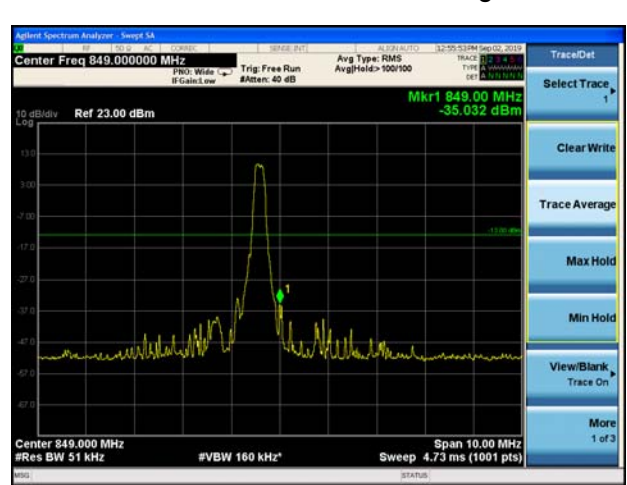
LTE Band 26 QPSK 3MHz CH-High 1RB
