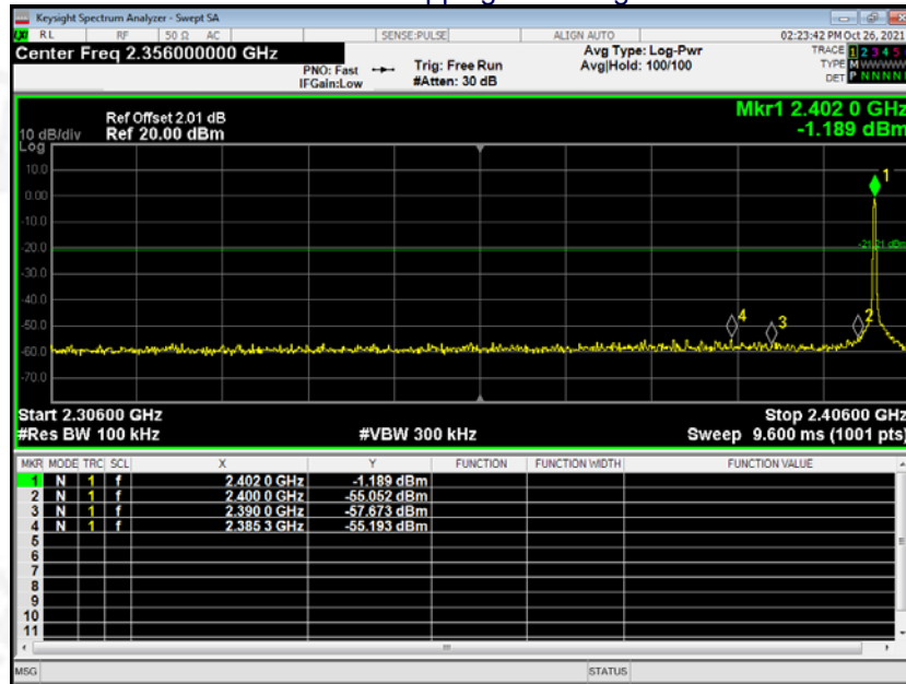
GFSK No-hopping Band edge-left side
