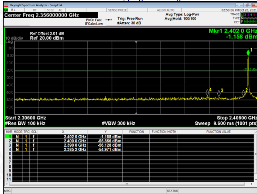
8DPSK No-hopping Band edge-left side
