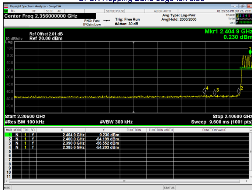
GFSK Hopping Band edge-left side
