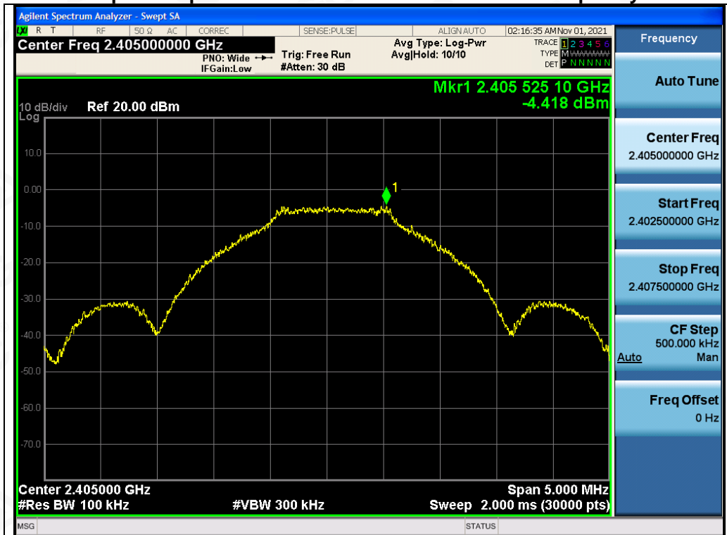
Test_Graph_LE2M_ANT1_2405_2Mbps_Reference Level
