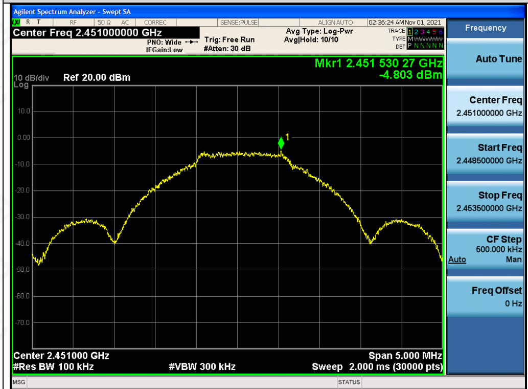
Test_Graph_LE2M_ANT1_2451_2Mbps_Reference Level
