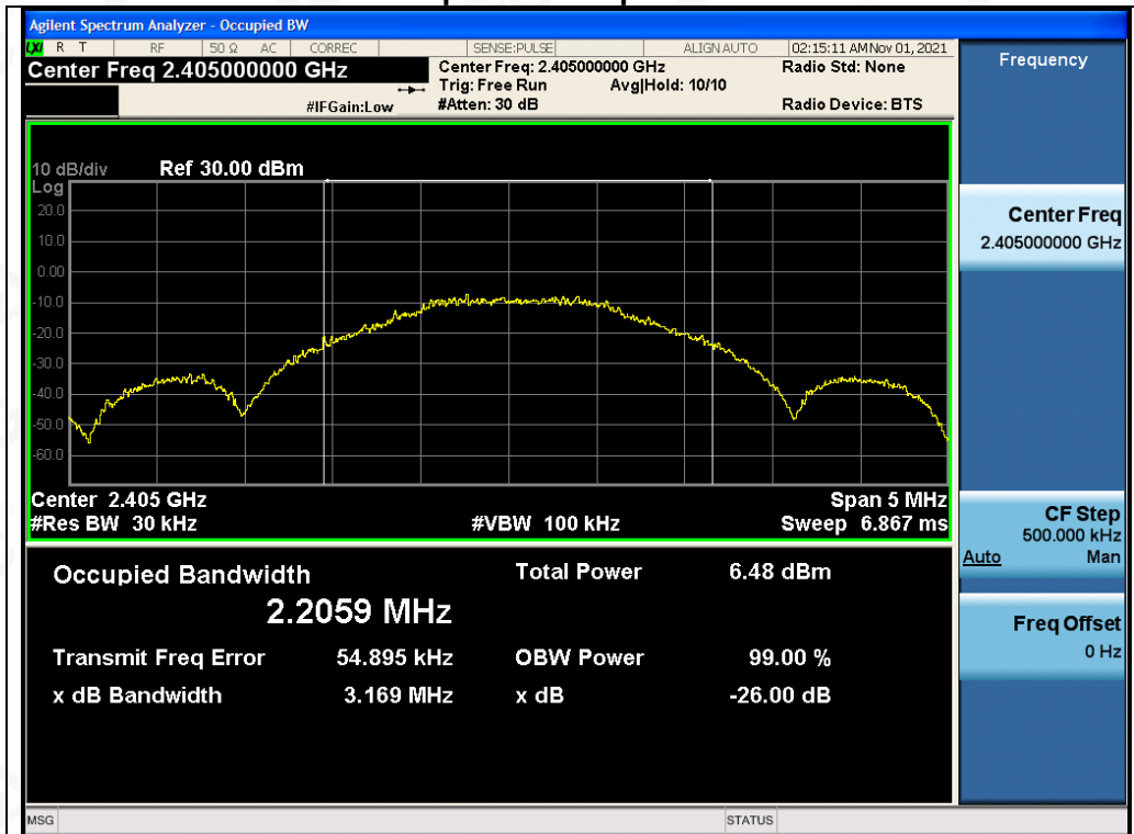
Test_Graph_LE2M_ANT1_2405_2Mbps_OBW
