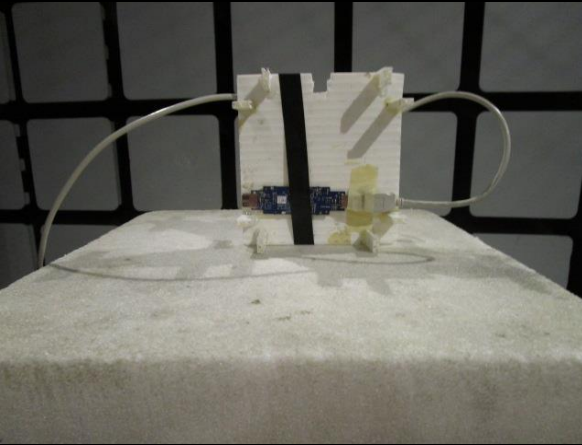
EUT Horizontal – Radiated
