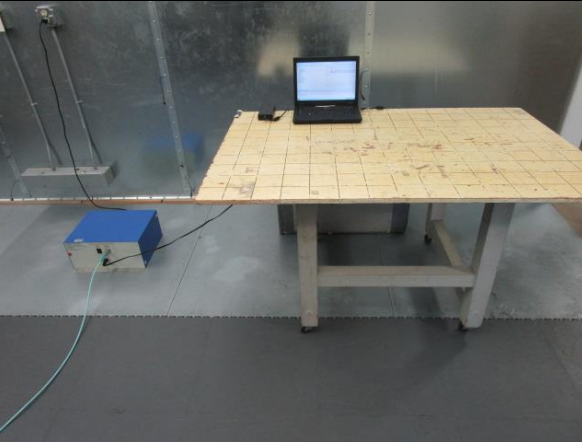
AC Mains Emissions Setup
