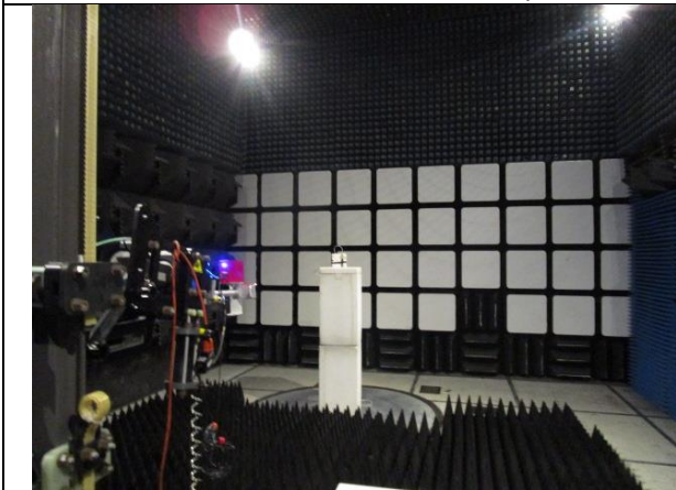
18-25 GHz Radiated Setup
