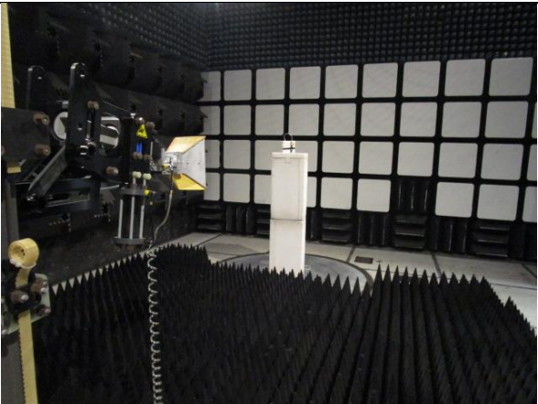
1-18 GHz Radiated Setup
