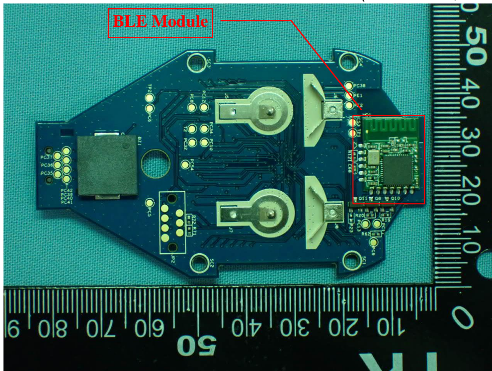
Figure 11 Internal View (Main Board, Back View)
