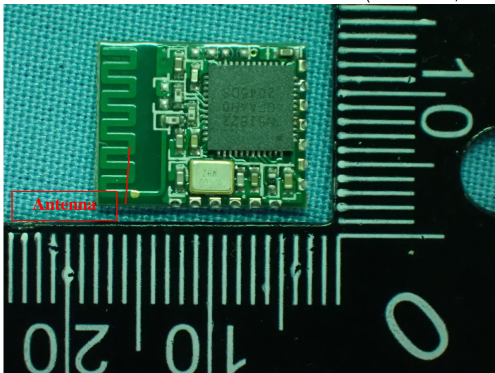
Figure 14 Internal View (BT Module, Front View)
