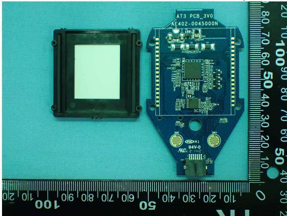
Figure 9 Internal View (Removed Panel)
