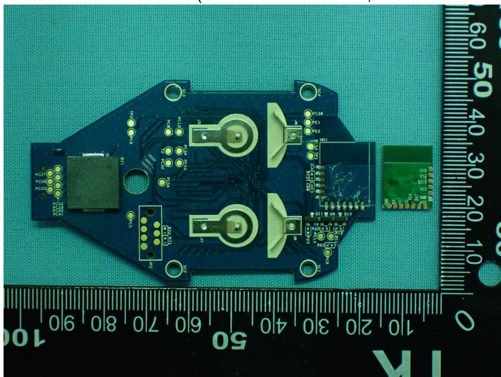
Figure 12 Internal View (Removed BT Module, Main Board/Back View)
