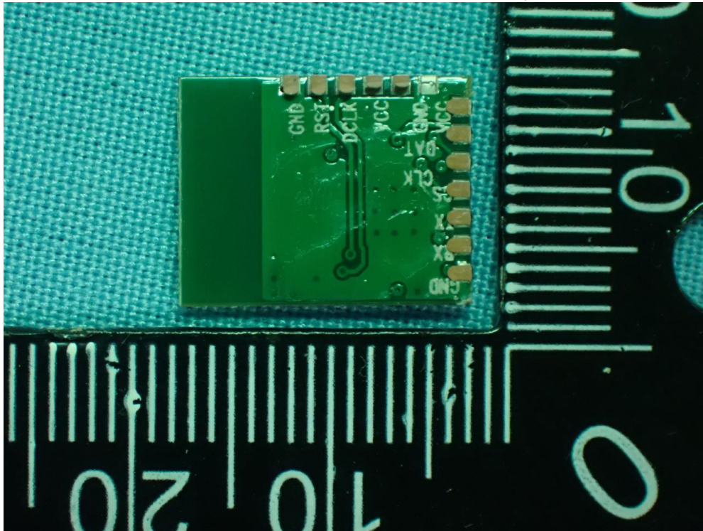
Figure 13 Internal View (BT Module, Back View)
