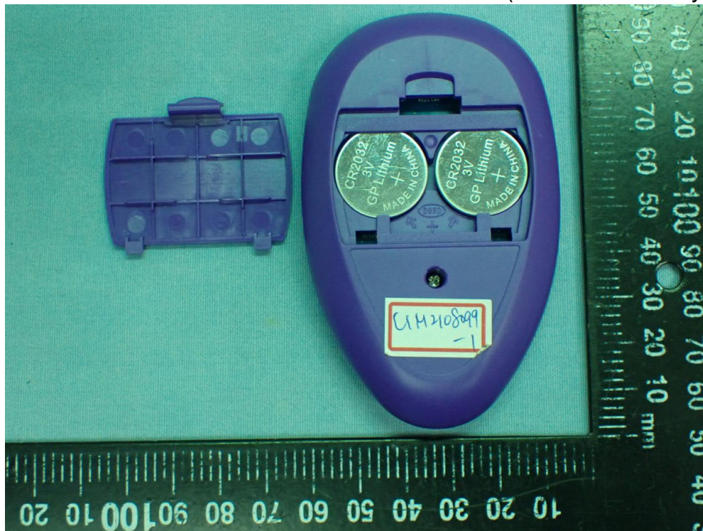
Figure 8 Internal View (Removed Covers)
