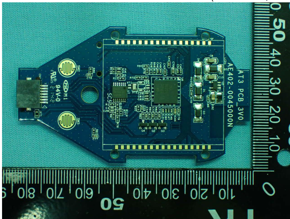
Figure 10 Internal View (Main Board, Front View)
