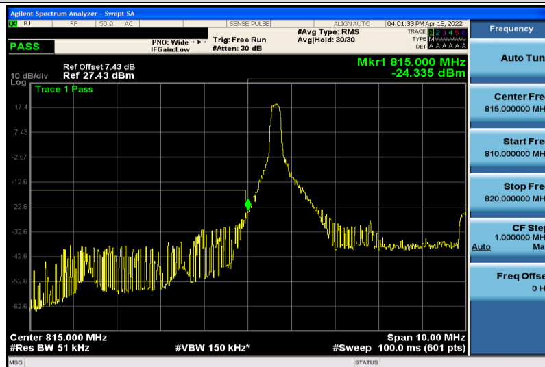
Band18-5MHz-16QAM-23875-1RB#0
