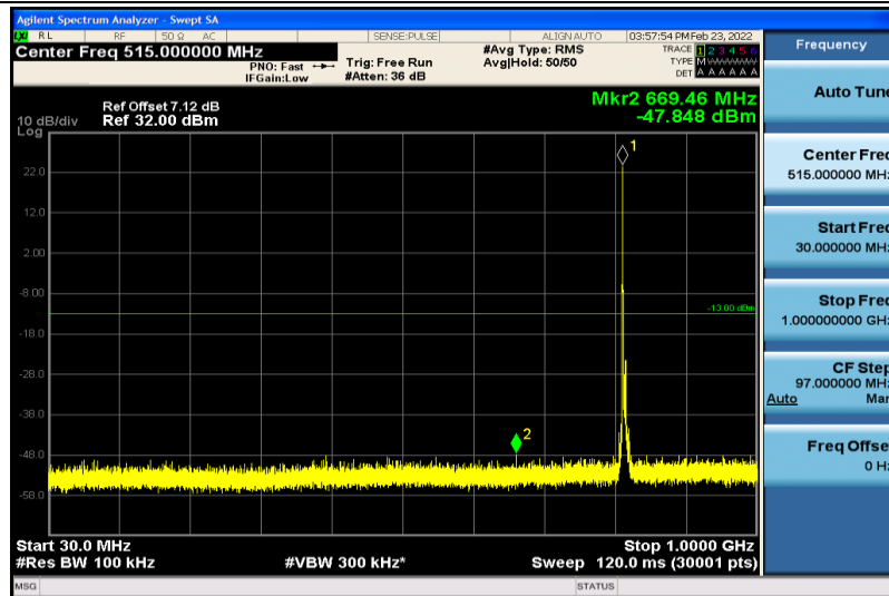
Band18-5MHz-16QAM-23875-1RB#0-30~1000MHz
