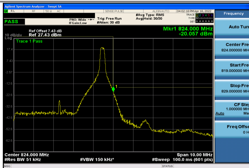
Band18-5MHz-QPSK-23915-1RB#24
