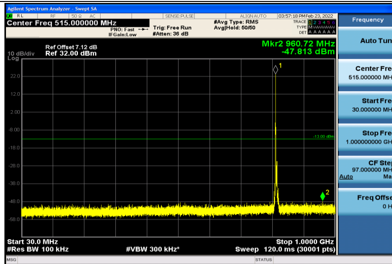
Band18-5MHz-QPSK-23875-1RB#0-30~1000MHz
