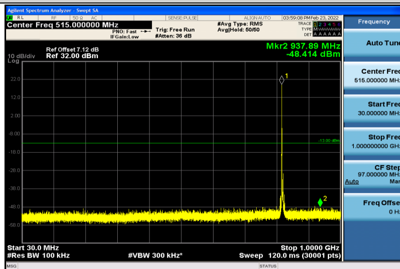
Band18-5MHz-16QAM-23895-1RB#0-30~1000MHz
