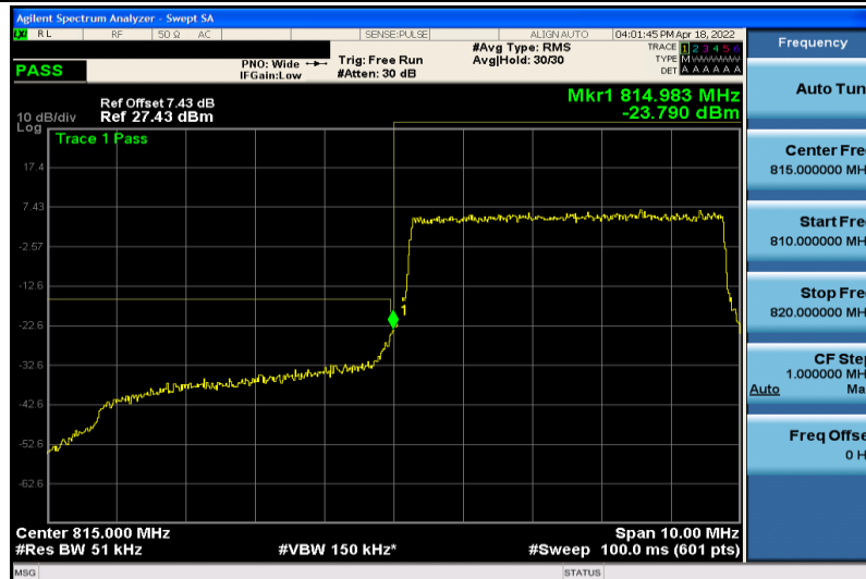
Band18-5MHz-QPSK-23875-25RB#0
