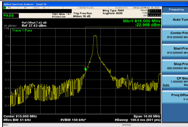
Band18-5MHz-QPSK-23875-1RB#0
