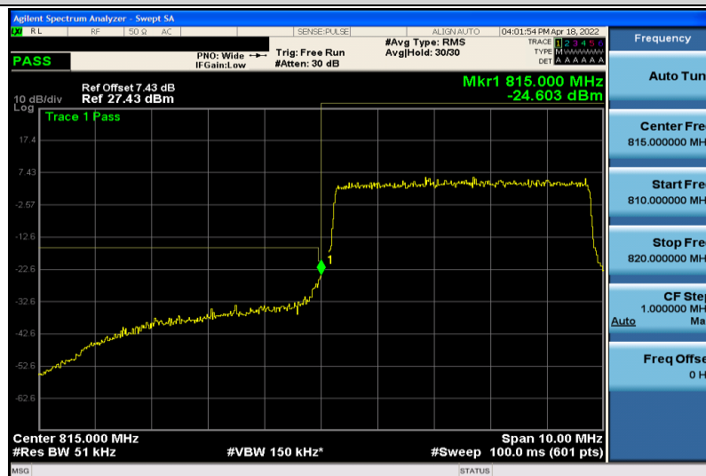
Band18-5MHz-16QAM-23875-25RB#0
