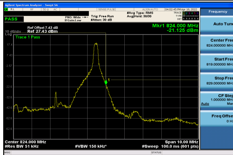
Band18-5MHz-16QAM-23915-1RB#24
