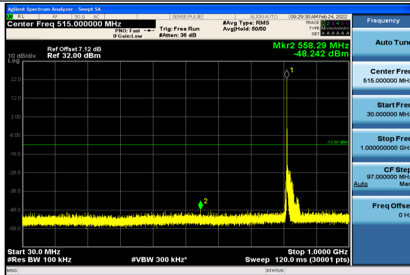
Band26-5MHz-QPSK-26715-1RB#0-30~1000MHz
