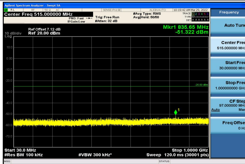
Band41-5MHz-16QAM-40640-1RB#0-30~1000MHz
