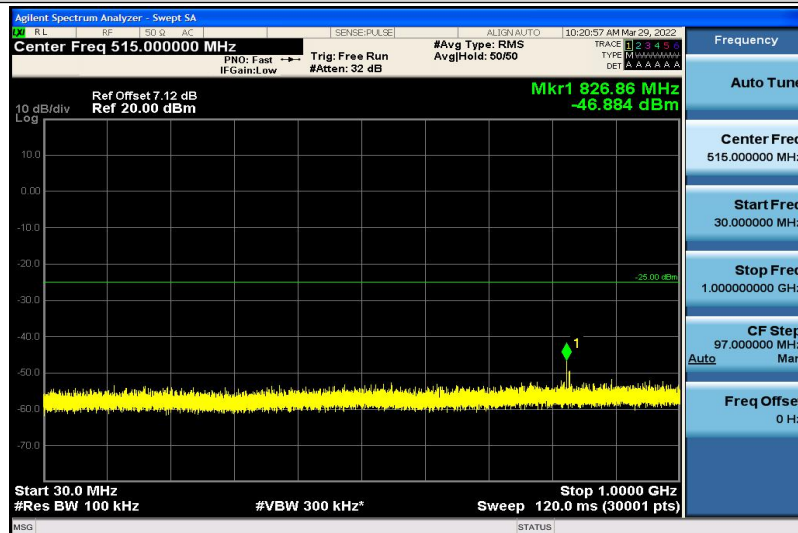
Band41-5MHz-16QAM-41215-1RB#0-30~1000MHz
