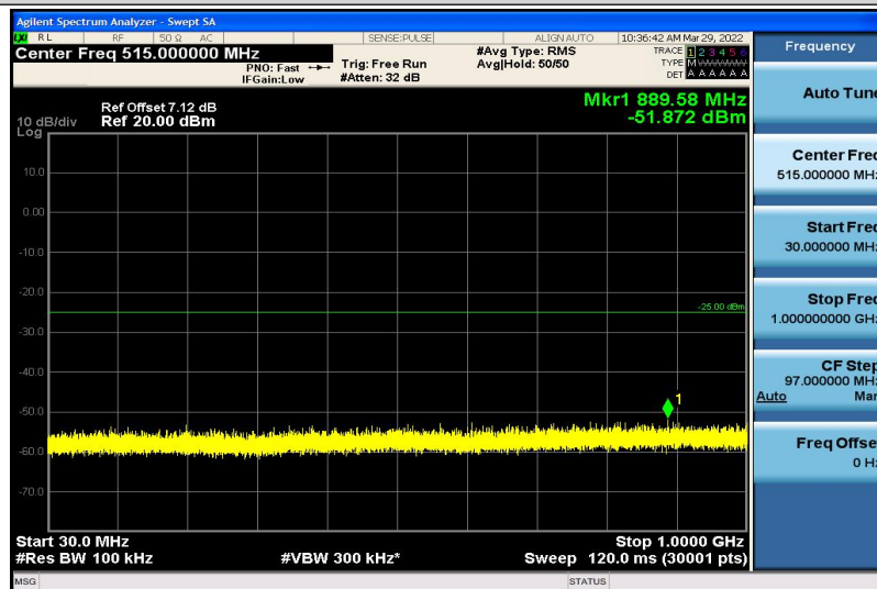
Band41-10MHz-QPSK-40090-1RB#0-30~1000MHz
