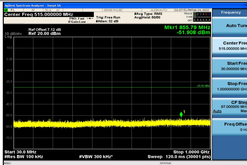
Band38-15MHz-16QAM-38175-1RB#0-30~1000MHz
