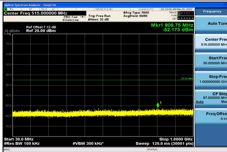
Band41-5MHz-QPSK-40640-1RB#0-30~1000MHz
