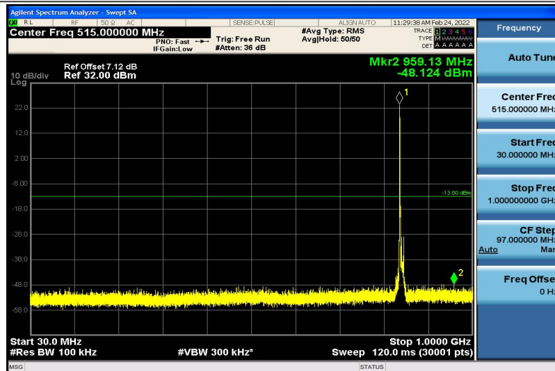
Band26-10MHz-16QAM-26990-1RB#0-30~1000MHz
