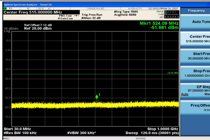
Band38-5MHz-16QAM-38225-1RB#0-30~1000MHz
