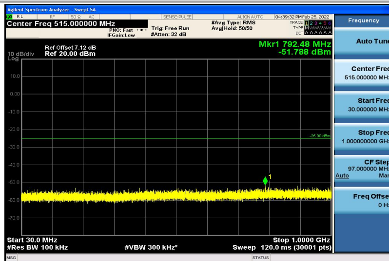
Band38-10MHz-QPSK-37800-1RB#0-30~1000MHz
