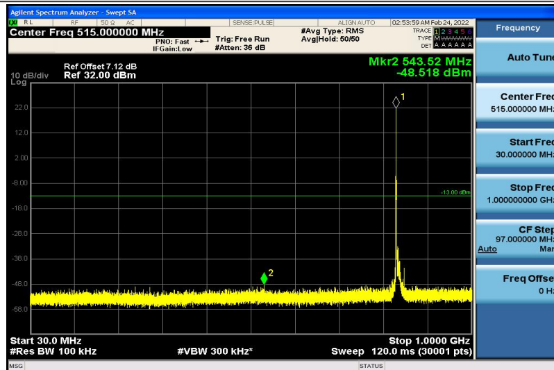
Band19-10MHz-QPSK-24075-1RB#0-30~1000MHz
