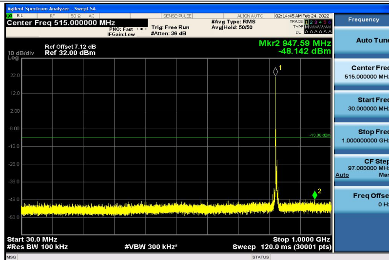
Band18-5MHz-16QAM-23970-1RB#0-30~1000MHz
