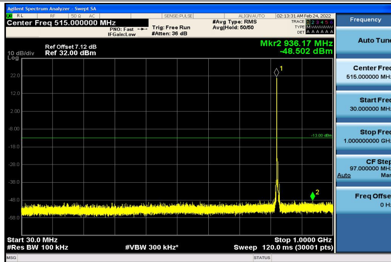
Band18-5MHz-16QAM-23965-1RB#0-30~1000MHz
