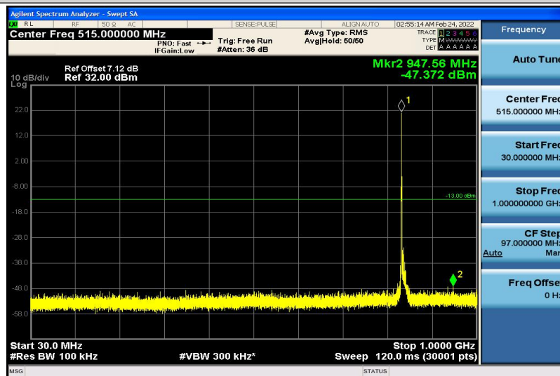
Band19-10MHz-QPSK-24100-1RB#0-30~1000MHz
