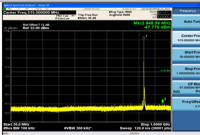
Band19-5MHz-QPSK-24075-1RB#0-30~1000MHz
