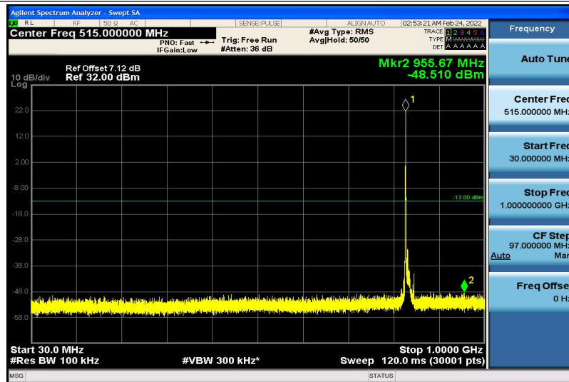
Band19-10MHz-16QAM-24050-1RB#0-30~1000MHz
