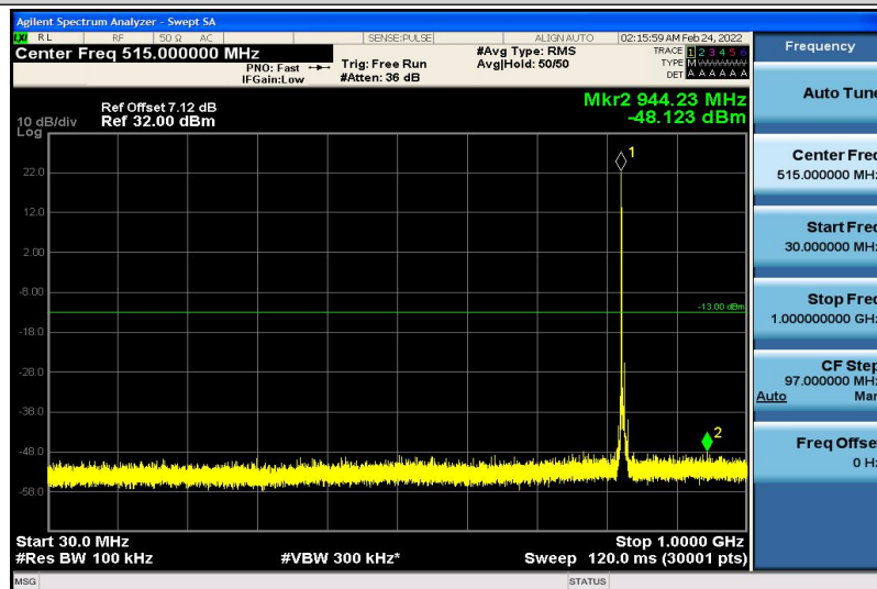
Band18-5MHz-16QAM-23975-1RB#0-30~1000MHz
