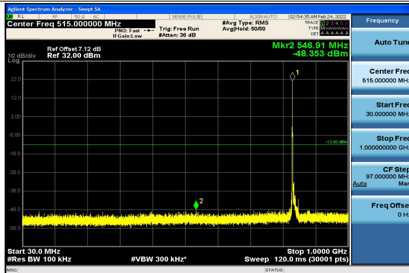
Band19-10MHz-16QAM-24075-1RB#0-30~1000MHz
