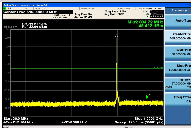
Band12-10MHz-16QAM-23095-1RB#0-30~1000MHz
