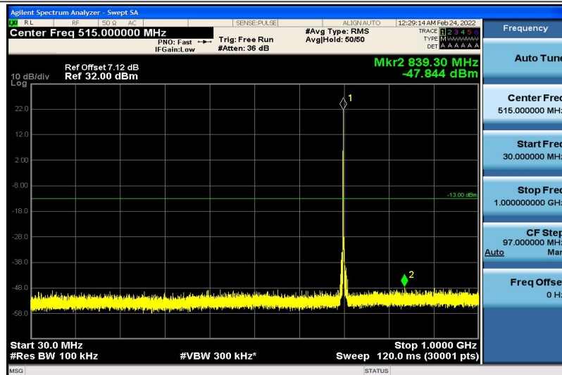
Band12-3MHz-QPSK-23095-1RB#0-30~1000MHz
