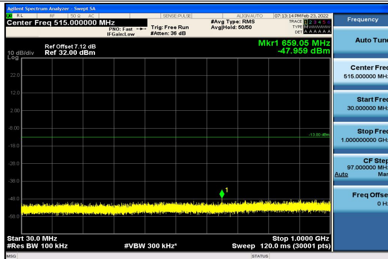
Band4-3MHz-16QAM-20175-1RB#0-30~1000MHz
