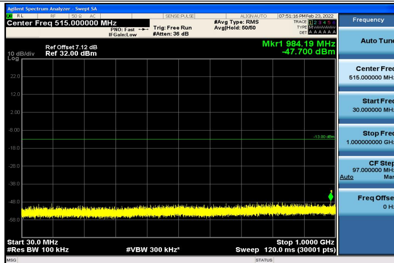
Band4-10MHz-16QAM-20175-1RB#0-30~1000MHz
