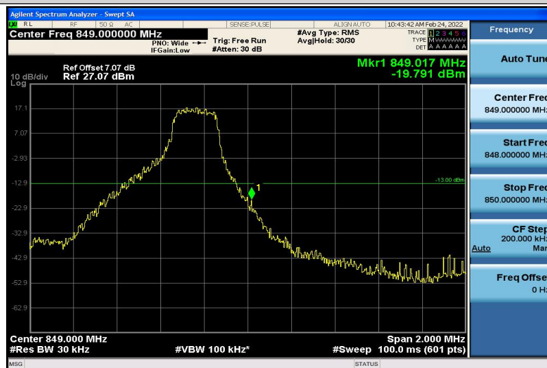
Band26-3MHz-QPSK-27025-1RB#14
