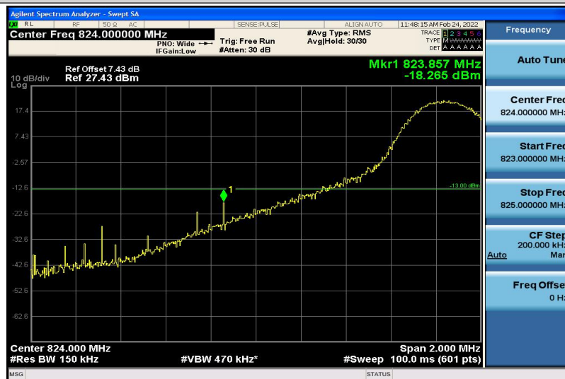
Band26-15MHz-16QAM-26865-1RB#0
