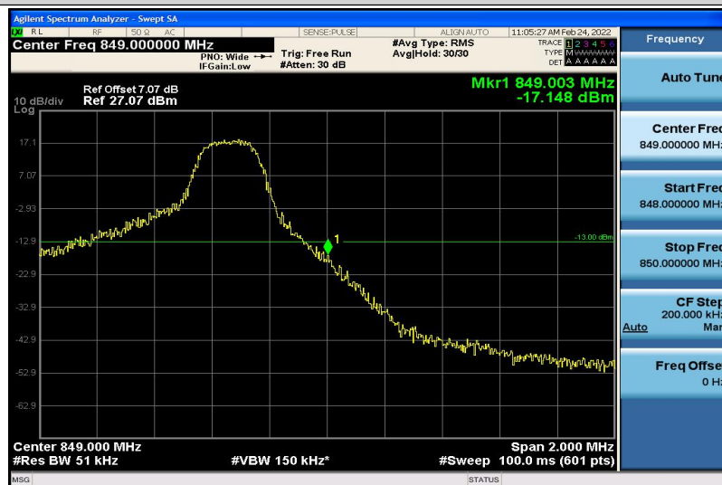
Band26-5MHz-16QAM-27015-1RB#24
