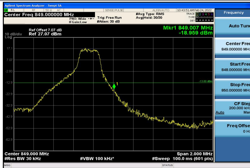
Band26-3MHz-16QAM-27025-1RB#14
