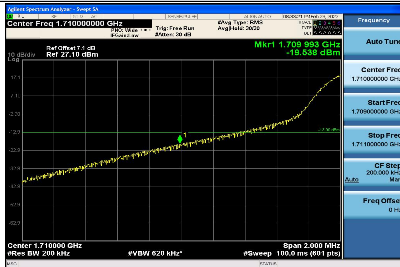
Band4-20MHz-16QAM-20050-1RB#0
