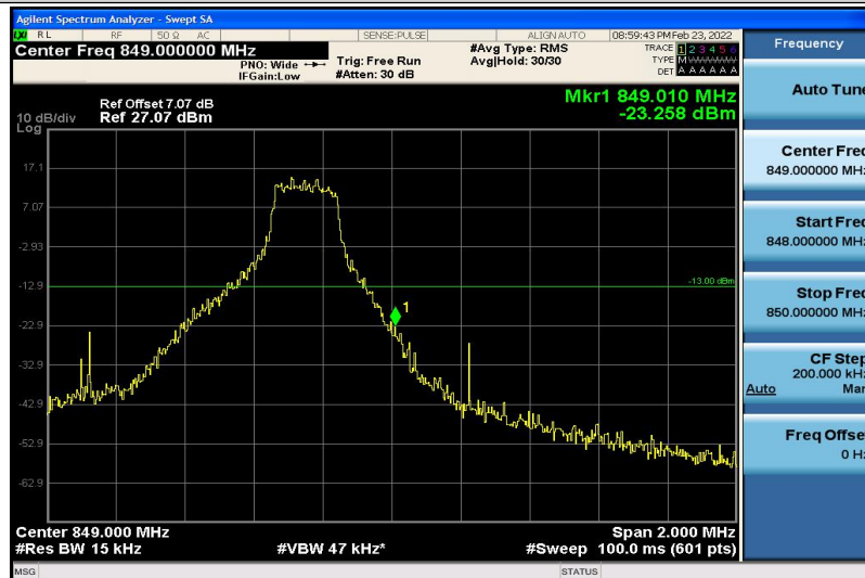
Band5-1.4MHz-QPSK-20643-1RB#5
