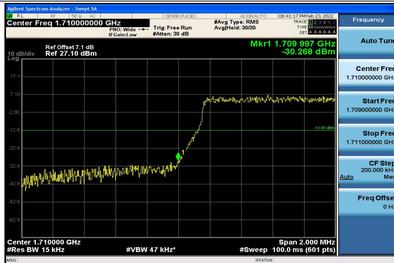
Band4-1.4MHz-16QAM-19957-6RB#0
