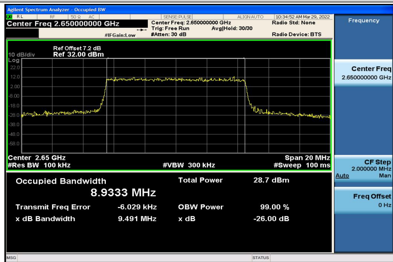
Band41-10MHz-16QAM-41190-50RB#0-8.9333
