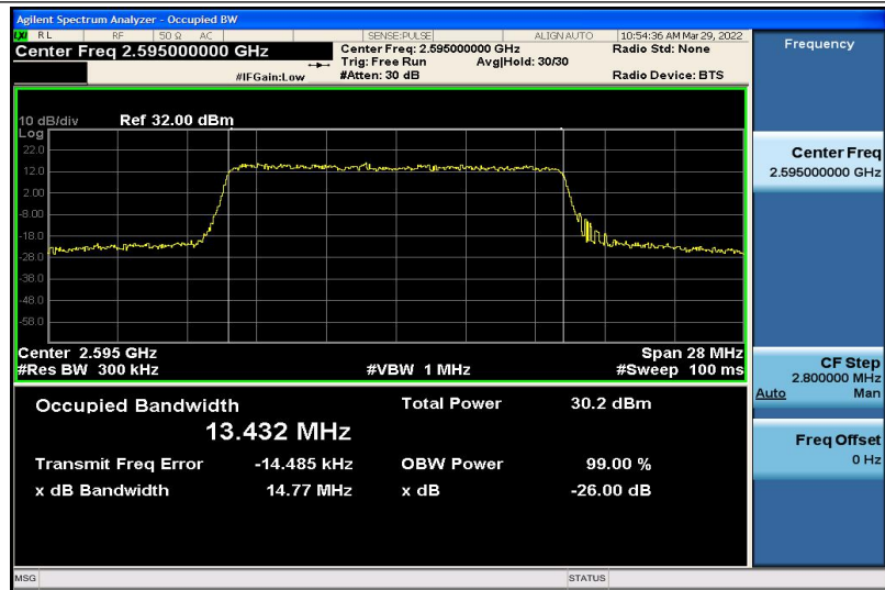
Band41-15MHz-QPSK-40640-75RB#0-13.432
