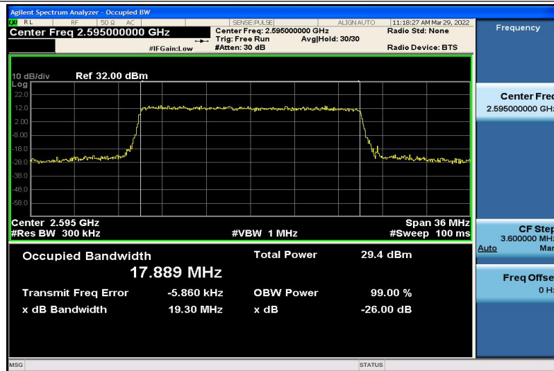
Band41-20MHz-16QAM-40640-100RB#0-17.889
