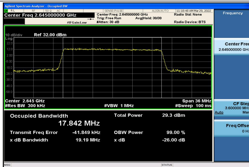
Band41-20MHz-16QAM-41140-100RB#0-17.842
