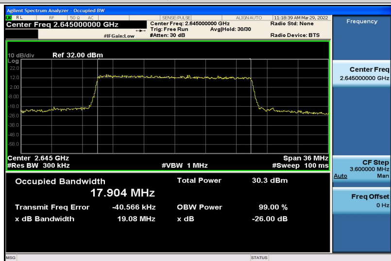
Band41-20MHz-QPSK-41140-100RB#0-17.904
