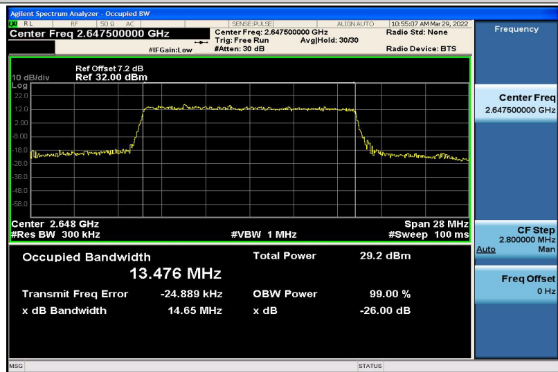
Band41-15MHz-16QAM-41165-75RB#0-13.476
