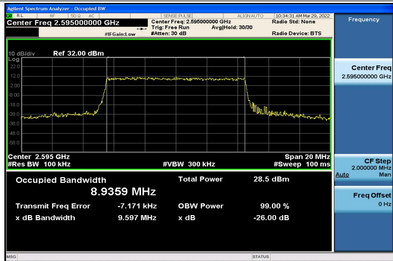
Band41-10MHz-16QAM-40640-50RB#0-8.9359
