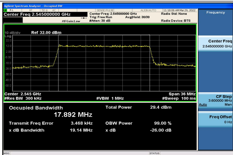
Band41-20MHz-16QAM-40140-100RB#0-17.892
