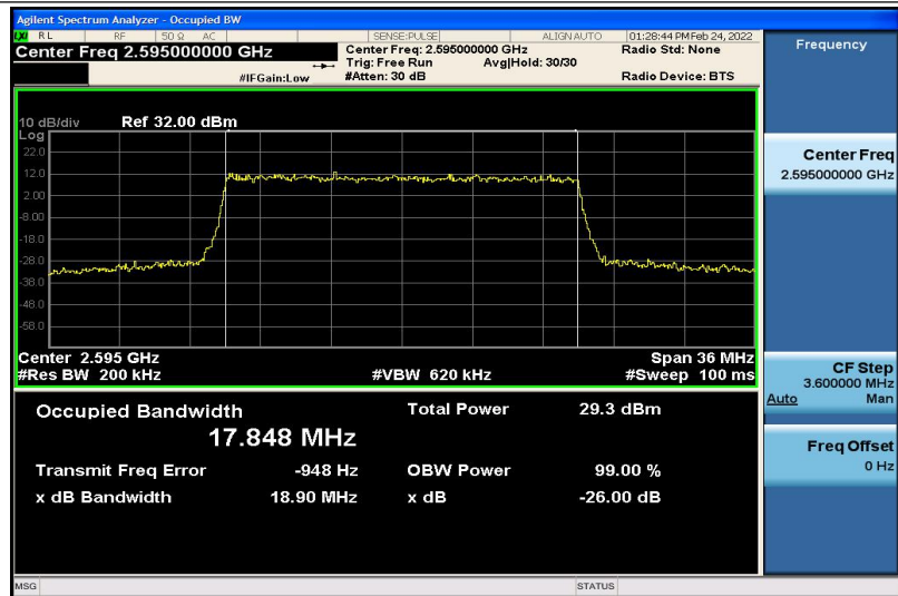
Band38-20MHz-QPSK-38000-100RB#0-17.848
