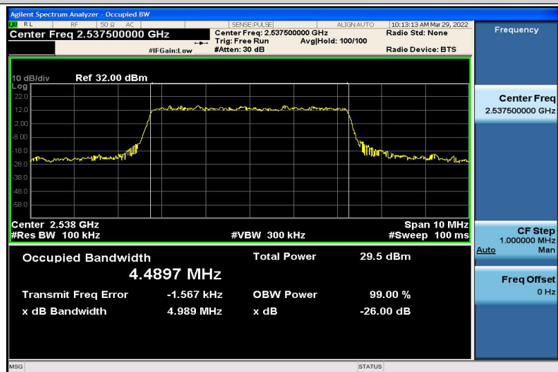
Band41-5MHz-QPSK-40065-25RB#0-4.4897
