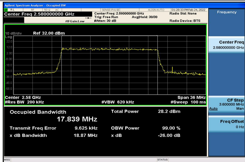
Band38-20MHz-16QAM-37850-100RB#0-17.839
