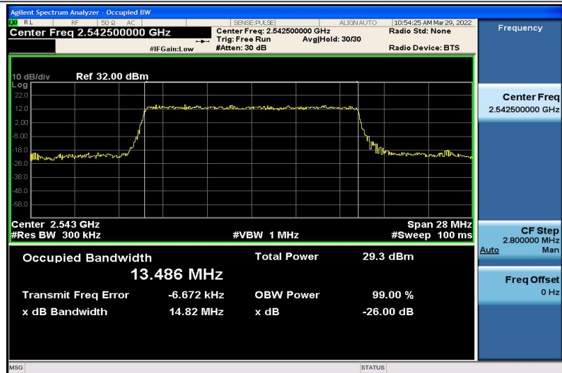
Band41-15MHz-16QAM-40115-75RB#0-13.486
