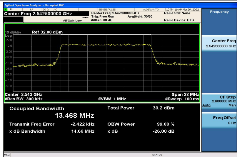
Band41-15MHz-QPSK-40115-75RB#0-13.468
