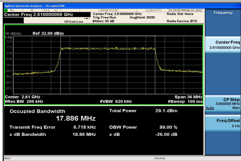
Band38-20MHz-QPSK-38150-100RB#0-17.886
