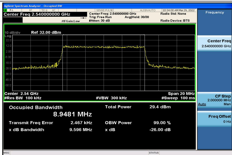
Band41-10MHz-QPSK-40090-50RB#0-8.9481
