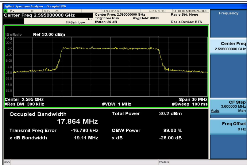
Band41-20MHz-QPSK-40640-100RB#0-17.864
