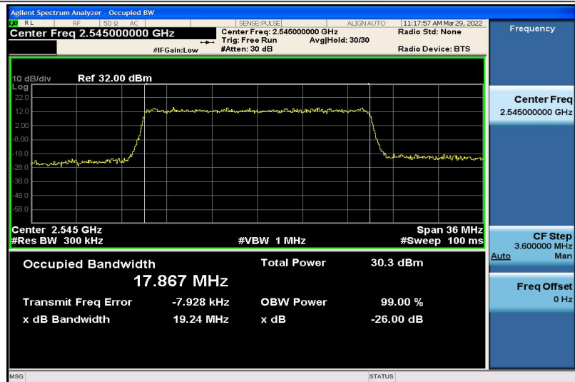
Band41-20MHz-QPSK-40140-100RB#0-17.867
