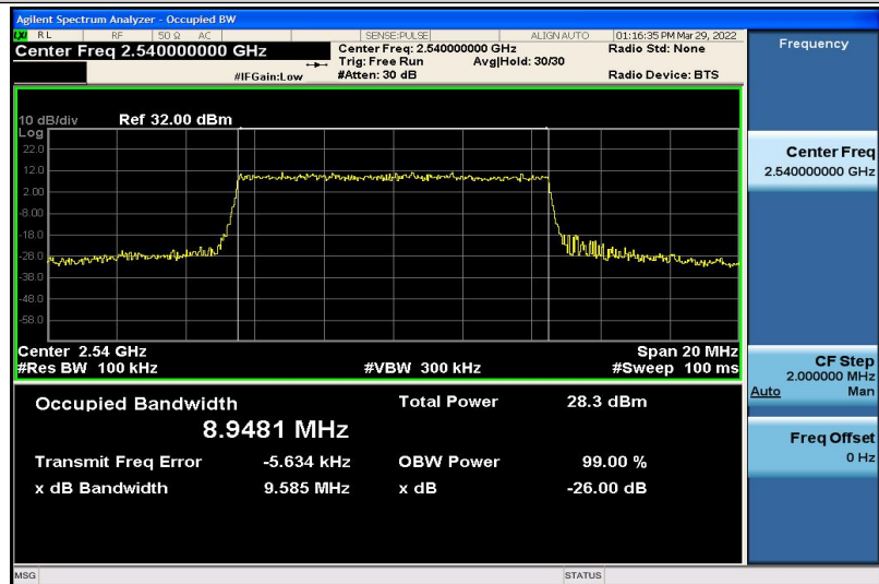
Band41-10MHz-16QAM-40090-50RB#0-8.9481
