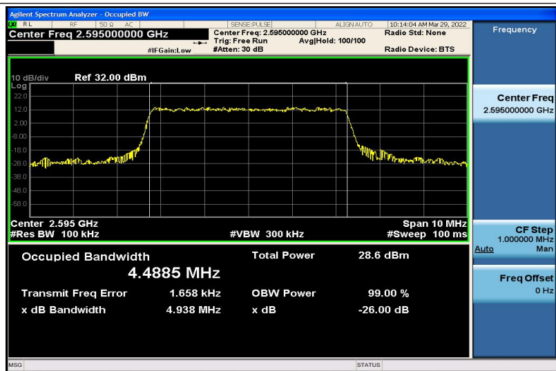
Band41-5MHz-16QAM-40640-25RB#0-4.4885
