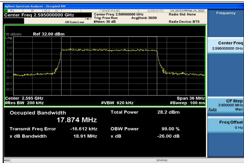
Band38-20MHz-16QAM-38000-100RB#0-17.874
