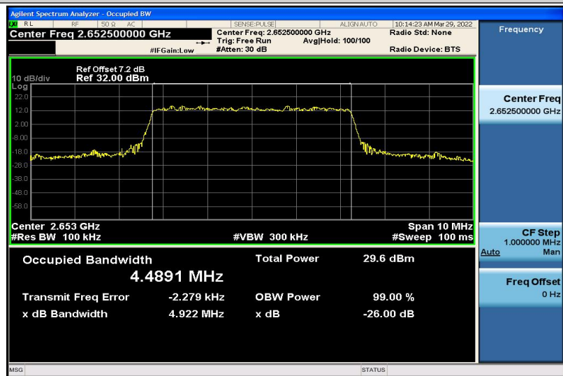
Band41-5MHz-QPSK-41215-25RB#0-4.4891
