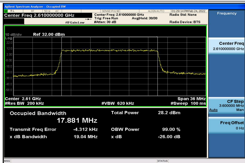
Band38-20MHz-16QAM-38150-100RB#0-17.881
