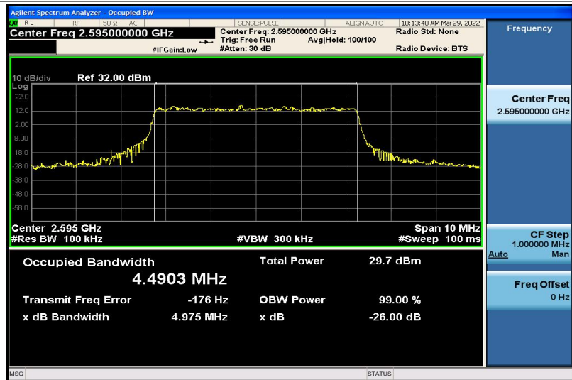
Band41-5MHz-QPSK-40640-25RB#0-4.4903
