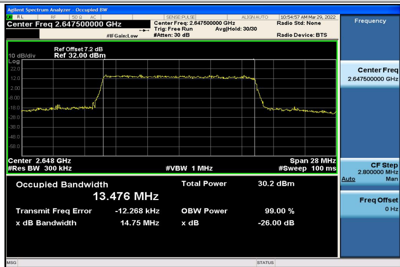
Band41-15MHz-QPSK-41165-75RB#0-13.476
