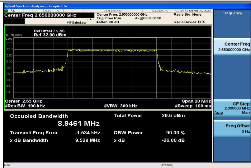
Band41-10MHz-QPSK-41190-50RB#0-8.9461
