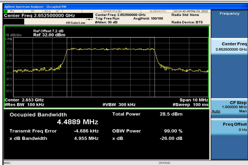
Band41-5MHz-16QAM-41215-25RB#0-4.4889
