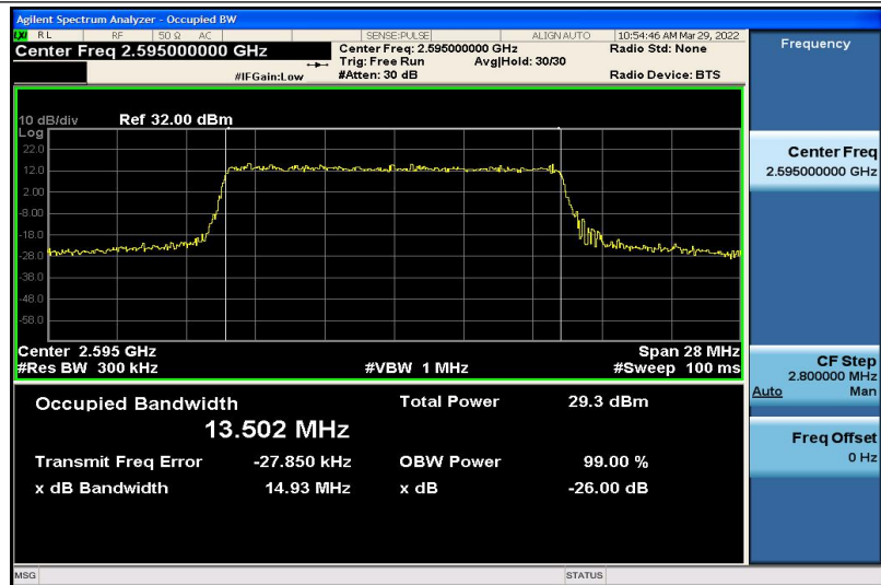
Band41-15MHz-16QAM-40640-75RB#0-13.502
