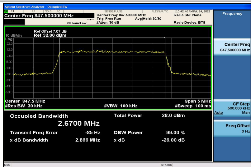
Band26-3MHz-16QAM-27025-15RB#0-2.6700
