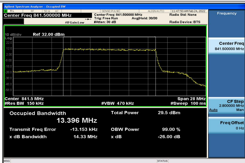
Band26-15MHz-16QAM-26965-75RB#0-13.396
