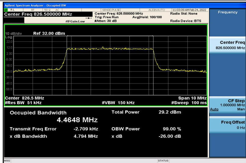
Band26-5MHz-16QAM-26815-25RB#0-4.4648
