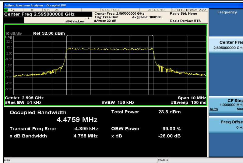
Band38-5MHz-QPSK-38000-25RB#0-4.4759
