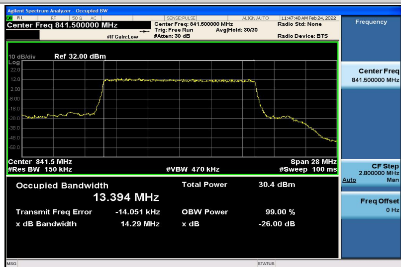
Band26-15MHz-QPSK-26965-75RB#0-13.394
