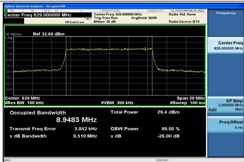
Band26-10MHz-16QAM-26840-50RB#0-8.9483
