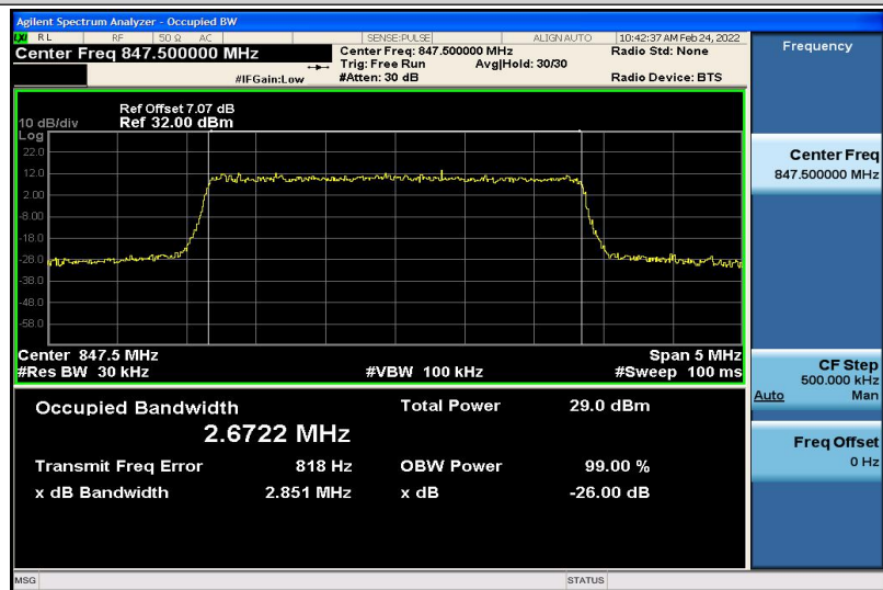
Band26-3MHz-QPSK-27025-15RB#0-2.6722
