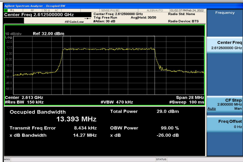
Band38-15MHz-QPSK-38175-75RB#0-13.393
