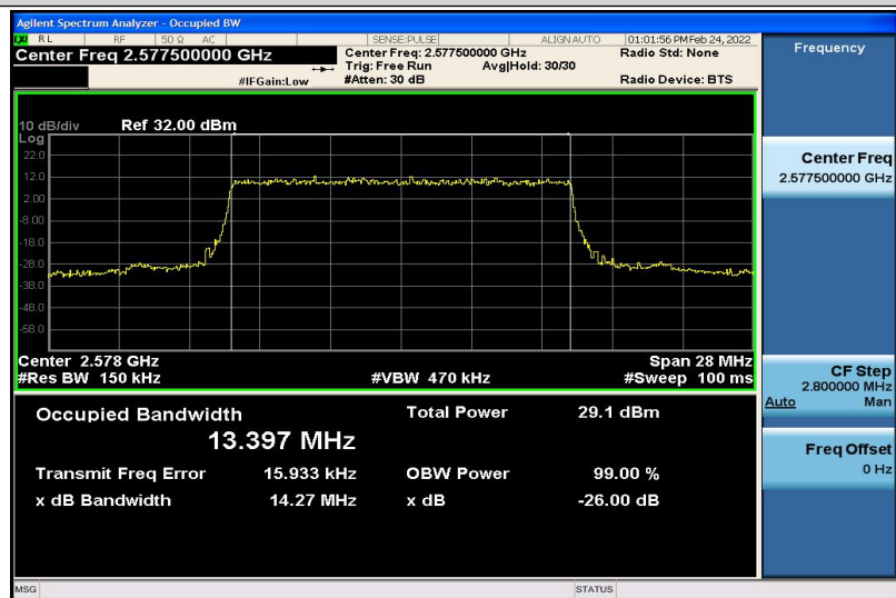
Band38-15MHz-QPSK-37825-75RB#0-13.397
