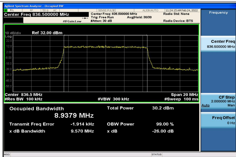
Band26-10MHz-QPSK-26915-50RB#0-8.9379
