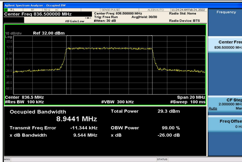
Band26-10MHz-16QAM-26915-50RB#0-8.9441
