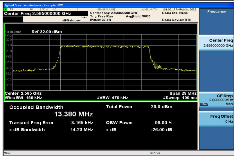
Band38-15MHz-QPSK-38000-75RB#0-13.380
