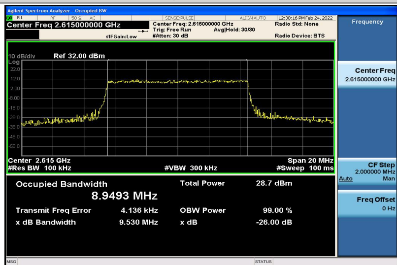
Band38-10MHz-QPSK-38200-50RB#0-8.9493
