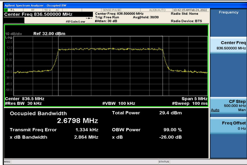
Band26-3MHz-QPSK-26915-15RB#0-2.6798
