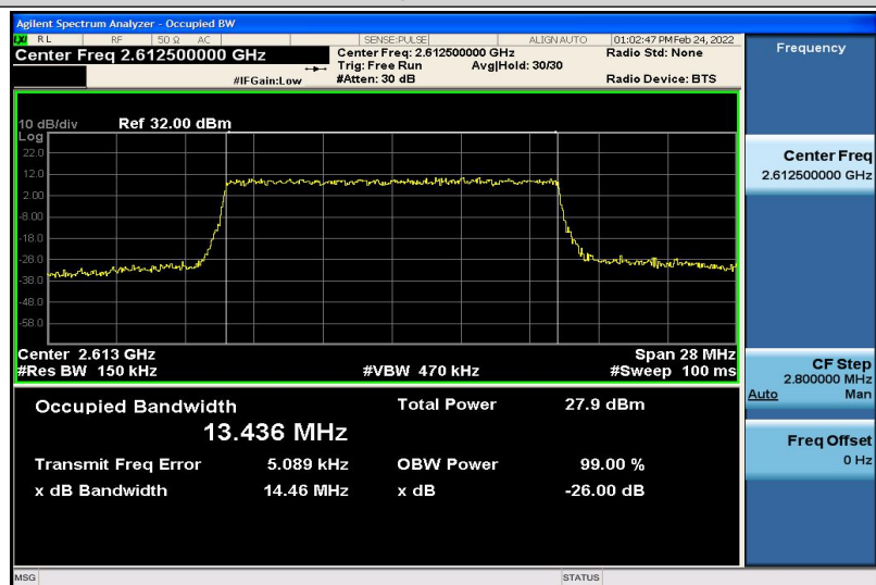
Band38-15MHz-16QAM-38175-75RB#0-13.436
