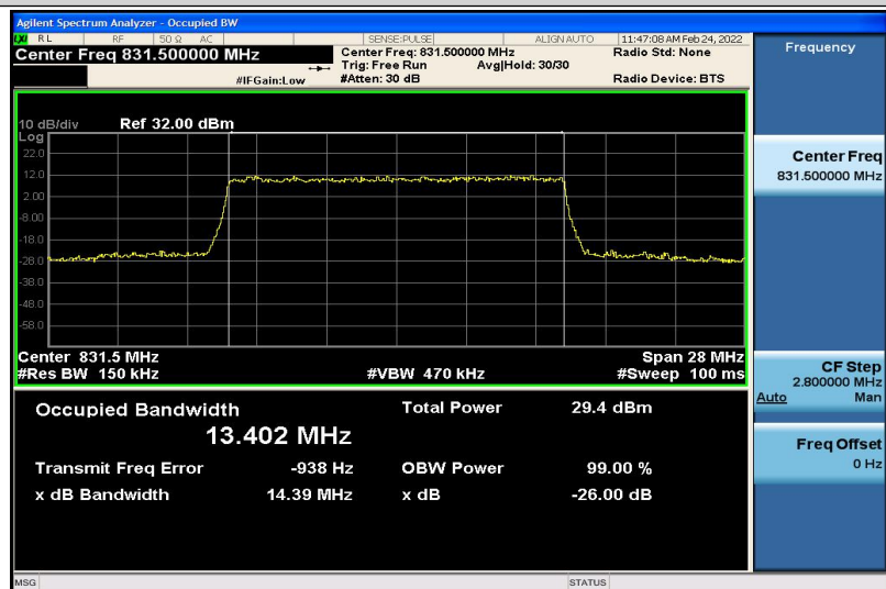
Band26-15MHz-16QAM-26865-75RB#0-13.402
