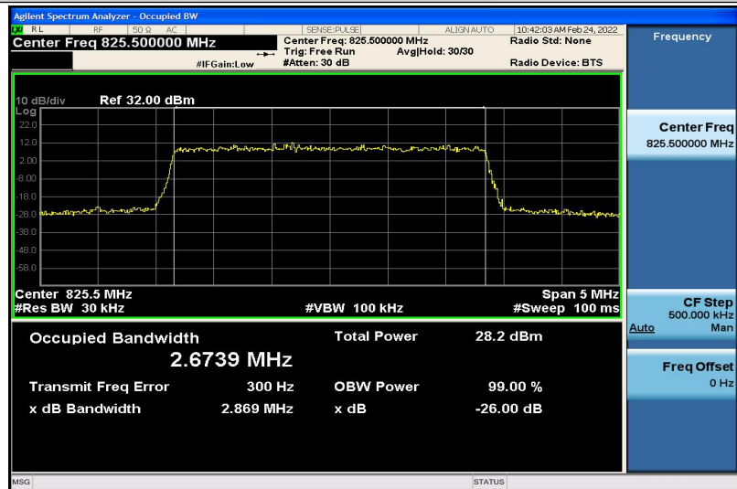
Band26-3MHz-16QAM-26805-15RB#0-2.6739
