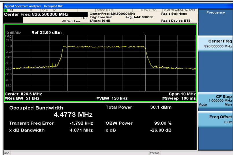
Band26-5MHz-QPSK-26815-25RB#0-4.4773
