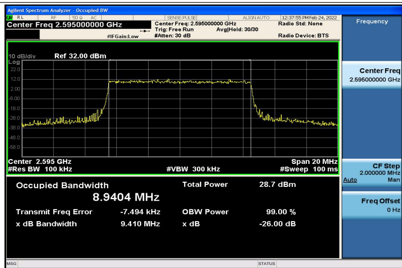
Band38-10MHz-QPSK-38000-50RB#0-8.9404
