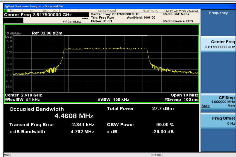
Band38-5MHz-16QAM-38225-25RB#0-4.4608
