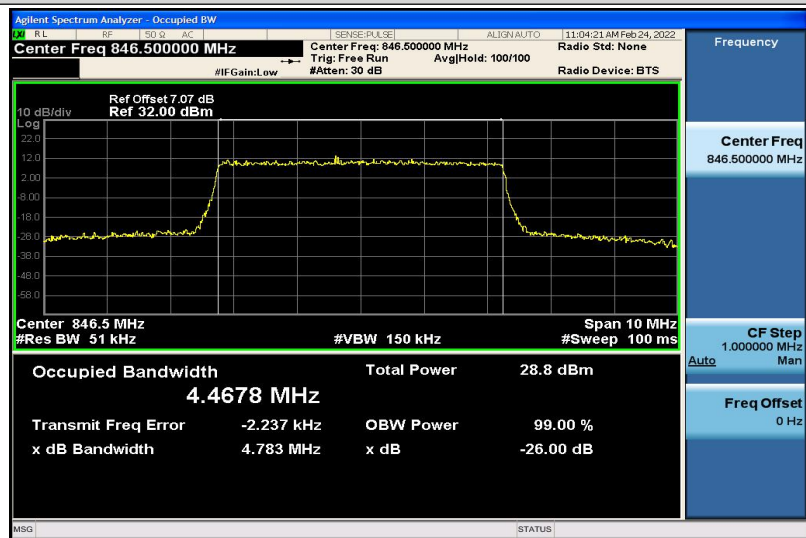
Band26-5MHz-16QAM-27015-25RB#0-4.4678
