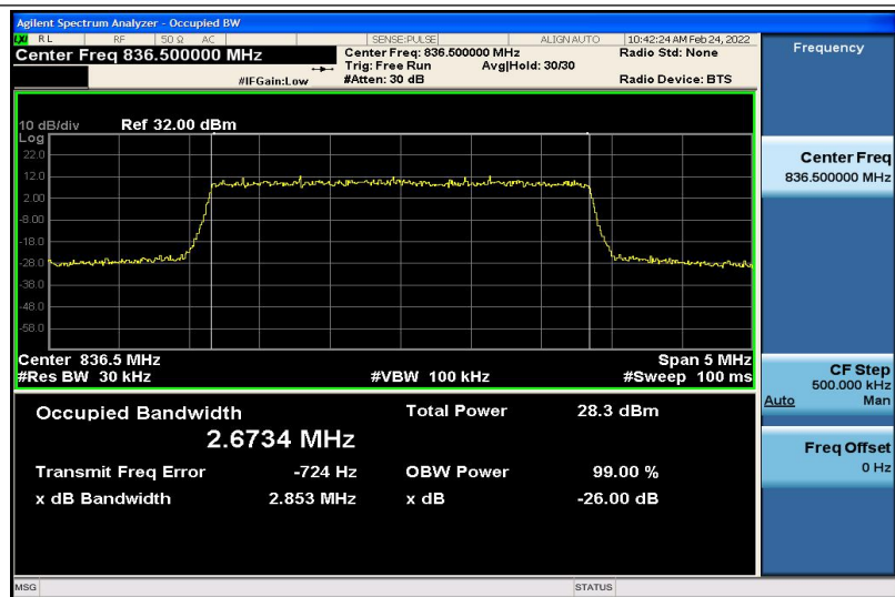
Band26-3MHz-16QAM-26915-15RB#0-2.6734
