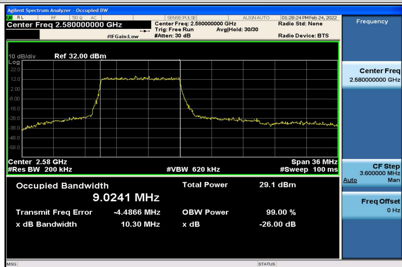
Band38-20MHz-QPSK-37850-100RB#0-9.0241
