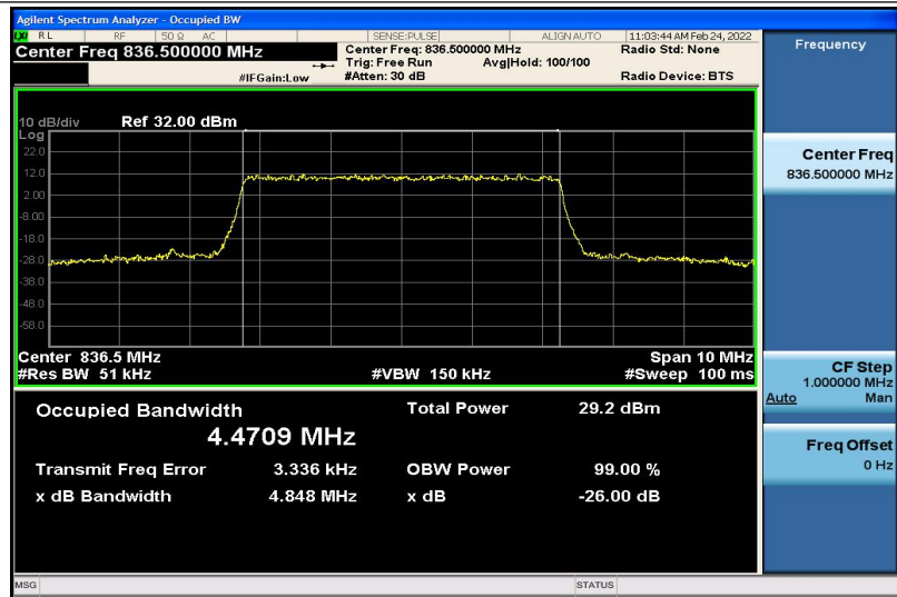
Band26-5MHz-16QAM-26915-25RB#0-4.4709
