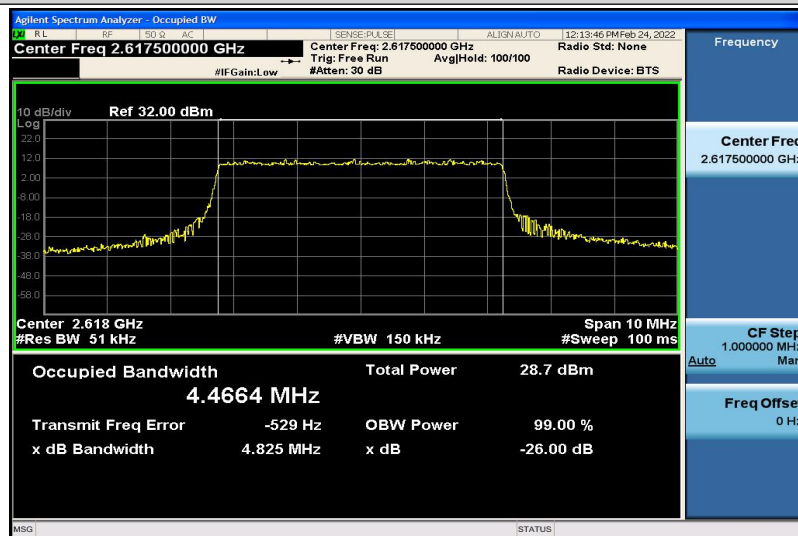
Band38-5MHz-QPSK-38225-25RB#0-4.4664
