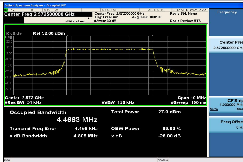
Band38-5MHz-16QAM-37775-25RB#0-4.4663
