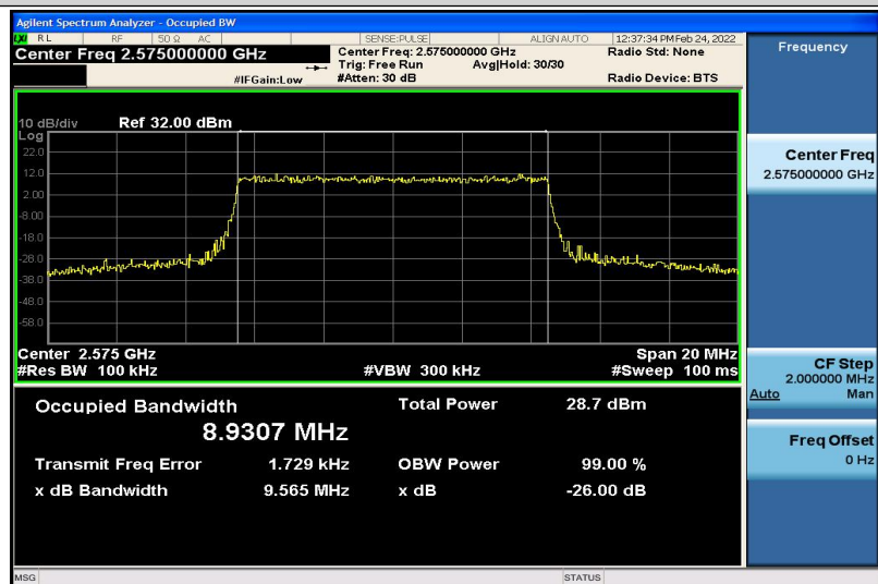
Band38-10MHz-QPSK-37800-50RB#0-8.9307
