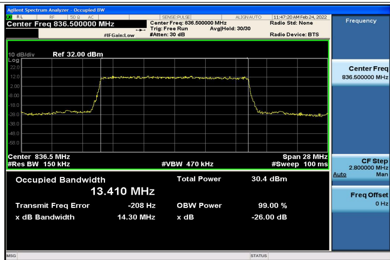
Band26-15MHz-QPSK-26915-75RB#0-13.410
