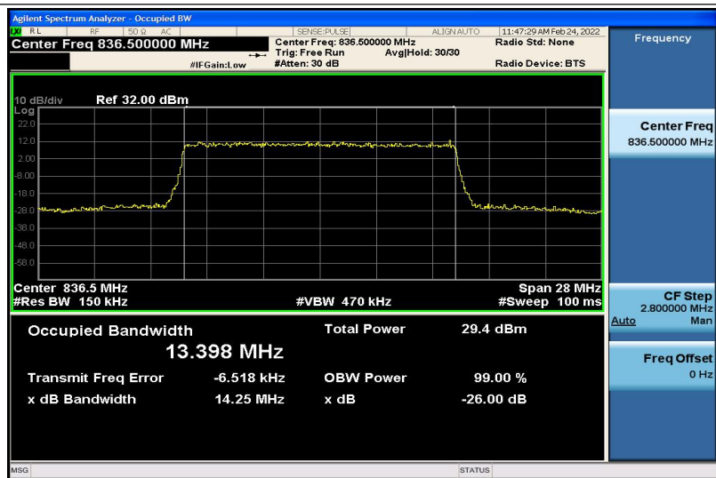
Band26-15MHz-16QAM-26915-75RB#0-13.398
