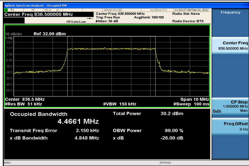
Band26-5MHz-QPSK-26915-25RB#0-4.4661
