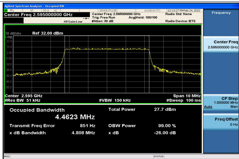
Band38-5MHz-16QAM-38000-25RB#0-4.4623
