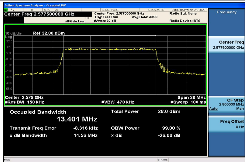
Band38-15MHz-16QAM-37825-75RB#0-13.401
