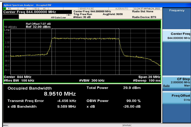
Band26-10MHz-QPSK-26990-50RB#0-8.9510
