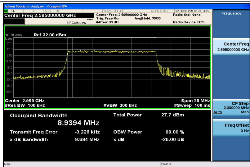
Band38-10MHz-16QAM-38000-50RB#0-8.9394
