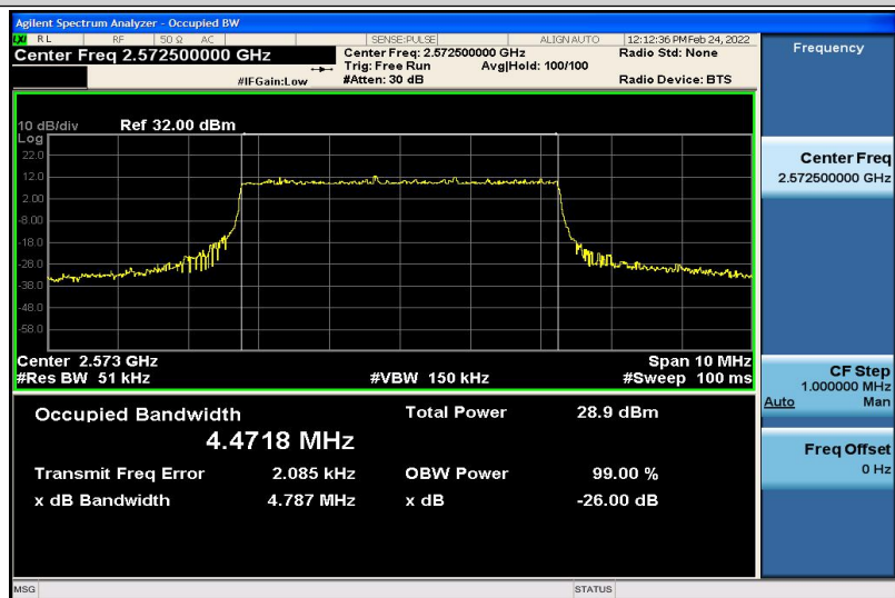
Band38-5MHz-QPSK-37775-25RB#0-4.4718
