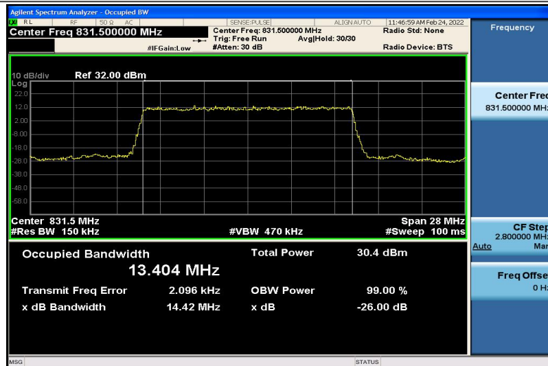
Band26-15MHz-QPSK-26865-75RB#0-13.404
