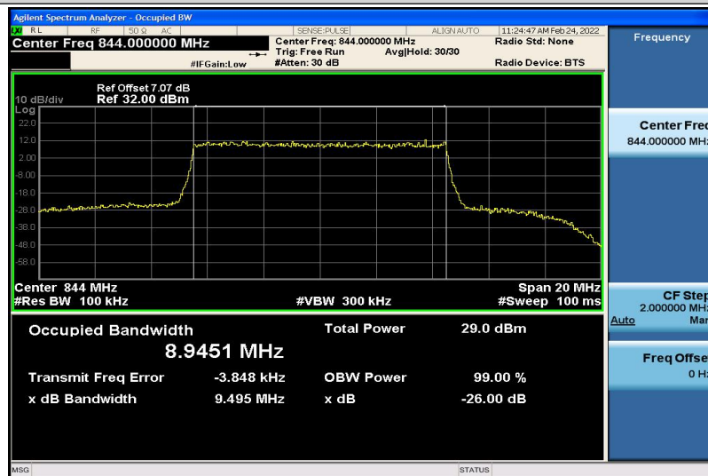
Band26-10MHz-16QAM-26990-50RB#0-8.9451
