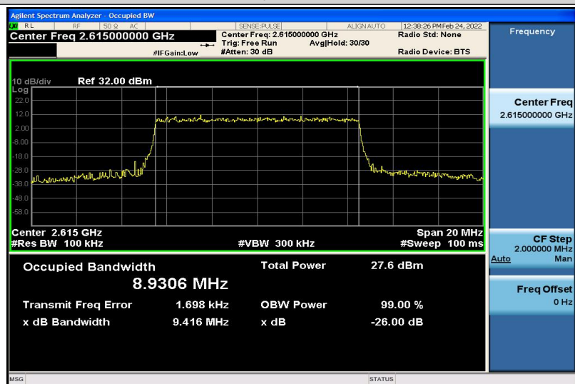
Band38-10MHz-16QAM-38200-50RB#0-8.9306
