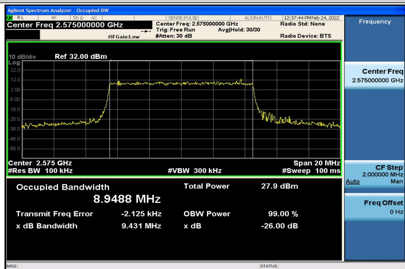
Band38-10MHz-16QAM-37800-50RB#0-8.9488
