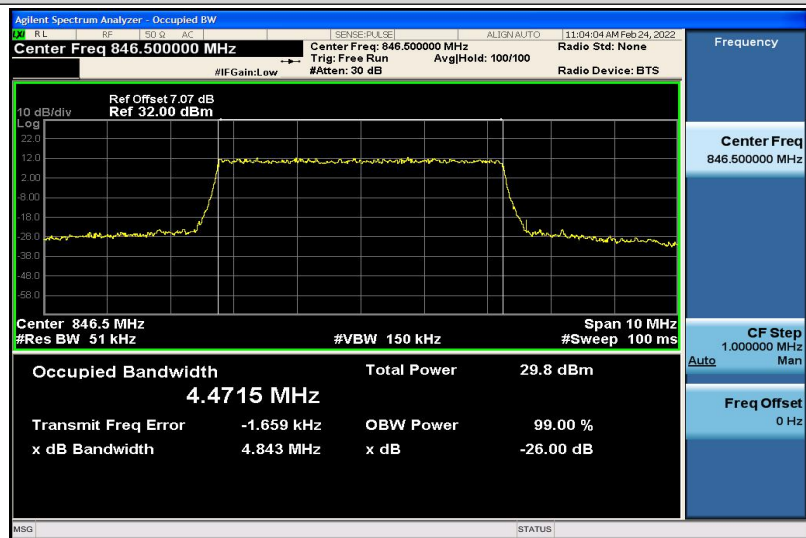
Band26-5MHz-QPSK-27015-25RB#0-4.4715
