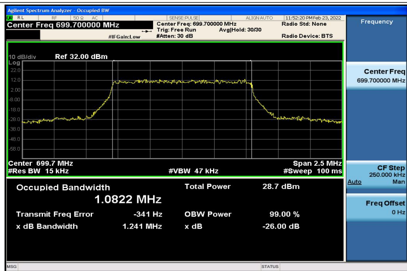
Band12-1.4MHz-QPSK-23017-6RB#0-1.0822
