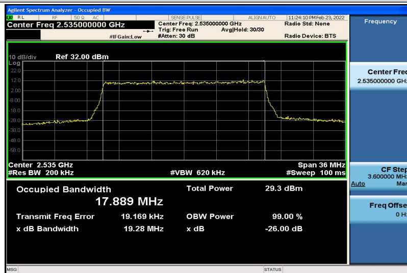
Band7-20MHz-QPSK-21100-100RB#0-17.889
