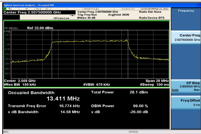
Band7-15MHz-16QAM-20825-75RB#0-13.411
