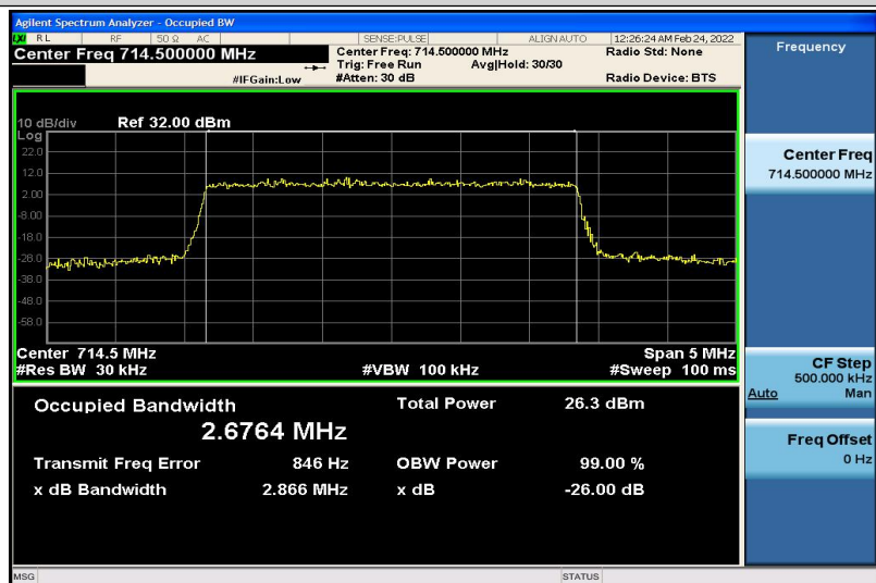
Band12-3MHz-16QAM-23165-15RB#0-2.6764
