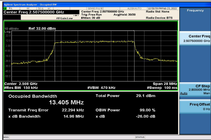
Band7-15MHz-QPSK-20825-75RB#0-13.405
