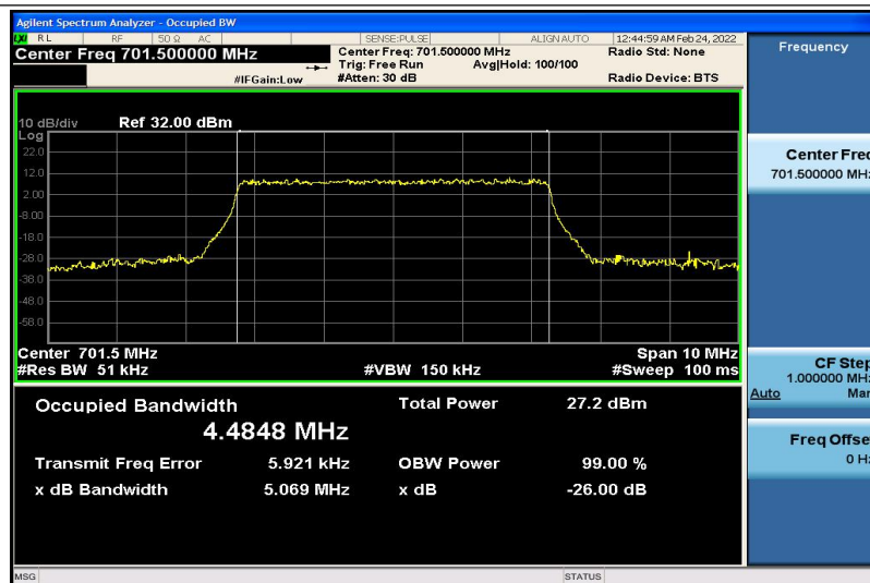
Band12-5MHz-16QAM-23035-25RB#0-4.4848
