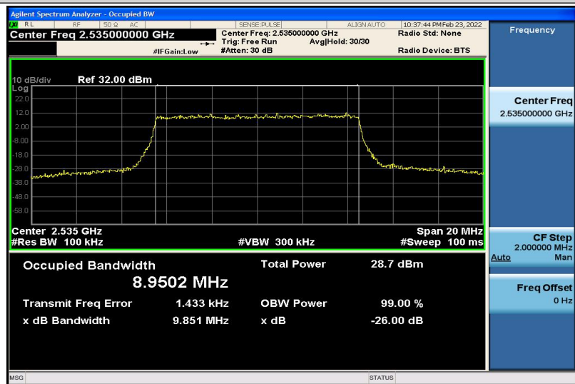
Band7-10MHz-QPSK-21100-50RB#0-8.9502
