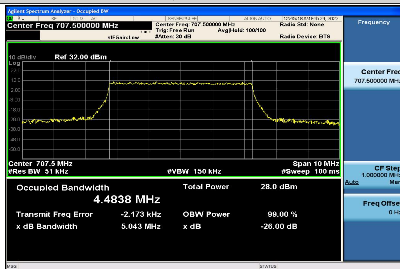
Band12-5MHz-QPSK-23095-25RB#0-4.4838
