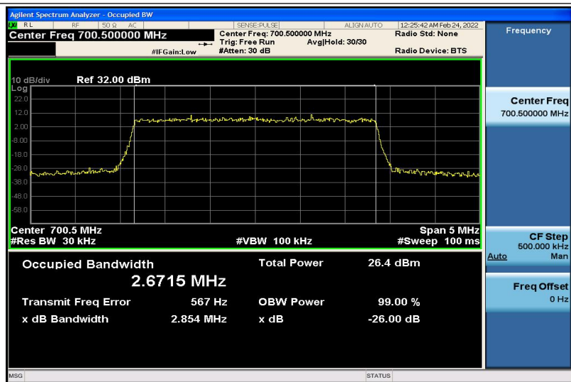
Band12-3MHz-16QAM-23025-15RB#0-2.6715
