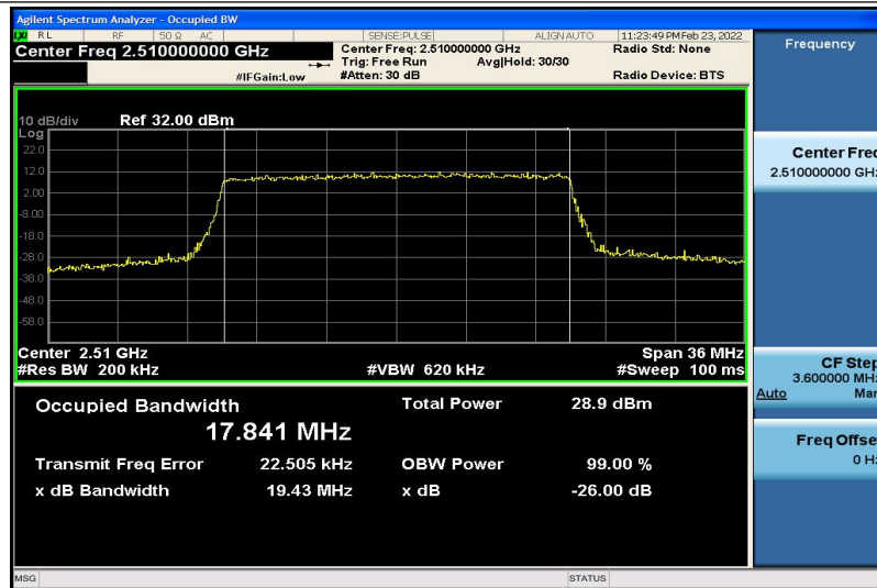
Band7-20MHz-QPSK-20850-100RB#0-17.841
