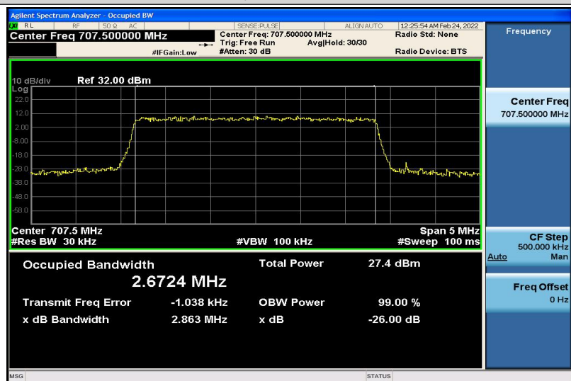
Band12-3MHz-QPSK-23095-15RB#0-2.6724
