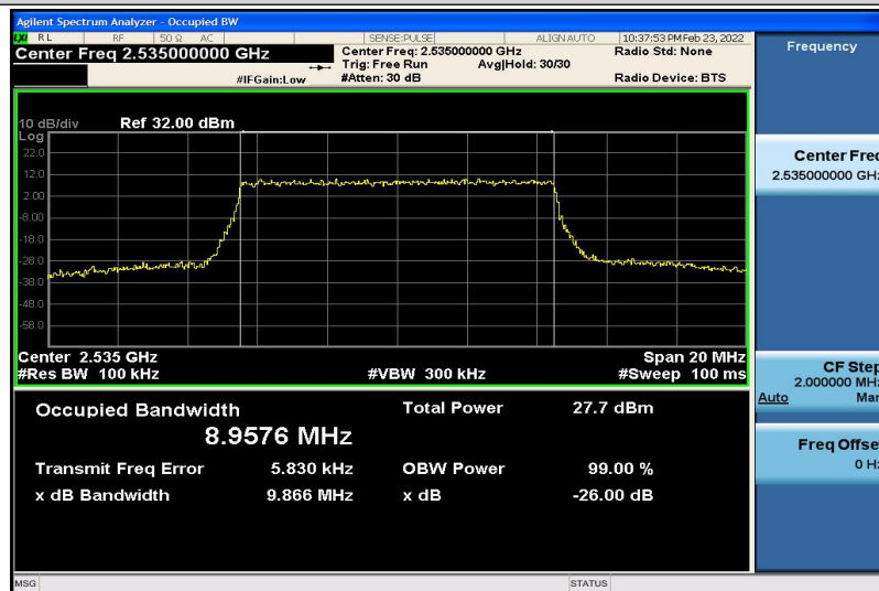
Band7-10MHz-16QAM-21100-50RB#0-8.9576
