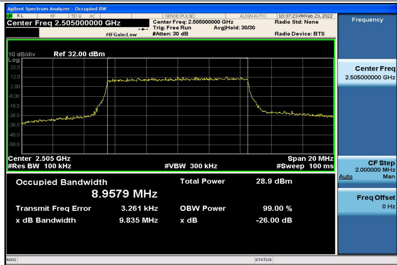
Band7-10MHz-QPSK-20800-50RB#0-8.9579
