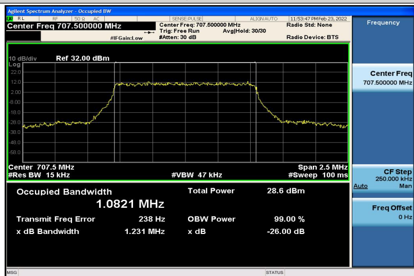
Band12-1.4MHz-QPSK-23095-6RB#0-1.0821
