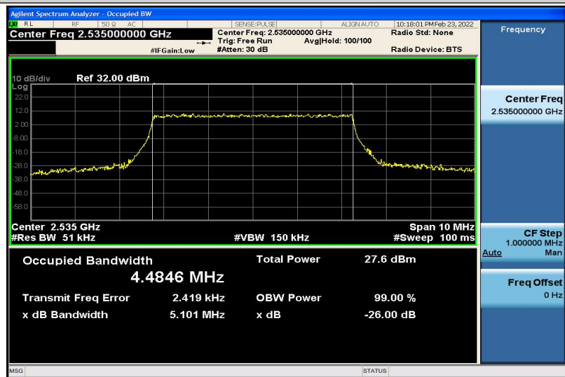
Band7-5MHz-16QAM-21100-25RB#0-4.4846
