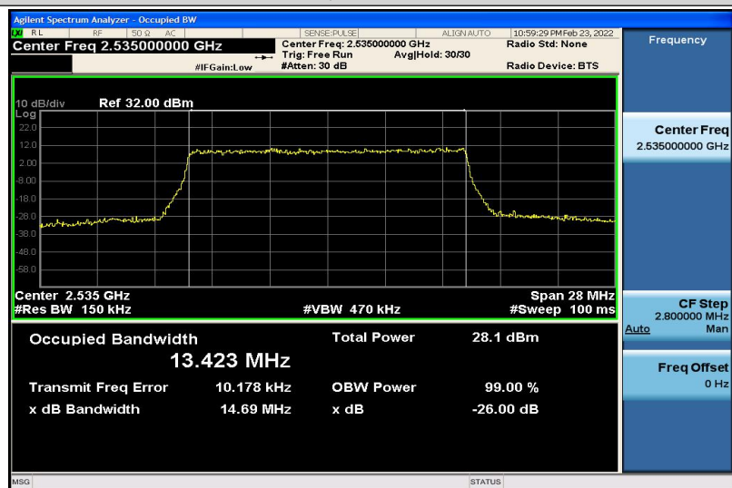
Band7-15MHz-16QAM-21100-75RB#0-13.423
