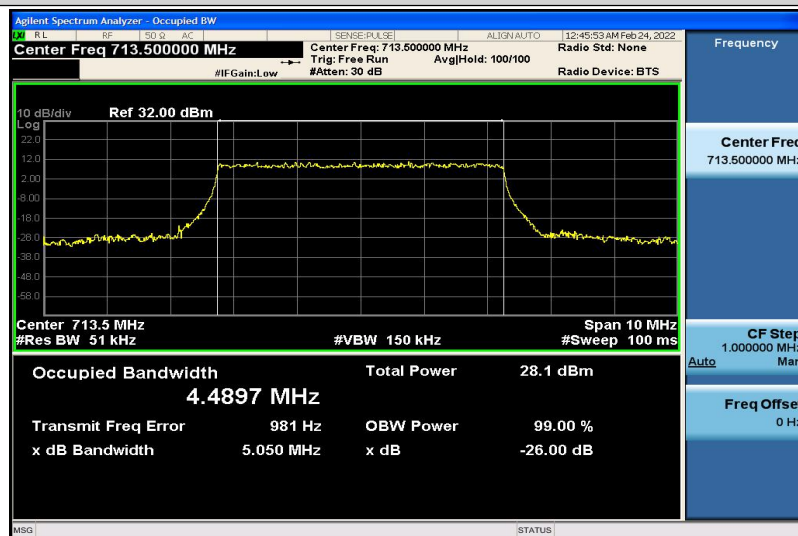
Band12-5MHz-QPSK-23155-25RB#0-4.4897
