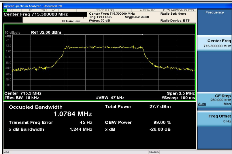
Band12-1.4MHz-16QAM-23173-6RB#0-1.0784
