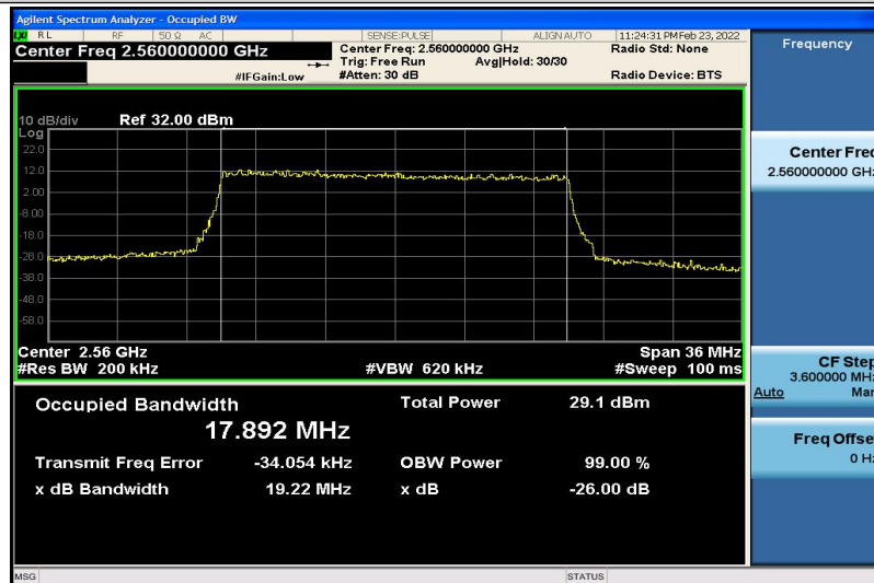
Band7-20MHz-QPSK-21350-100RB#0-17.892
