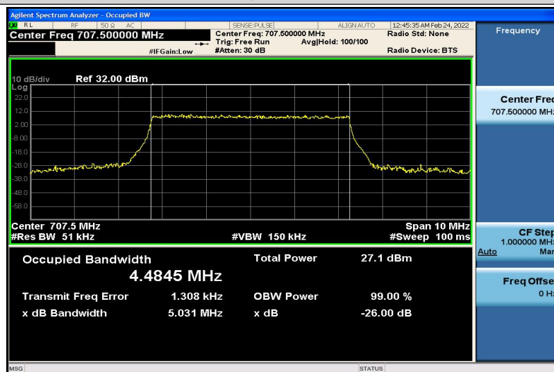
Band12-5MHz-16QAM-23095-25RB#0-4.4845
