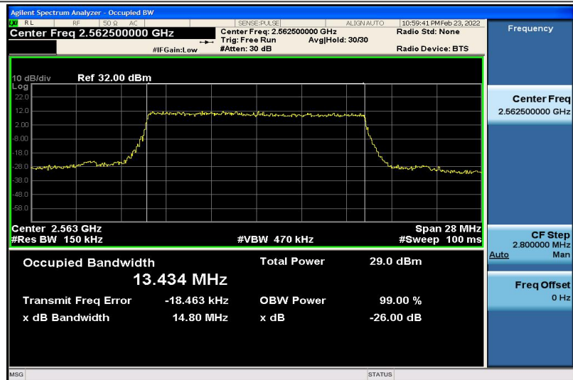
Band7-15MHz-QPSK-21375-75RB#0-13.434
