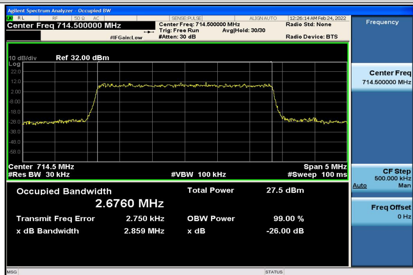
Band12-3MHz-QPSK-23165-15RB#0-2.6760
