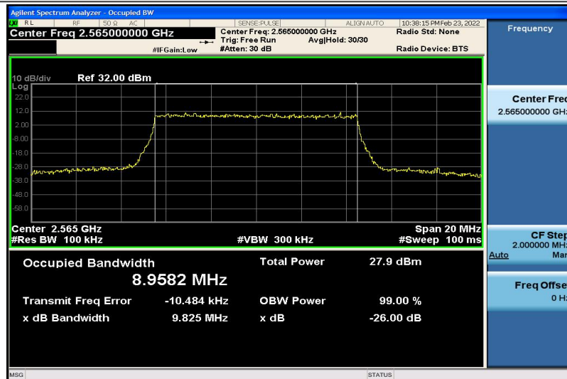
Band7-10MHz-16QAM-21400-50RB#0-8.9582
