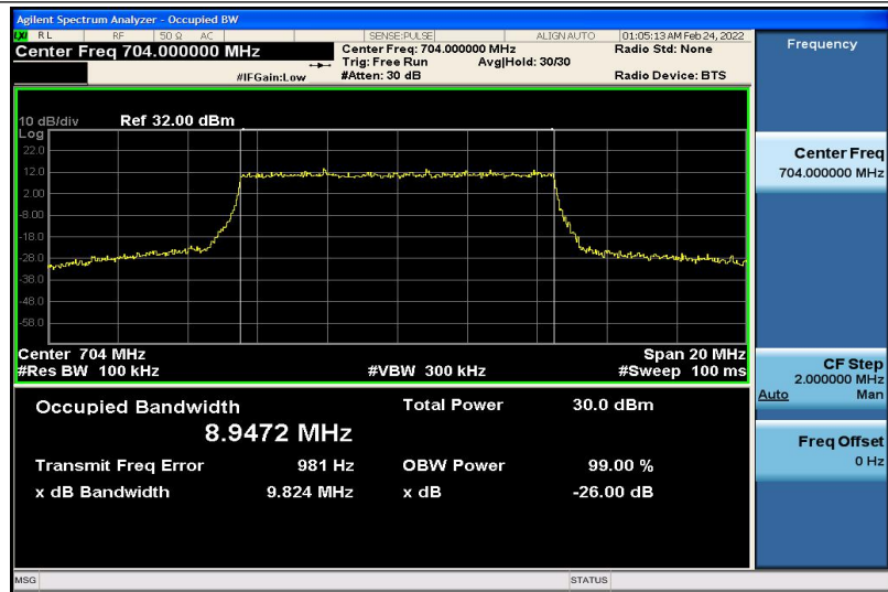
Band12-10MHz-QPSK-23060-50RB#0-8.9472
