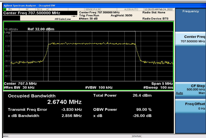
Band12-3MHz-16QAM-23095-15RB#0-2.6740
