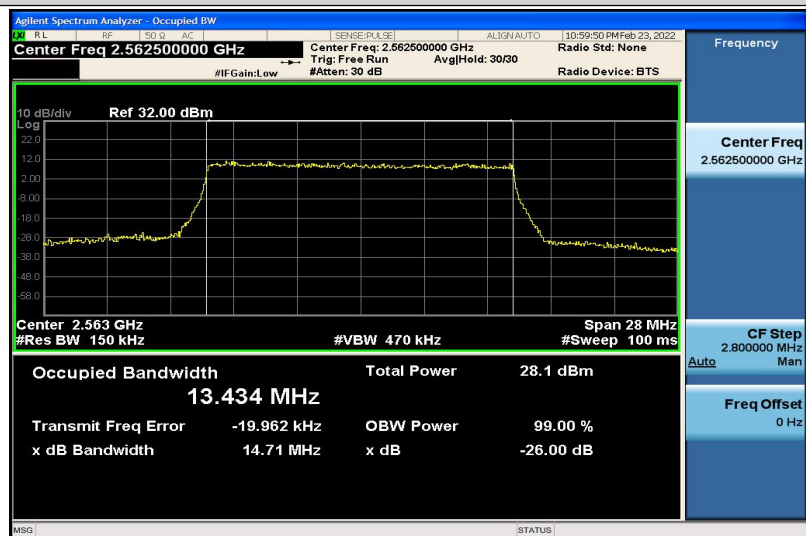
Band7-15MHz-16QAM-21375-75RB#0-13.434
