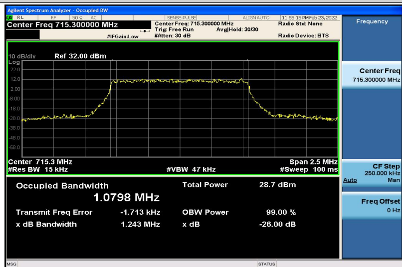
Band12-1.4MHz-QPSK-23173-6RB#0-1.0798
