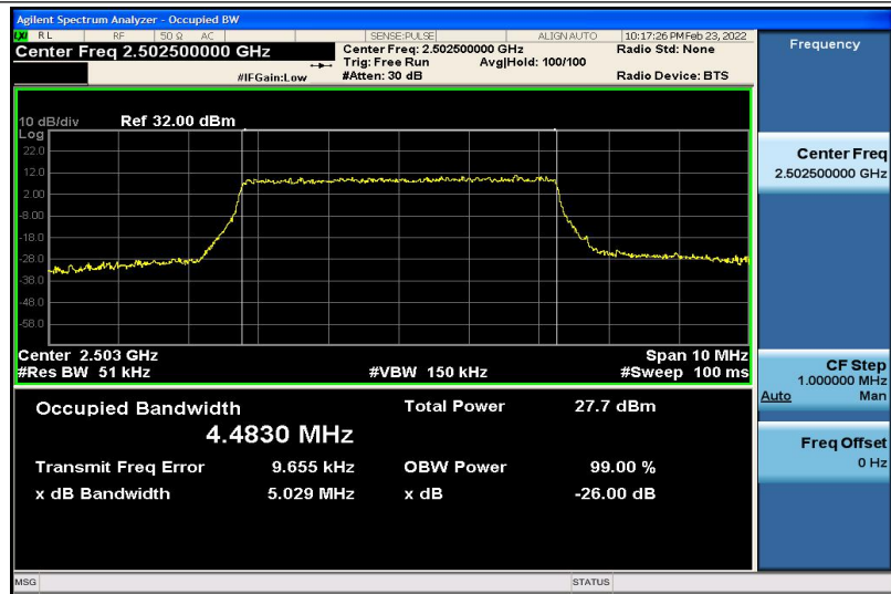
Band7-5MHz-16QAM-20775-25RB#0-4.4830
