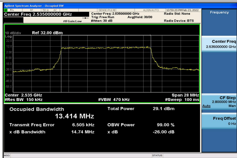
Band7-15MHz-QPSK-21100-75RB#0-13.414
