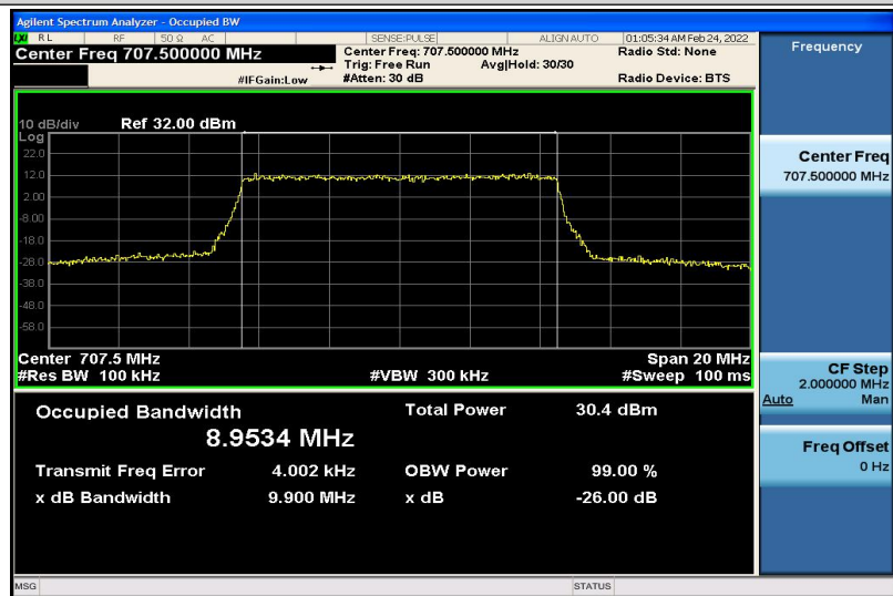
Band12-10MHz-QPSK-23095-50RB#0-8.9534
