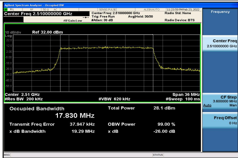
Band7-20MHz-16QAM-20850-100RB#0-17.830
