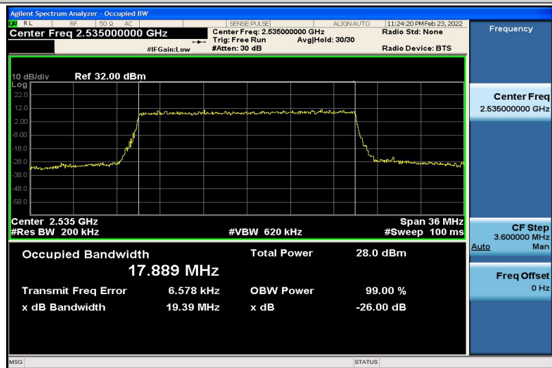
Band7-20MHz-16QAM-21100-100RB#0-17.889
