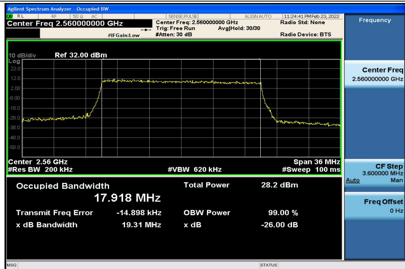
Band7-20MHz-16QAM-21350-100RB#0-17.918
