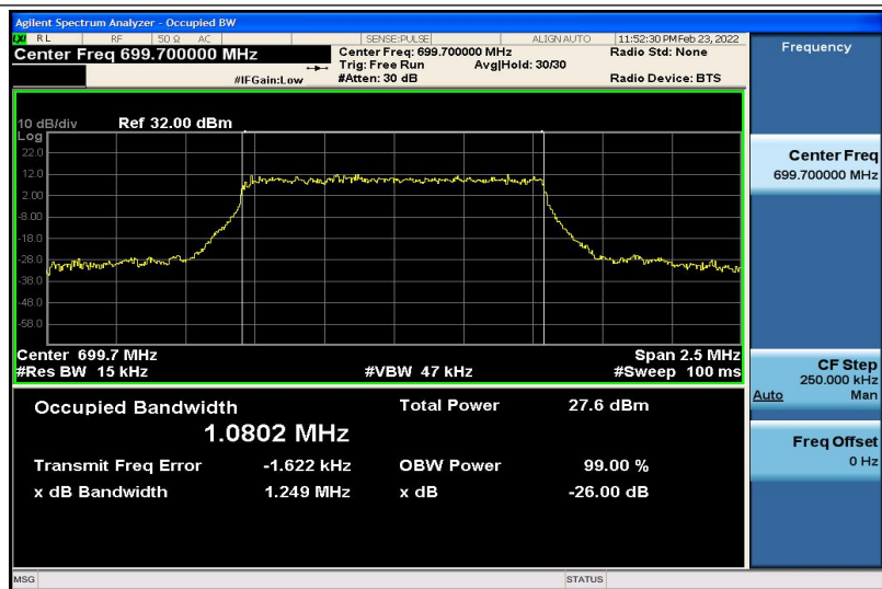
Band12-1.4MHz-16QAM-23017-6RB#0-1.0802
