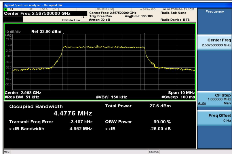
Band7-5MHz-16QAM-21425-25RB#0-4.4776
