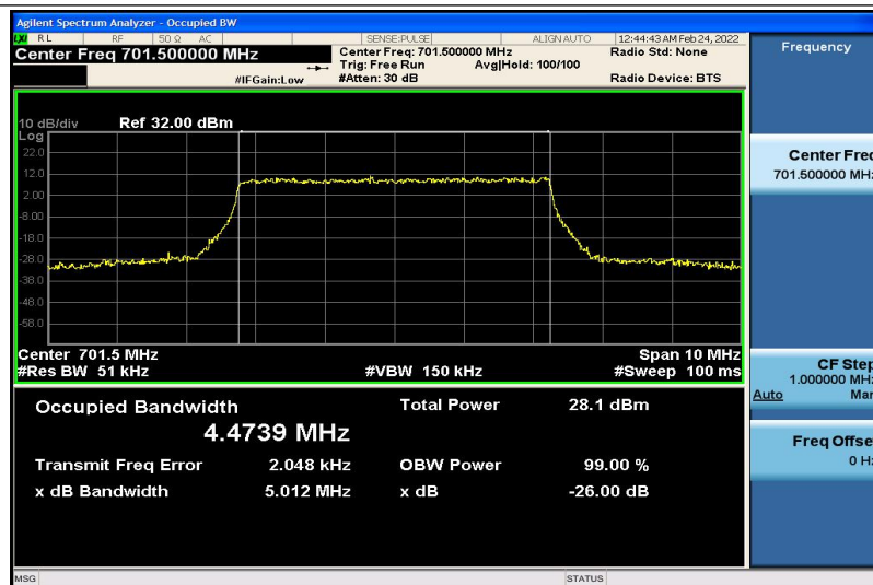
Band12-5MHz-QPSK-23035-25RB#0-4.4739
