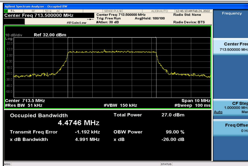
Band12-5MHz-16QAM-23155-25RB#0-4.4746
