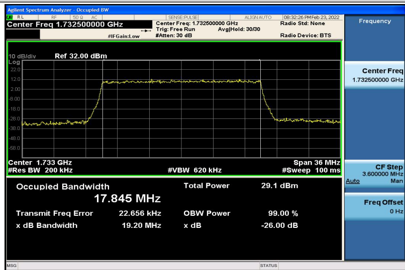
Band4-20MHz-QPSK-20175-100RB#0-17.845
