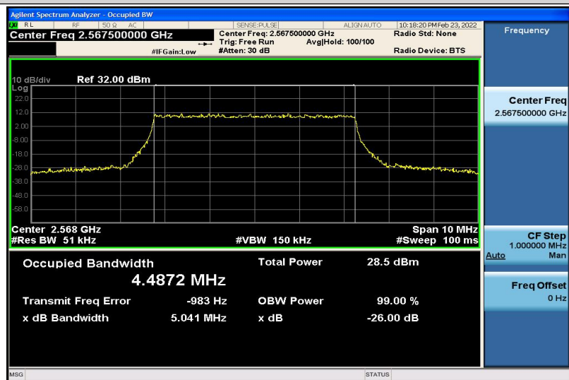
Band7-5MHz-QPSK-21425-25RB#0-4.4872
