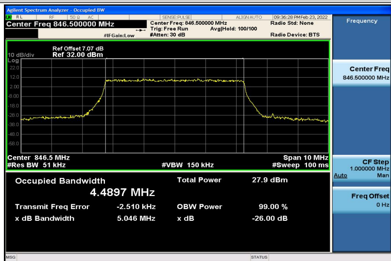
Band5-5MHz-QPSK-20625-25RB#0-4.4897
