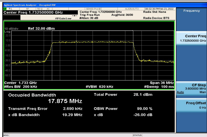
Band4-20MHz-16QAM-20175-100RB#0-17.875
