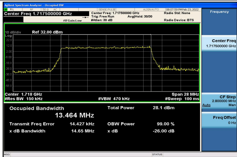
Band4-15MHz-16QAM-20025-75RB#0-13.464
