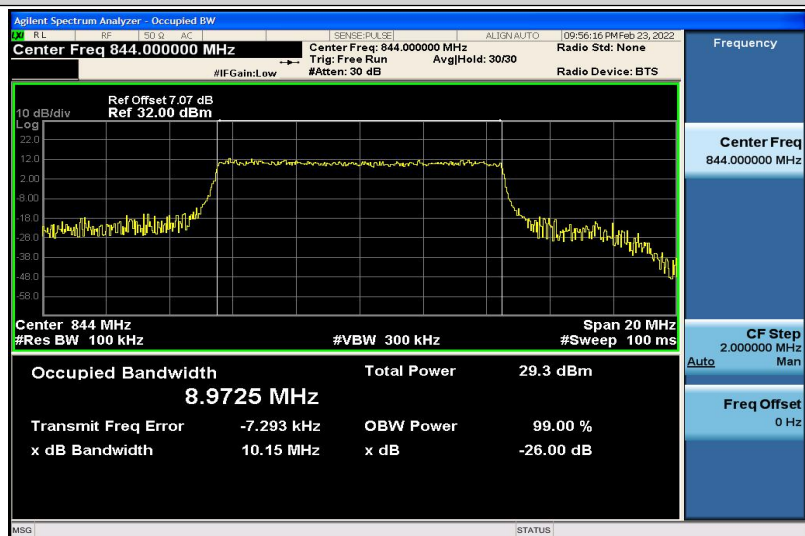
Band5-10MHz-QPSK-20600-50RB#0-8.9725
