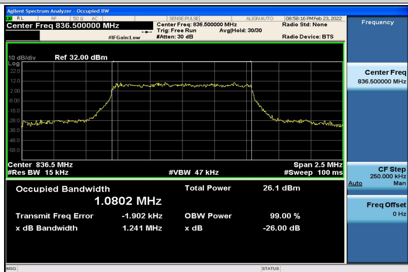
Band5-1.4MHz-16QAM-20525-6RB#0-1.0802
