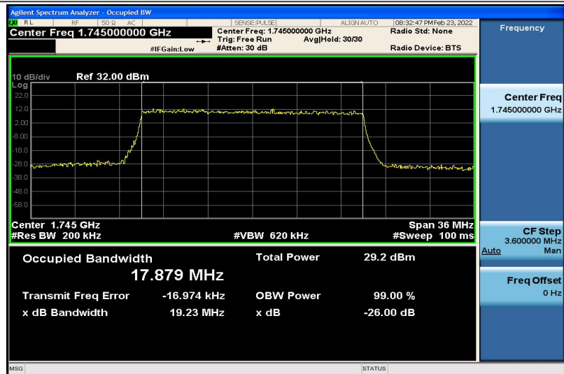
Band4-20MHz-QPSK-20300-100RB#0-17.879
