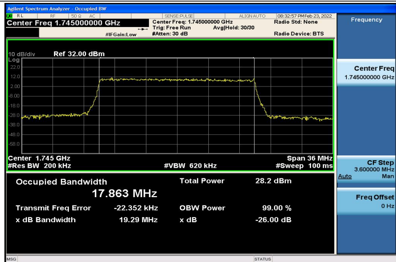
Band4-20MHz-16QAM-20300-100RB#0-17.863
