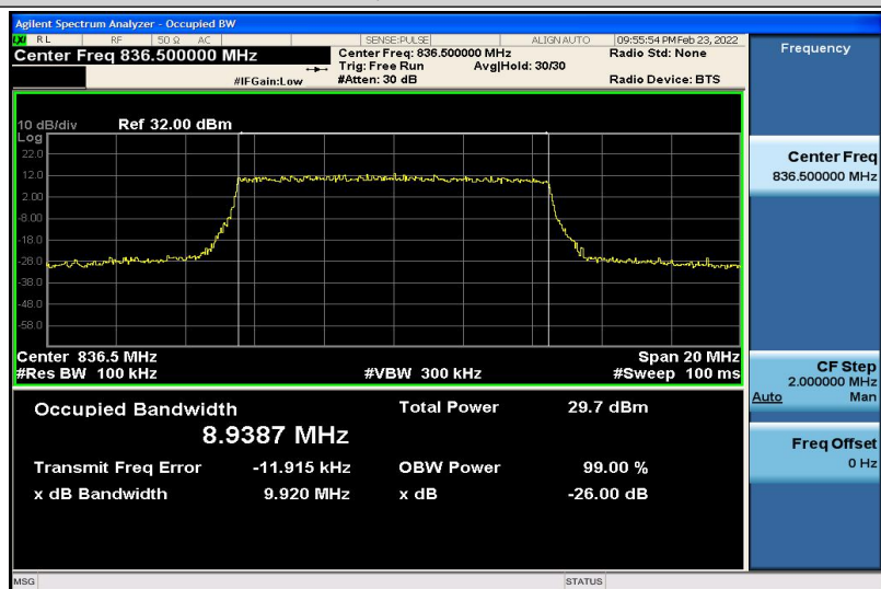
Band5-10MHz-QPSK-20525-50RB#0-8.9387
