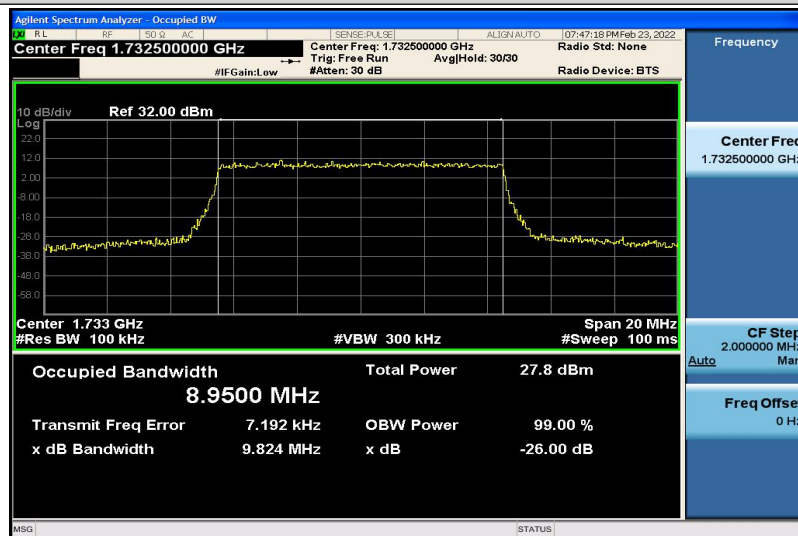
Band4-10MHz-16QAM-20175-50RB#0-8.9500
