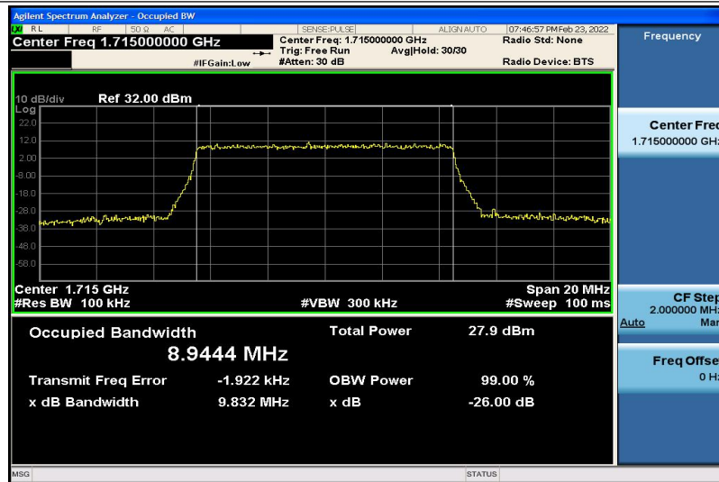
Band4-10MHz-16QAM-20000-50RB#0-8.9444
