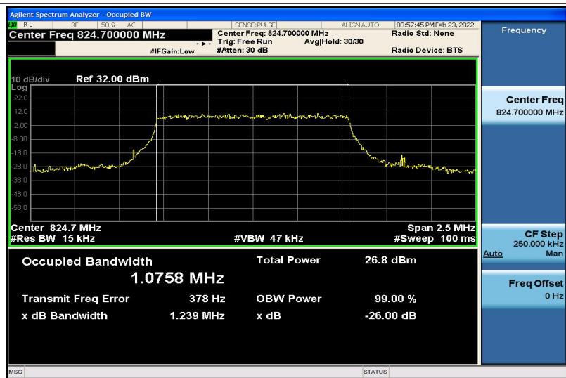
Band5-1.4MHz-QPSK-20407-6RB#0-1.0758
