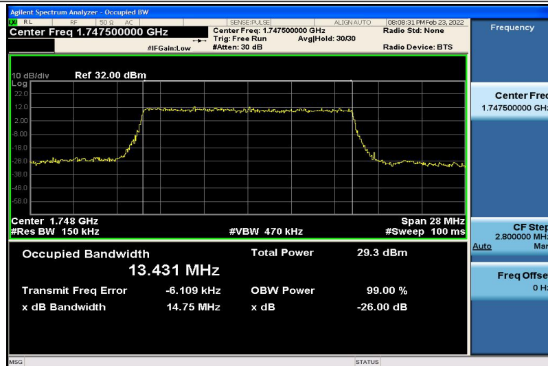
Band4-15MHz-QPSK-20325-75RB#0-13.431
