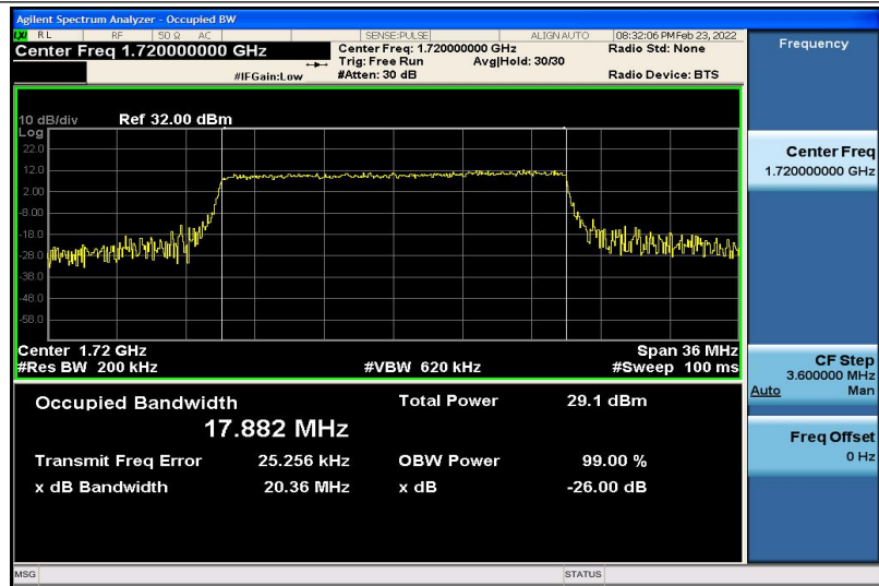
Band4-20MHz-QPSK-20050-100RB#0-17.882
