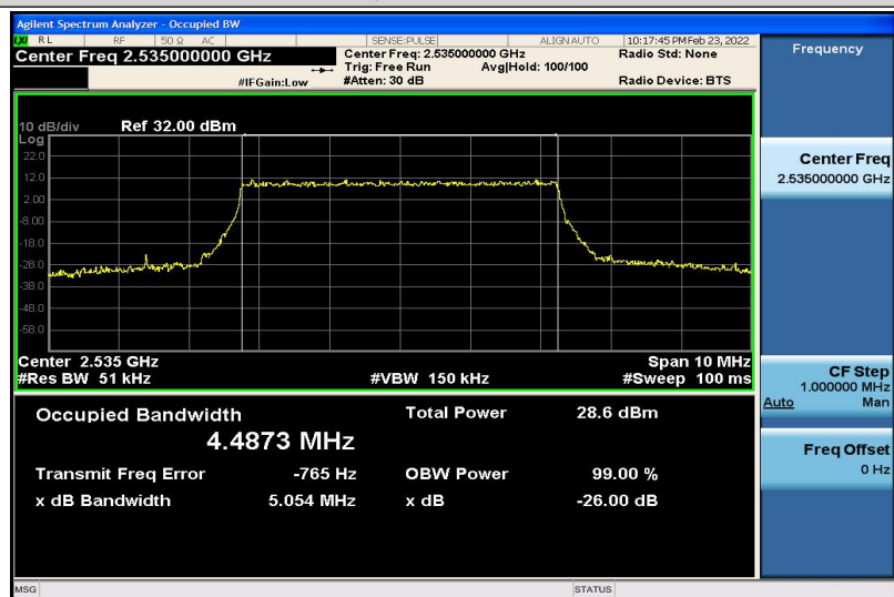
Band7-5MHz-QPSK-21100-25RB#0-4.4873
