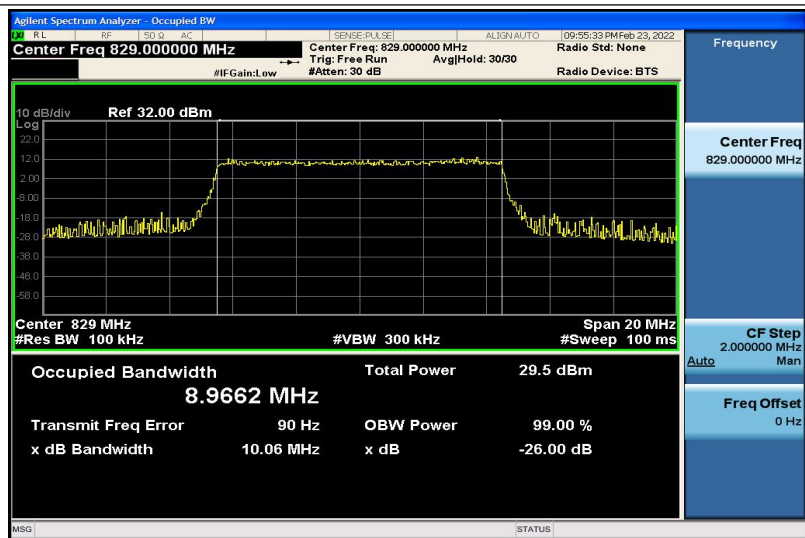
Band5-10MHz-QPSK-20450-50RB#0-8.9662
