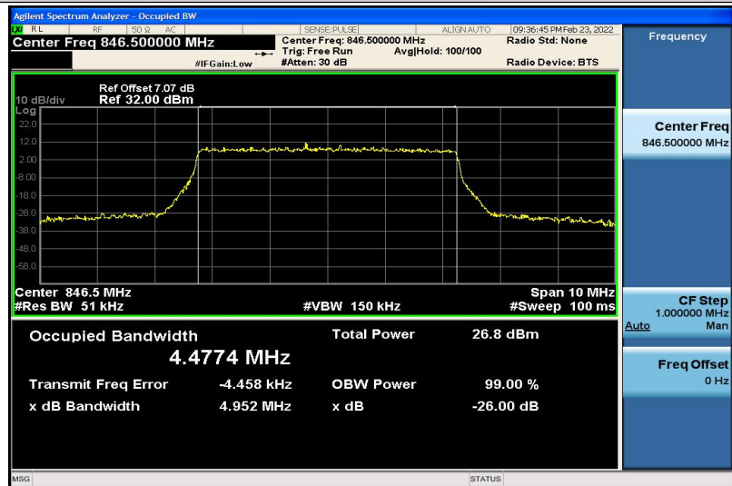
Band5-5MHz-16QAM-20625-25RB#0-4.4774
