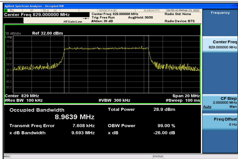
Band5-10MHz-16QAM-20450-50RB#0-8.9639
