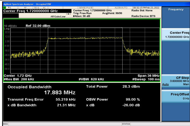
Band4-20MHz-16QAM-20050-100RB#0-17.883
