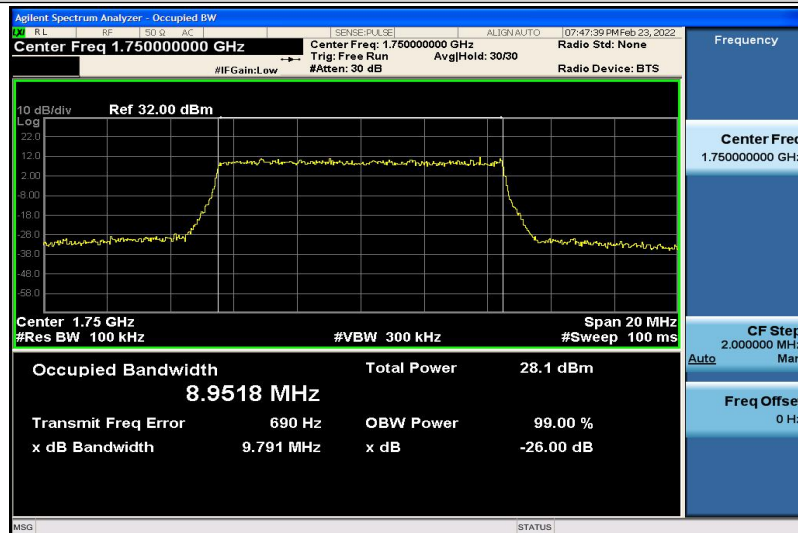
Band4-10MHz-16QAM-20350-50RB#0-8.9518
