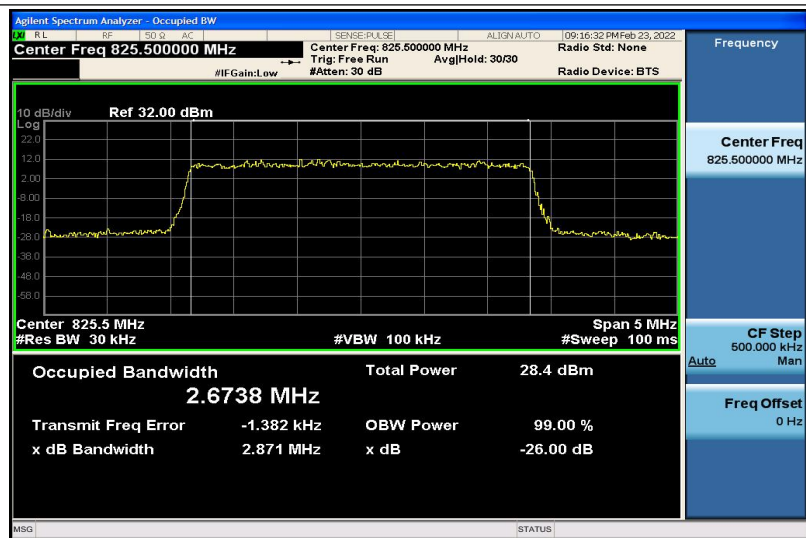
Band5-3MHz-16QAM-20415-15RB#0-2.6738
