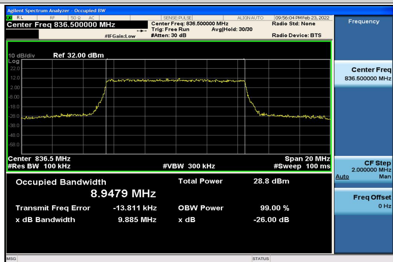
Band5-10MHz-16QAM-20525-50RB#0-8.9479
