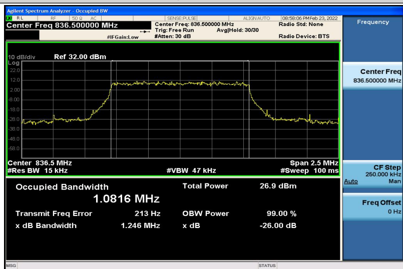
Band5-1.4MHz-QPSK-20525-6RB#0-1.0816
