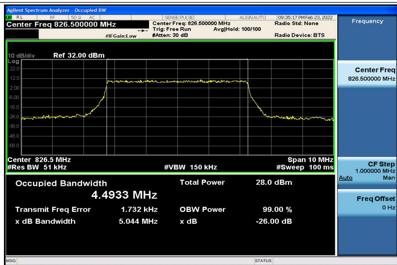
Band5-5MHz-QPSK-20425-25RB#0-4.4933
