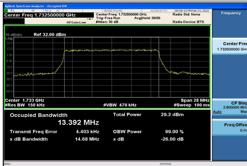
Band4-15MHz-QPSK-20175-75RB#0-13.392
