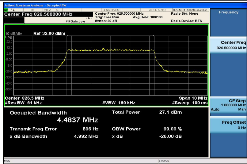
Band5-5MHz-16QAM-20425-25RB#0-4.4837
