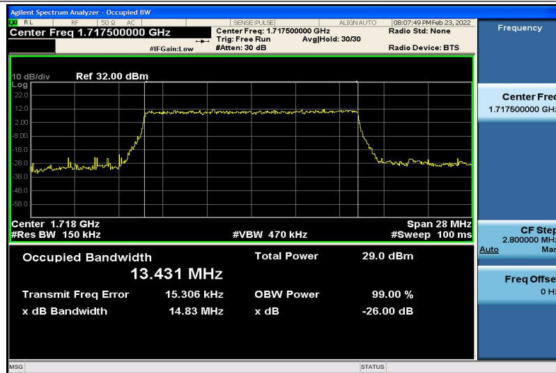
Band4-15MHz-QPSK-20025-75RB#0-13.431
