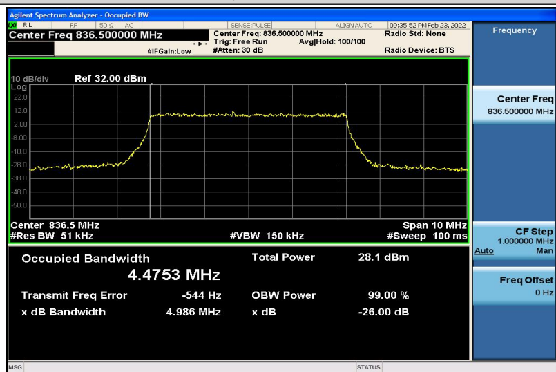
Band5-5MHz-QPSK-20525-25RB#0-4.4753
