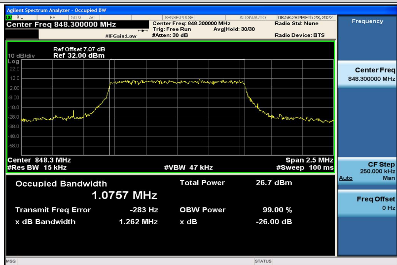
Band5-1.4MHz-QPSK-20643-6RB#0-1.0757
