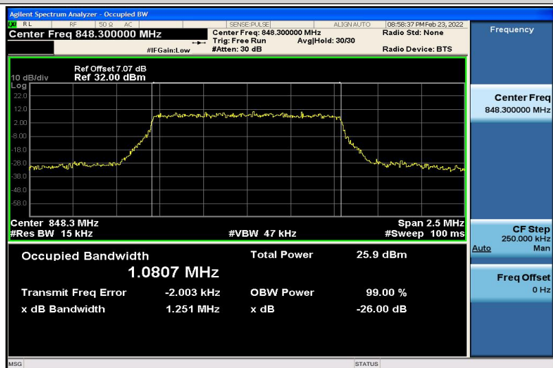
Band5-1.4MHz-16QAM-20643-6RB#0-1.0807
