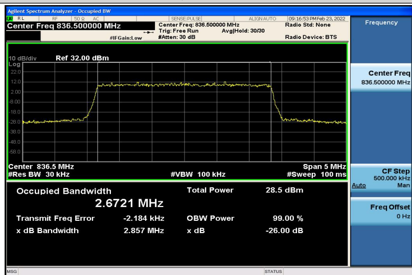
Band5-3MHz-16QAM-20525-15RB#0-2.6721
