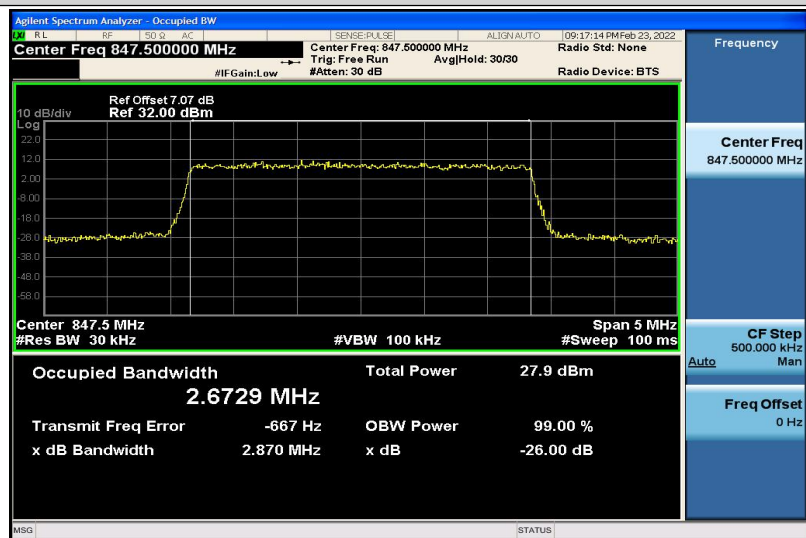
Band5-3MHz-16QAM-20635-15RB#0-2.6729
