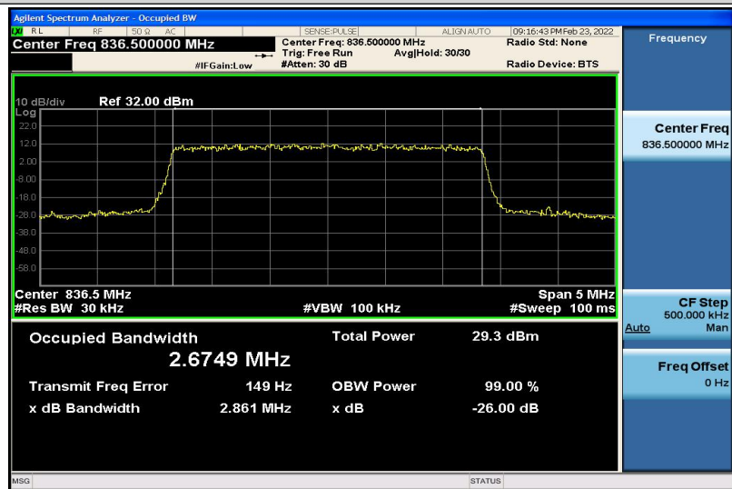
Band5-3MHz-QPSK-20525-15RB#0-2.6749
