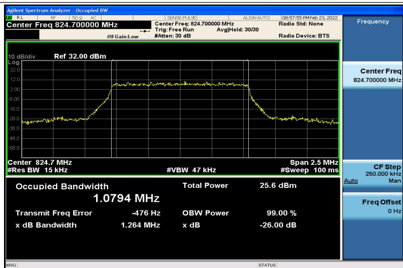
Band5-1.4MHz-16QAM-20407-6RB#0-1.0794
