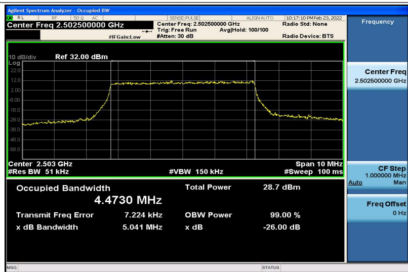
Band7-5MHz-QPSK-20775-25RB#0-4.4730
