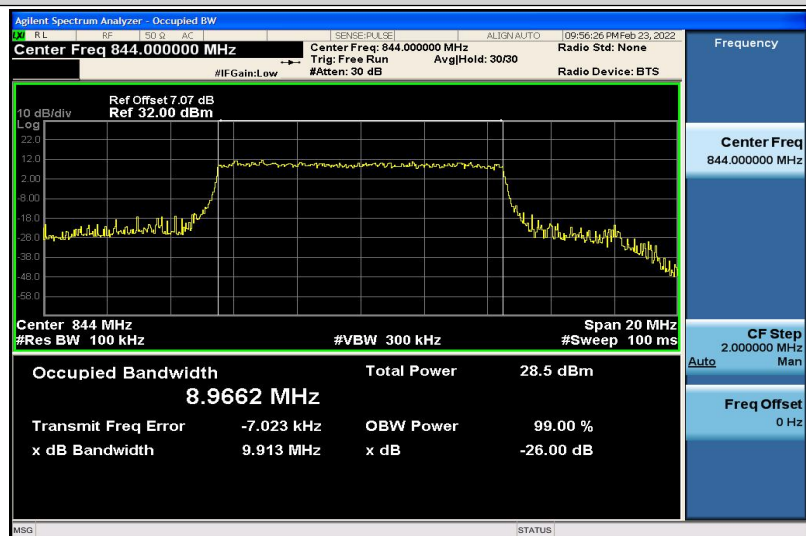
Band5-10MHz-16QAM-20600-50RB#0-8.9662
