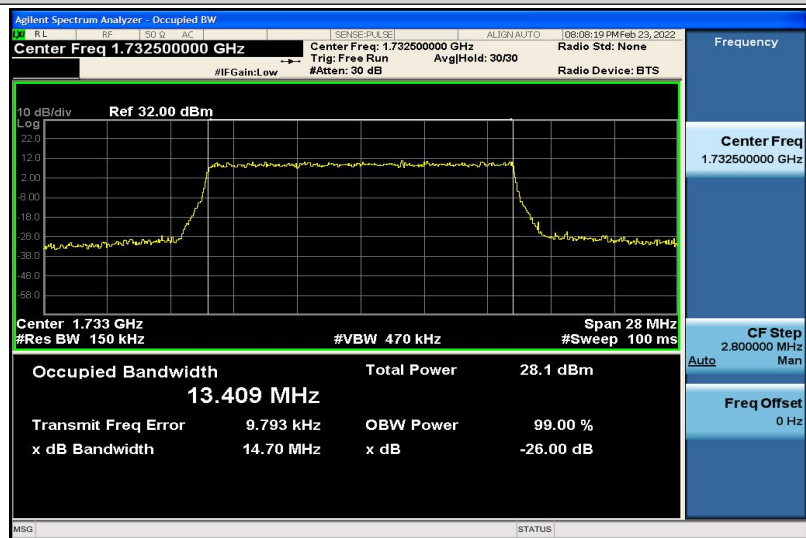
Band4-15MHz-16QAM-20175-75RB#0-13.409
