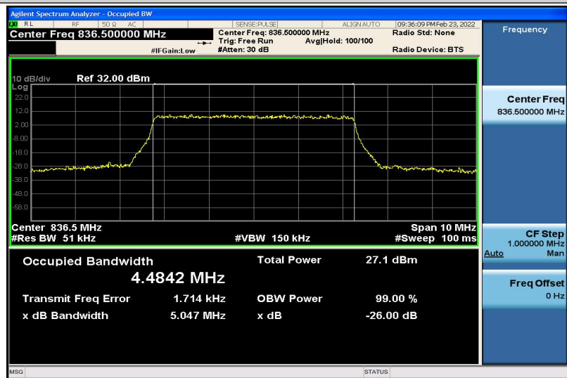
Band5-5MHz-16QAM-20525-25RB#0-4.4842
