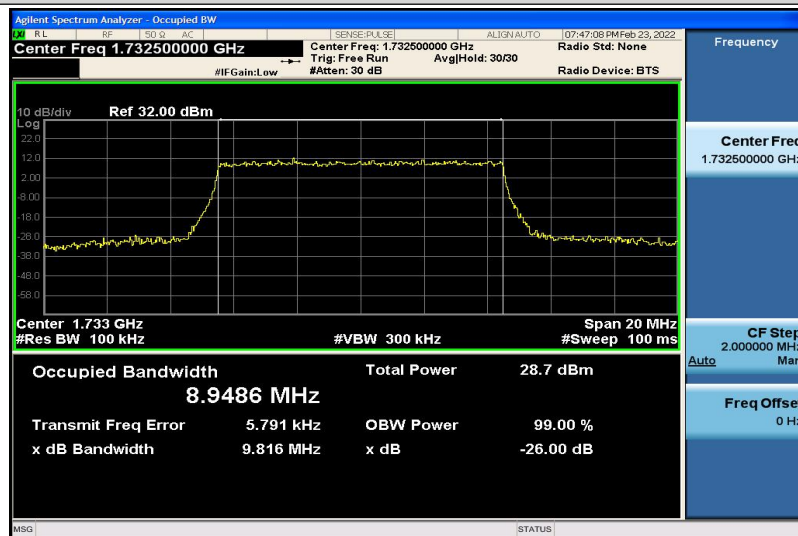
Band4-10MHz-QPSK-20175-50RB#0-8.9486
