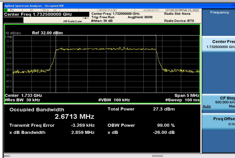
Band4-3MHz-16QAM-20175-15RB#0-2.6713
