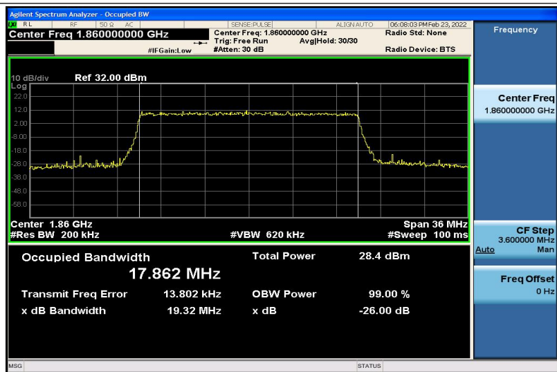
Band2-20MHz-16QAM-18700-100RB#0-17.862
