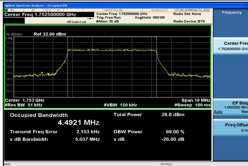
Band4-5MHz-QPSK-20375-25RB#0-4.4921
