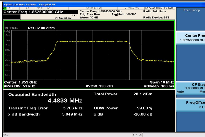
Band2-5MHz-16QAM-18625-25RB#0-4.4833
