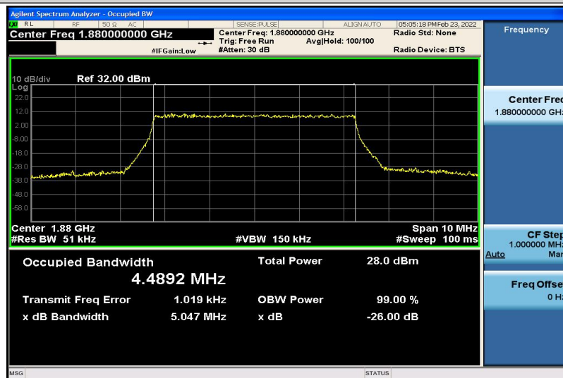
Band2-5MHz-16QAM-18900-25RB#0-4.4892
