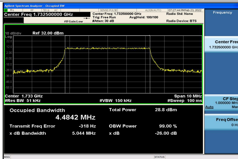
Band4-5MHz-QPSK-20175-25RB#0-4.4842
