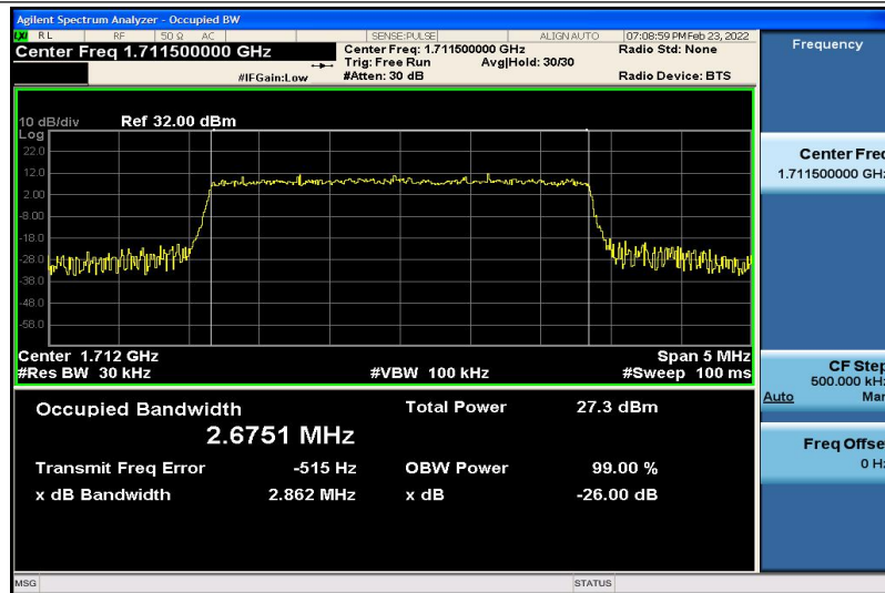
Band4-3MHz-16QAM-19965-15RB#0-2.6751
