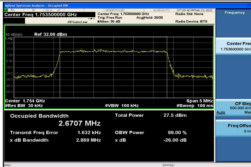
Band4-3MHz-16QAM-20385-15RB#0-2.6707
