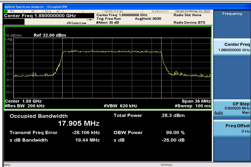
Band2-20MHz-16QAM-18900-100RB#0-17.905
