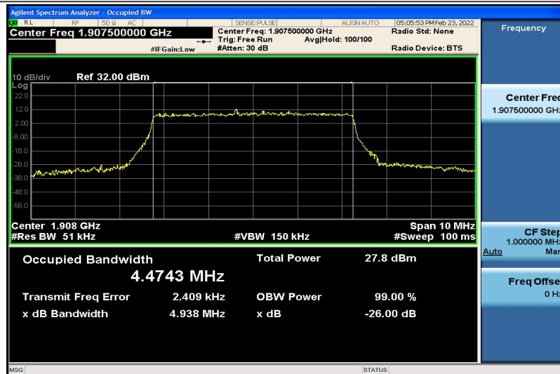
Band2-5MHz-16QAM-19175-25RB#0-4.4743
