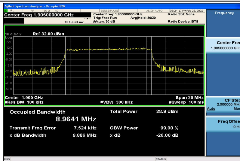
Band2-10MHz-QPSK-19150-50RB#0-8.9641
