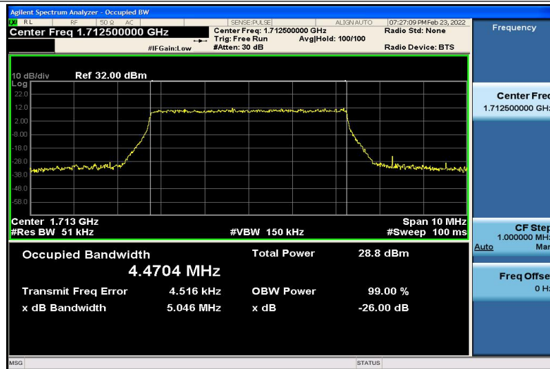
Band4-5MHz-QPSK-19975-25RB#0-4.4704
