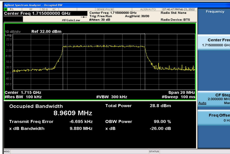
Band4-10MHz-QPSK-20000-50RB#0-8.9609
