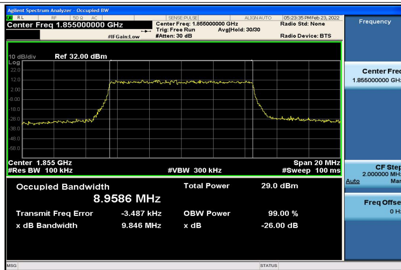
Band2-10MHz-QPSK-18650-50RB#0-8.9586
