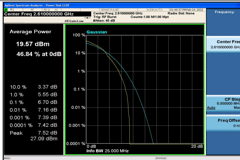
Band38-20MHz-16QAM-38150-1RB#0
