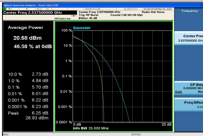
Band41-5MHz-16QAM-40065-25RB#0
