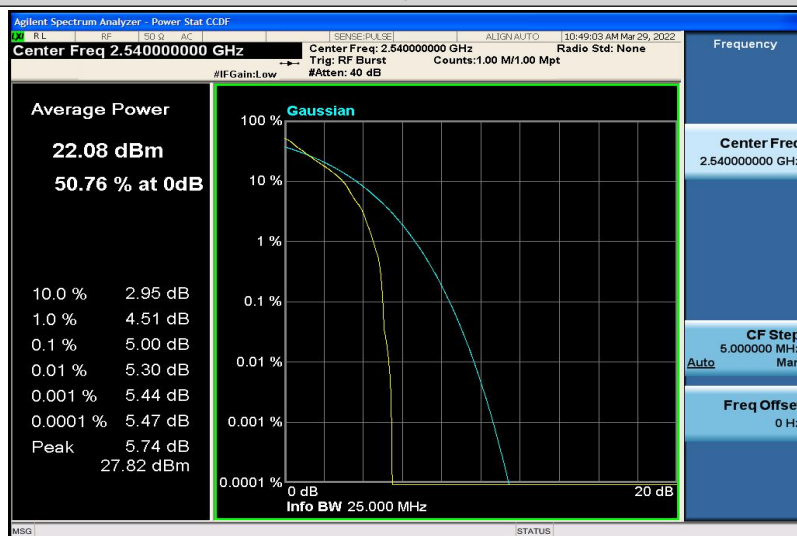
Band41-10MHz-QPSK-40090-1RB#0
