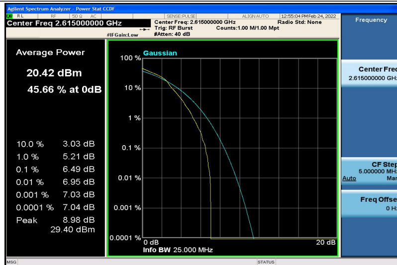
Band38-10MHz-16QAM-38200-1RB#0
