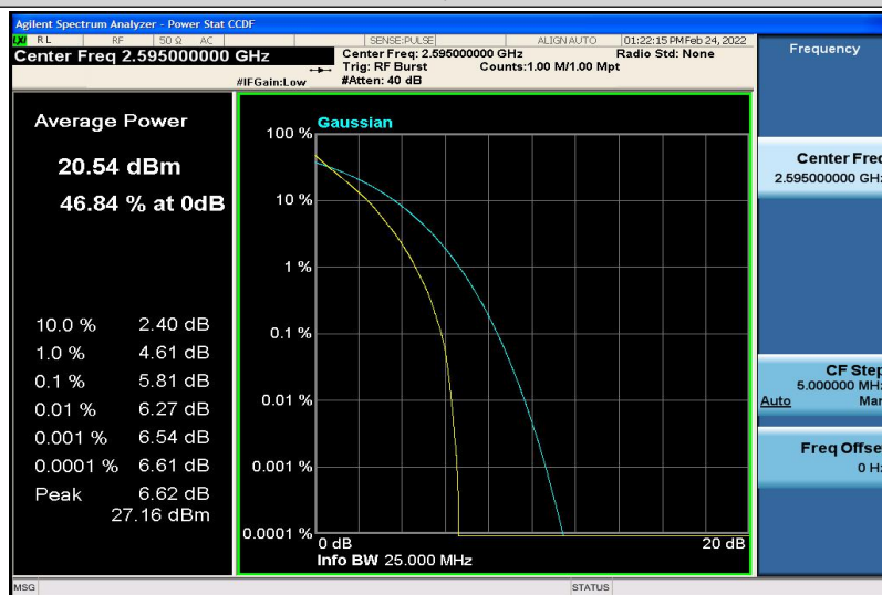
Band38-15MHz-QPSK-38000-75RB#0
