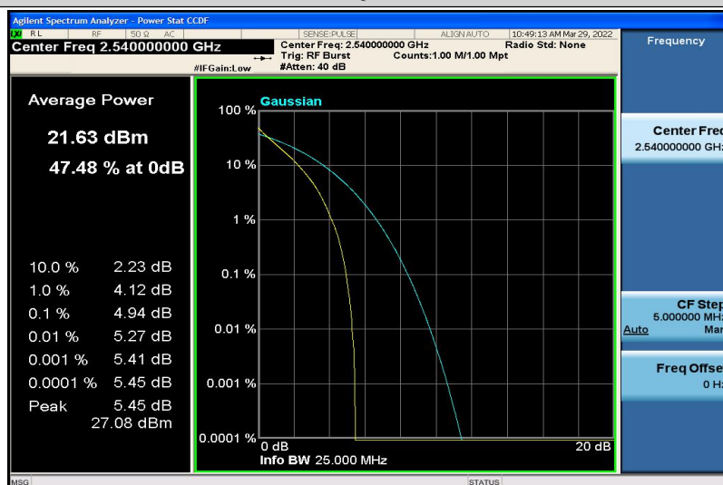
Band41-10MHz-QPSK-40090-50RB#0
