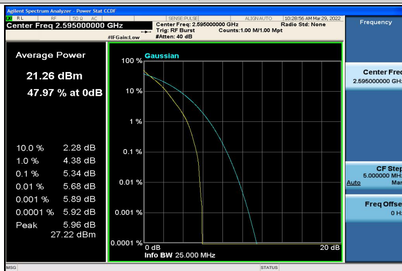
Band41-5MHz-QPSK-40640-25RB#0
