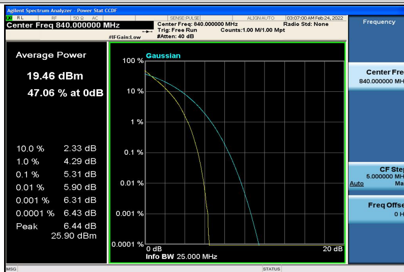
Band19-10MHz-QPSK-24100-50RB#0
