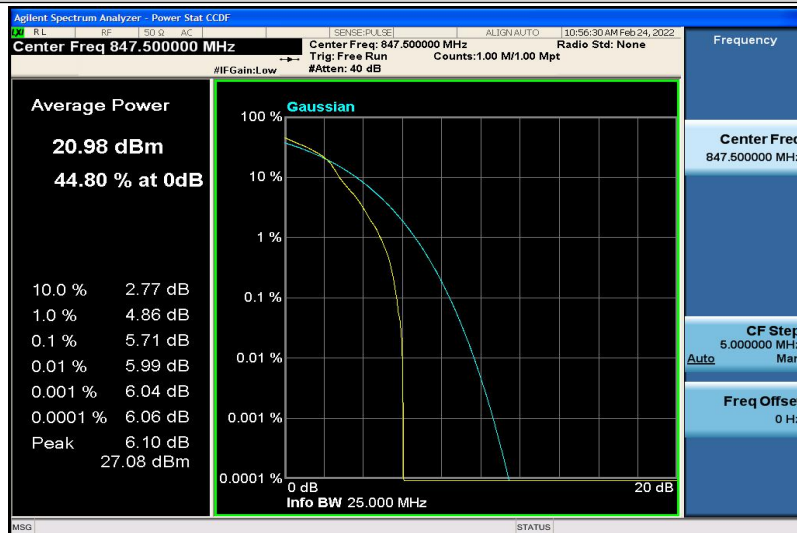
Band26-3MHz-16QAM-27025-1RB#0
