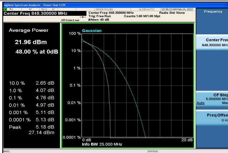
Band26-1.4MHz-QPSK-27033-1RB#0
