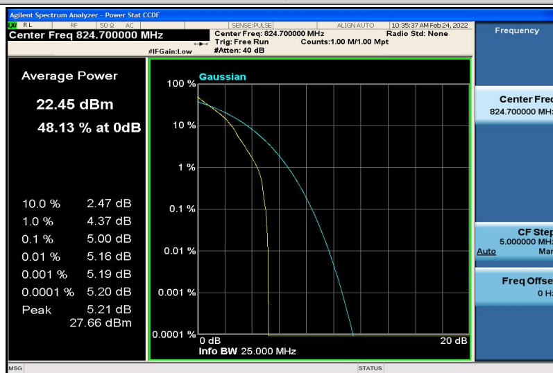
Band26-1.4MHz-QPSK-26797-1RB#0
