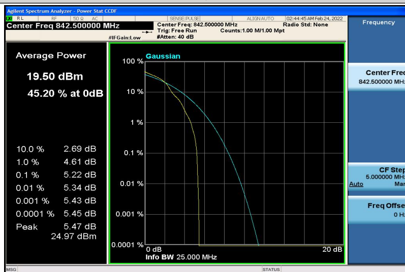
Band19-5MHz-16QAM-24125-1RB#0
