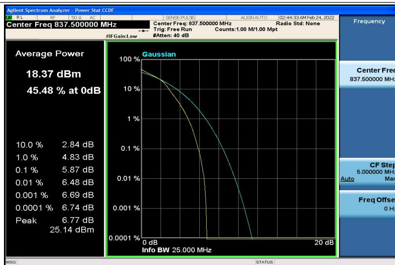
Band19-5MHz-16QAM-24075-25RB#0
