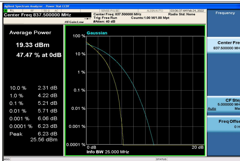
Band19-10MHz-QPSK-24075-50RB#0
