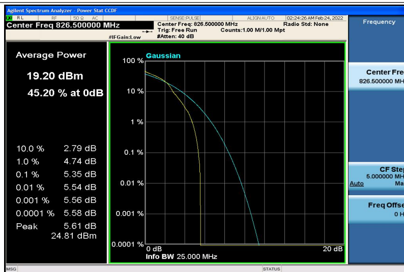
Band18-5MHz-16QAM-23965-1RB#0
