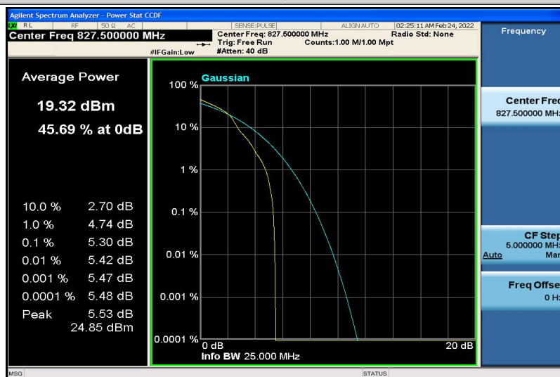
Band18-5MHz-16QAM-23975-1RB#0
