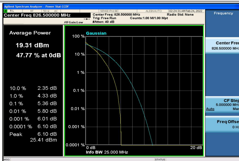
Band18-5MHz-QPSK-23965-25RB#0
