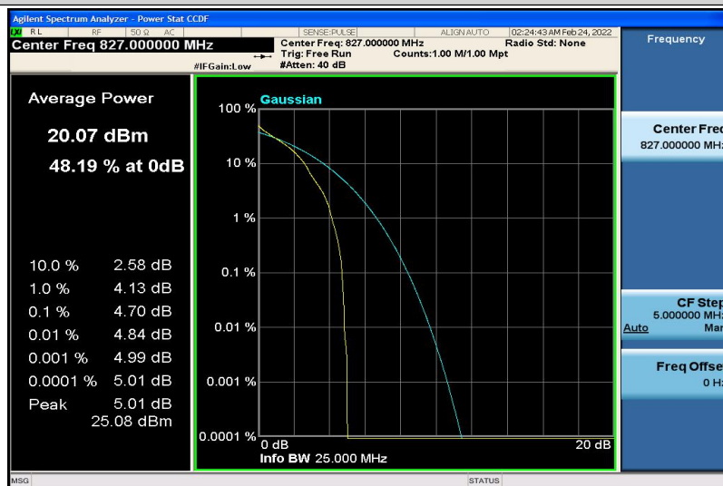
Band18-5MHz-QPSK-23970-1RB#0
