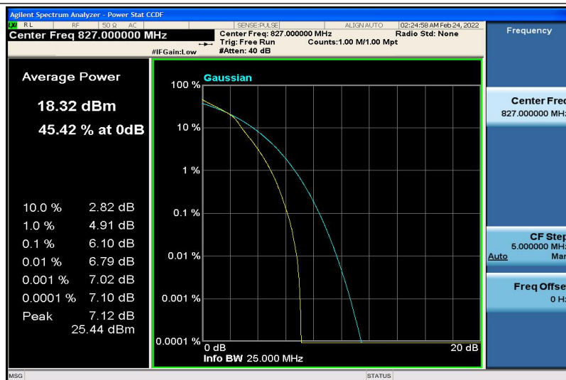
Band18-5MHz-16QAM-23970-25RB#0
