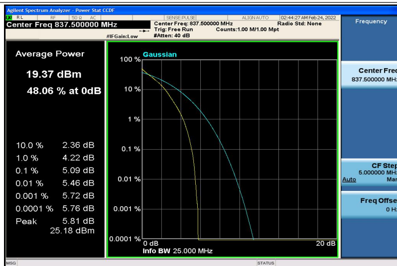
Band19-5MHz-QPSK-24075-25RB#0
