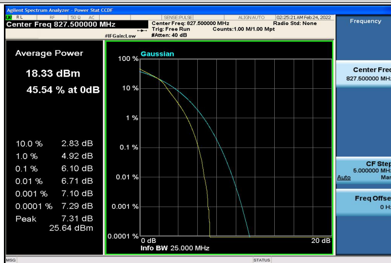
Band18-5MHz-16QAM-23975-25RB#0
