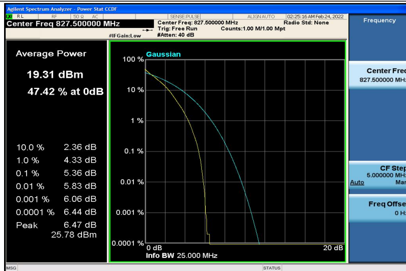
Band18-5MHz-QPSK-23975-25RB#0
