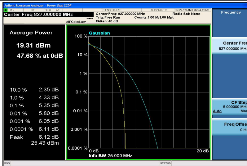
Band18-5MHz-QPSK-23970-25RB#0
