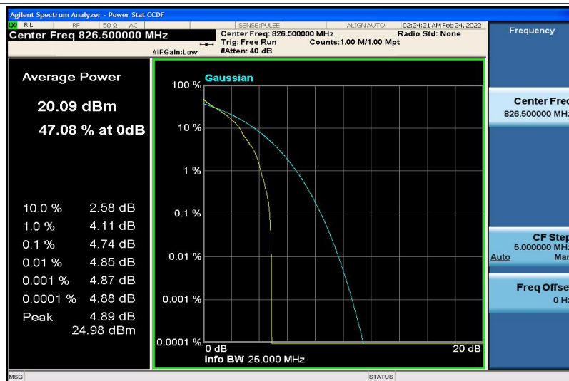
Band18-5MHz-QPSK-23965-1RB#0
