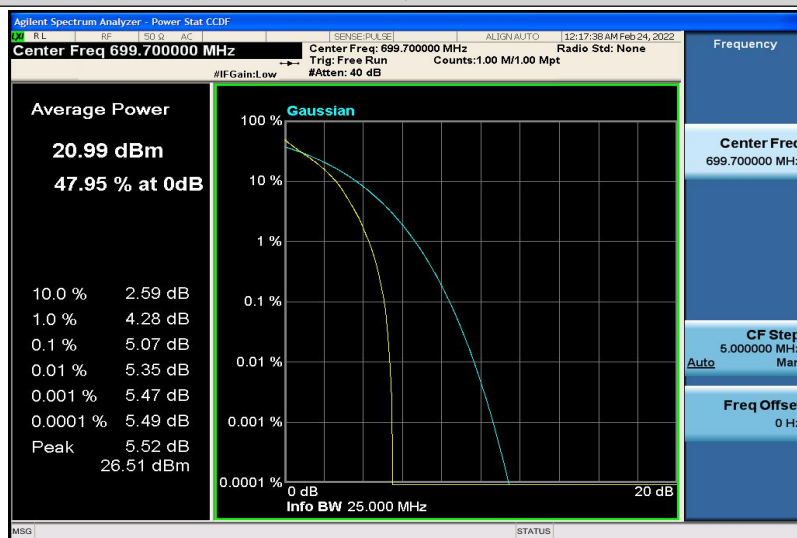
Band12-1.4MHz-QPSK-23017-6RB#0
