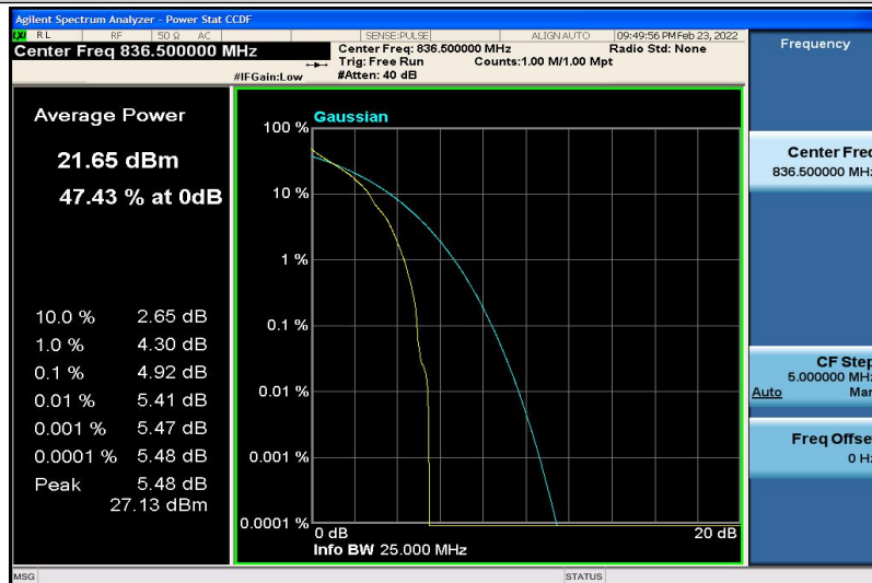
Band5-5MHz-QPSK-20525-1RB#0
