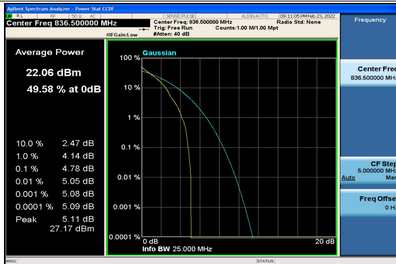
Band5-1.4MHz-QPSK-20525-1RB#0
