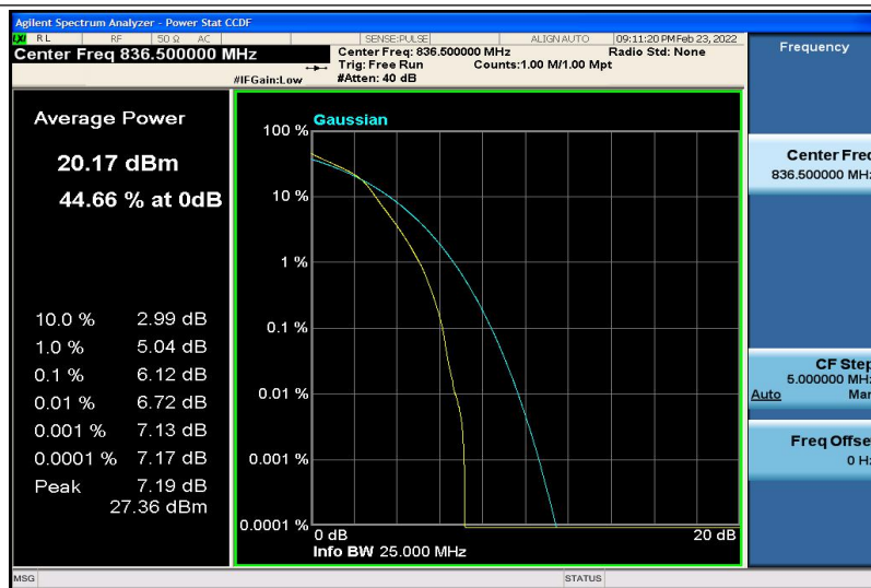
Band5-1.4MHz-16QAM-20525-6RB#0
