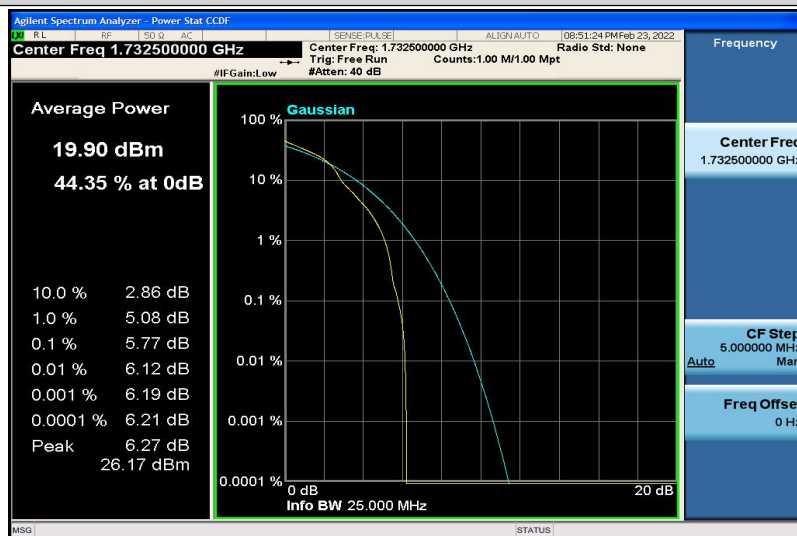
Band4-20MHz-16QAM-20175-1RB#0
