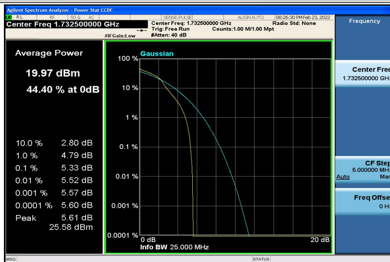
Band4-15MHz-16QAM-20175-1RB#0
