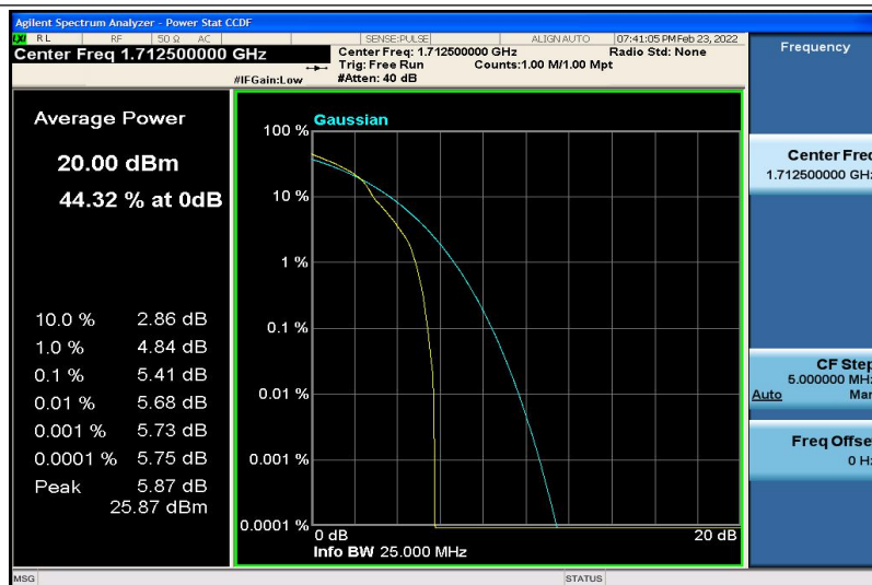
Band4-5MHz-16QAM-19975-1RB#0
