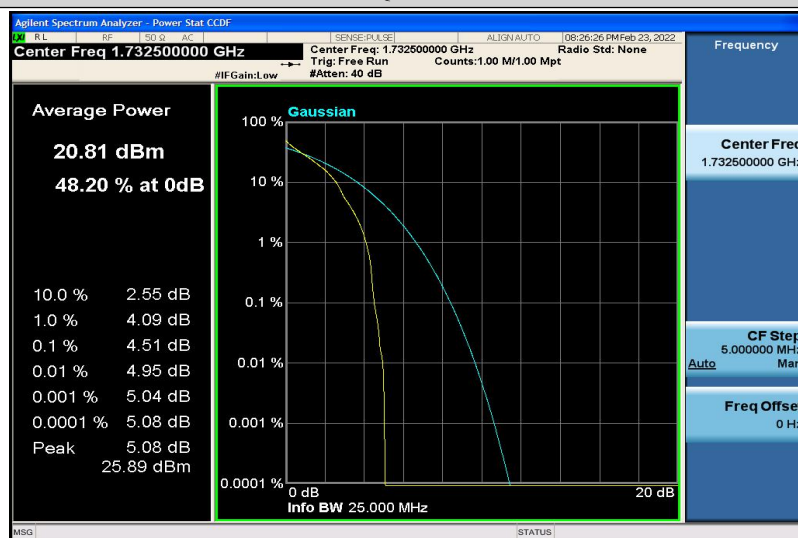
Band4-15MHz-QPSK-20175-1RB#0
