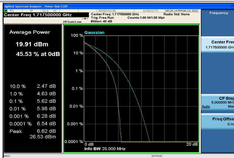
Band4-15MHz-QPSK-20025-75RB#0
