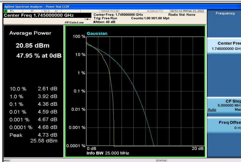
Band4-20MHz-QPSK-20300-1RB#0
