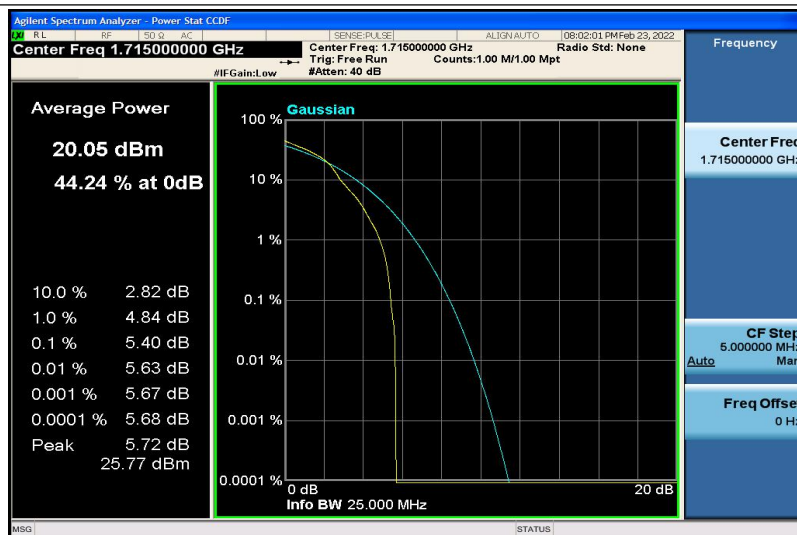
Band4-10MHz-16QAM-20000-1RB#0
