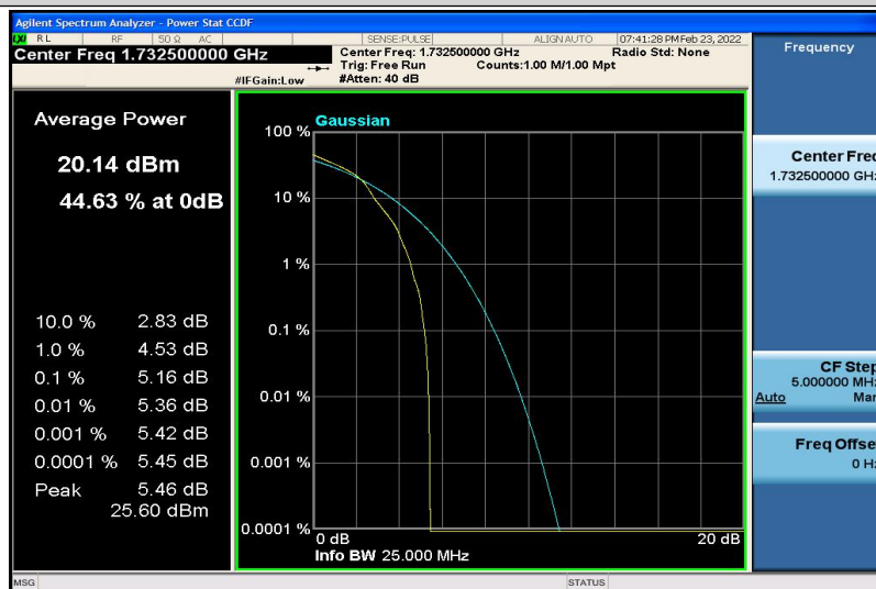
Band4-5MHz-16QAM-20175-1RB#0
