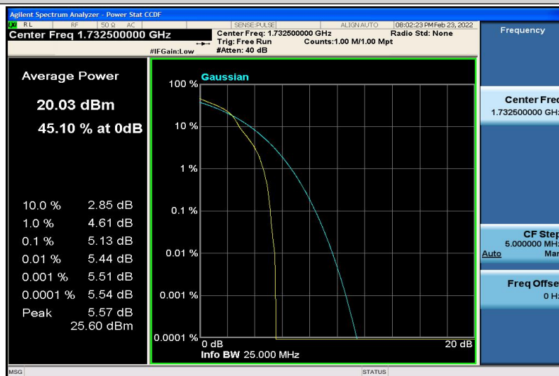
Band4-10MHz-16QAM-20175-1RB#0
