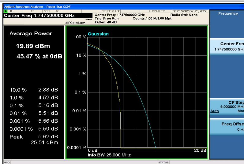
Band4-15MHz-16QAM-20325-1RB#0
