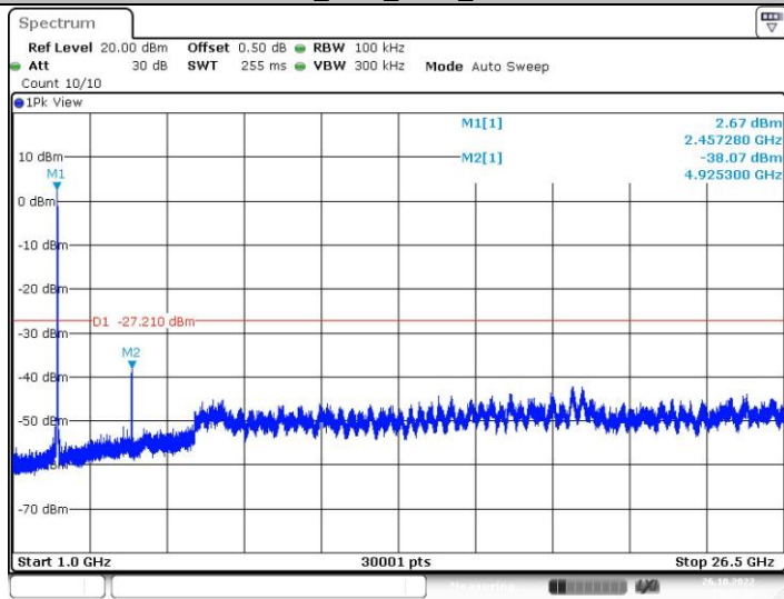
11N20SISO_Ant1_2462_1000~26500
