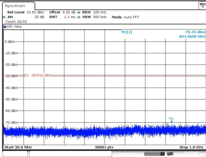
11N40SISO_Ant1_2437_30~1000
